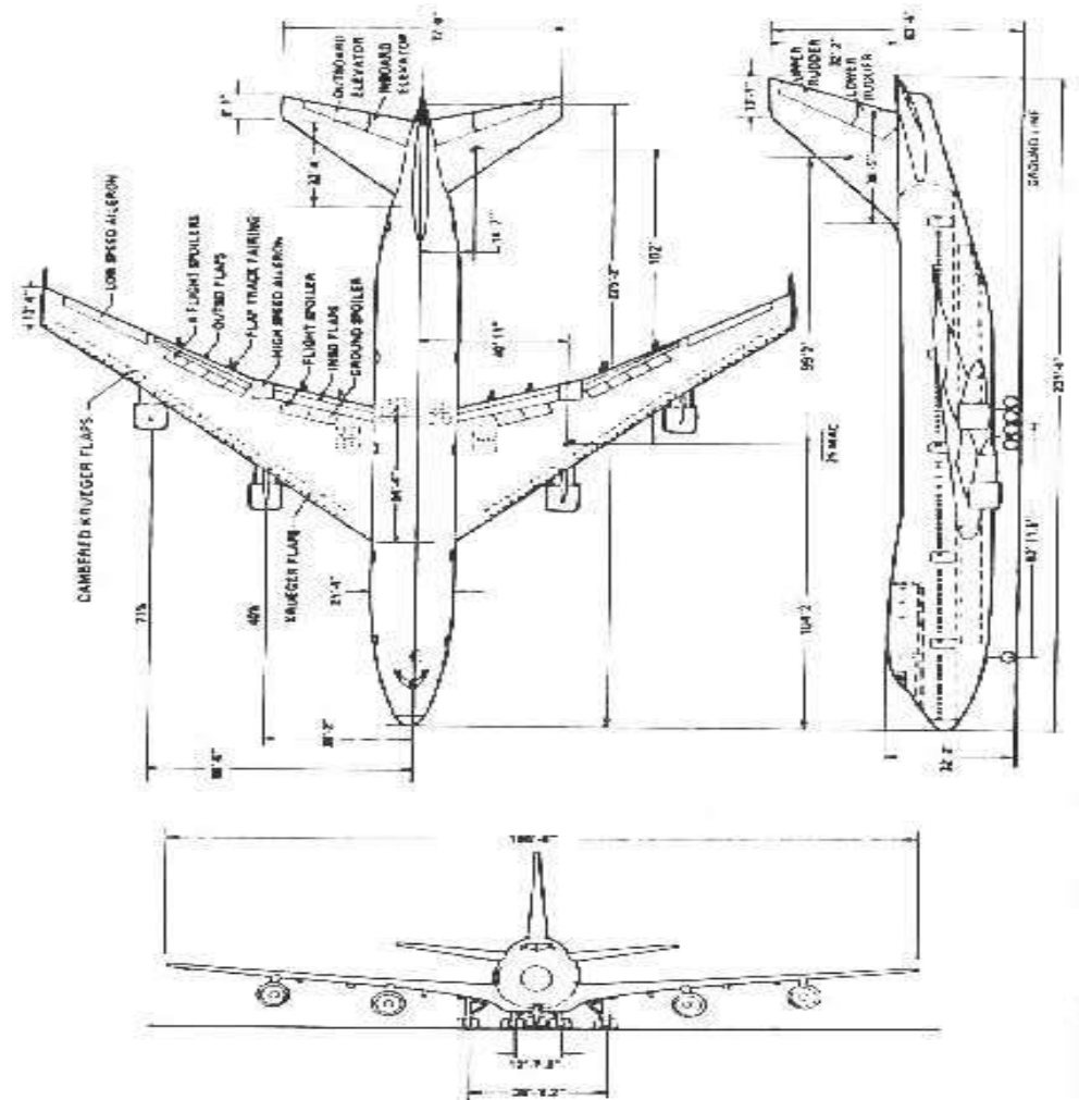
Figure 4-4 Boeing 747
