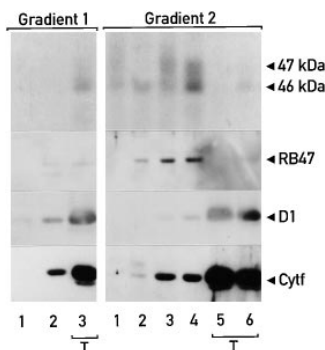
Figure 5. Immunoblot and UV cross-linking analyses of fractions from gradients 1 and 2. The 46-, 47-, and 60-kD RNA-binding proteins, which were found to bind to the ^{32}P -RNA probe in the UV cross-linking assay, cofractionate with thylakoids ( T ) in the presence of magnesium ions ( Gradient 1 ). In the absence of magnesium ions ( Gradient 2 ), these proteins and the low density
