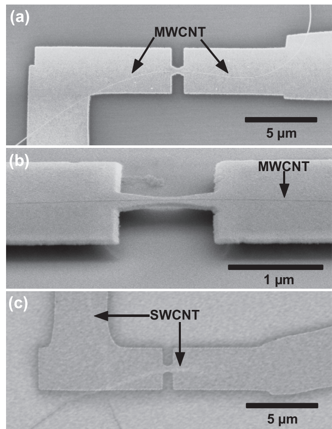
FIG. 1. SEM images of a MWCNT and a SWCNT breakjunction devices before electromigration. (a) A gold breakjunction directly on top of a MWCNT. The width of the junction is about 300 nm. (b) Tilted SEM image of the device in (a) after suspension. The MWCNT is clearly visible under the gold film. (c) A breakjunction aligned on top of a SWCNT (device A). The image is obtained from the superposition of two SEM images, before and after the breakjunction is exposed, as a SWCNT is not visible under the gold film.
