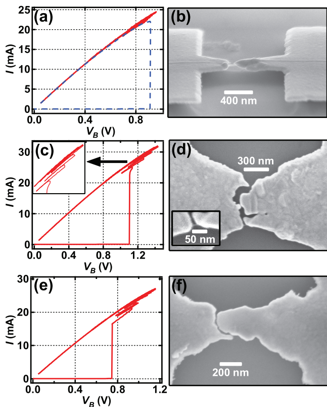
FIG. 2. (Color online) Nanoetching technique. (a) I-V_B characteristics during the electromigration of the device shown in Fig. 1(b). V_B is ramped up until the feedback detects an increase in the resistance and rapidly lowers the bias. This procedure is repeated to gradually narrow the gold bridge (full red curve). The process can be stopped at any position in the I-V_B , and then the partially etched junction can be broken with a continuous voltage ramp (dashed blue curve). (b) Tilted SEM image of the 70 nm-long MWCNT device electromigrated in (a). (c) Nanoetching I-V_B curve for SWCNT-device A (Fig. 1(c)). The inset is a zoom on the gradual etching of the device. (d) Top view SEM image of device A after breaking. The inset shows a zoom-in on the 22 \pm 5 nm-long SWCNT. The location of the tube corresponds to its position after e-beam lithography. (e) Electromigration curve for SWCNT-device B. (f) SEM of device B after breaking, showing a gap \lesssim 10 nm.
