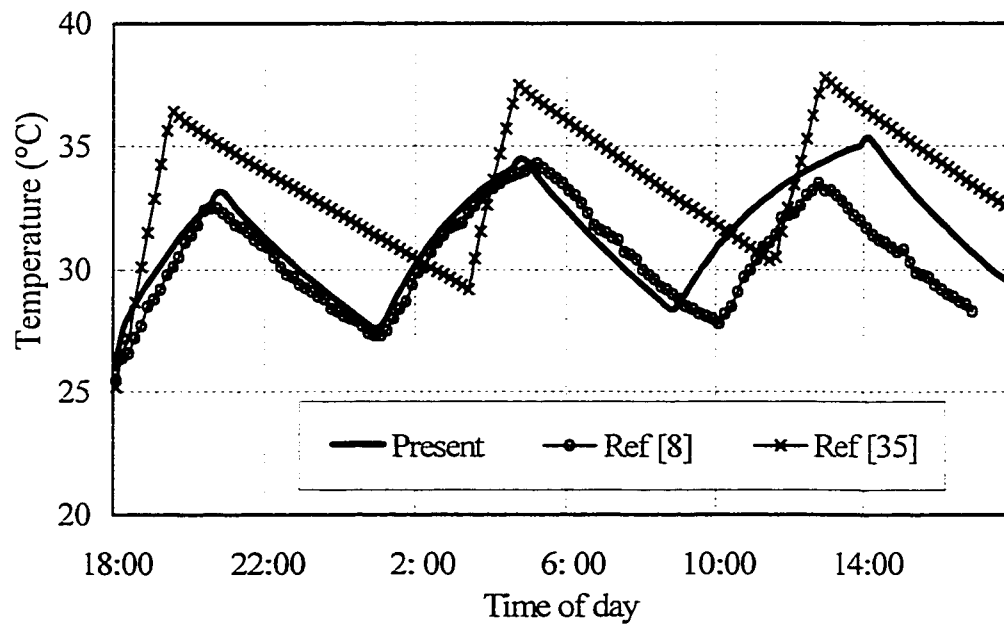
Figure 2.6.2 Comparison of predicted slab temperatures with published data
