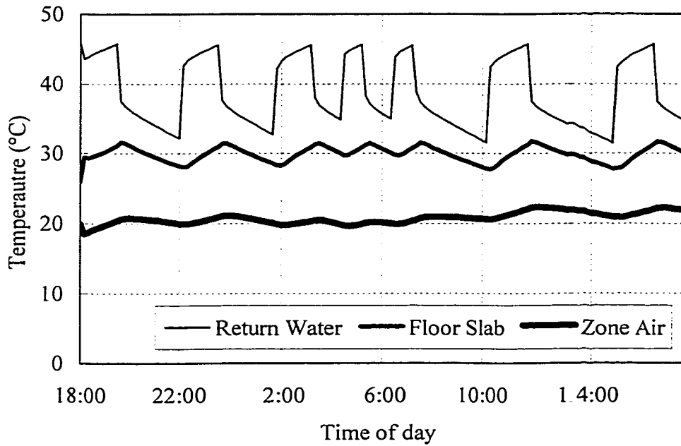
Figure 4.3.8 TPC with solar and internal heat gains
