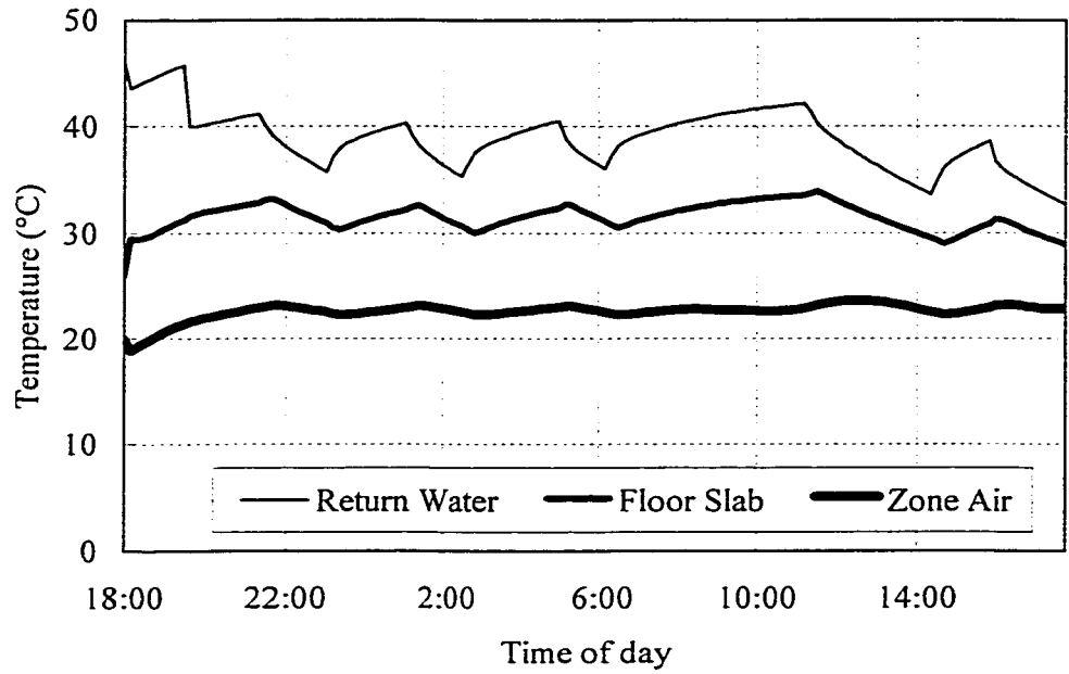
Figure 4.3.9 TSC-MM with solar and internal heat gain
