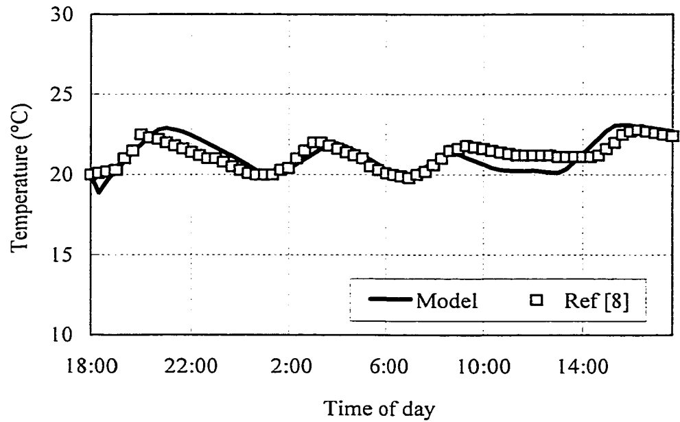
Figure 3.7.6 Zone air temperature responses on Feb. 27 with 30 minutes switching interval
