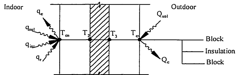
Figure 2.4.1 Typical wall section and heat fluxes
