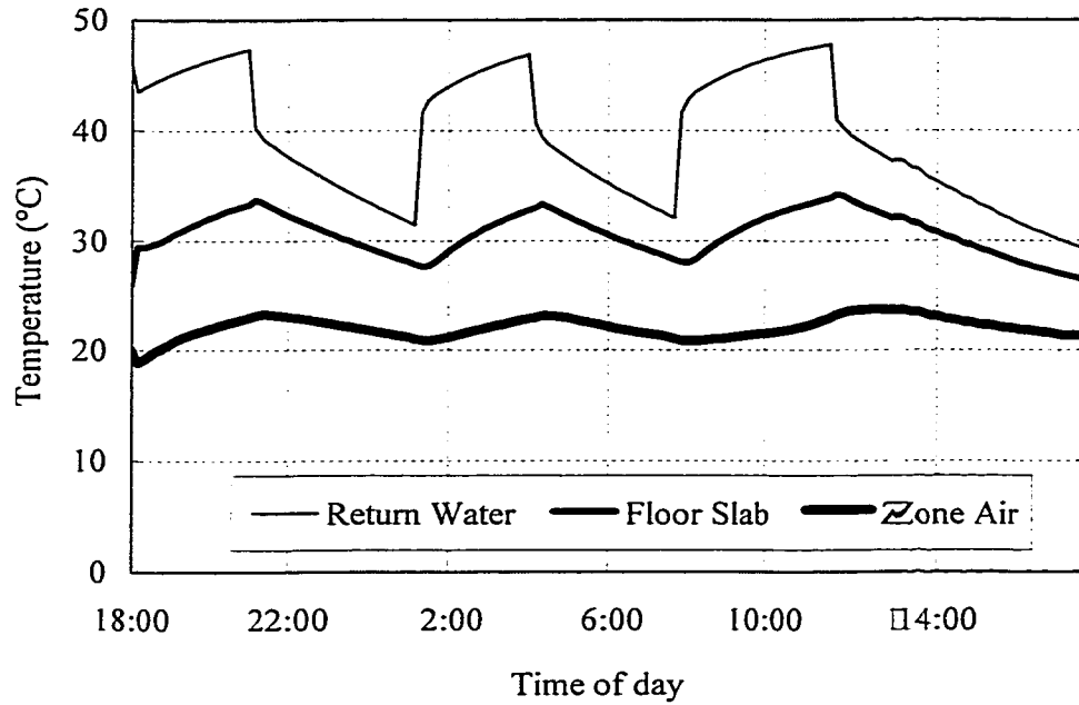
Figure 4.3.7 SPC with solar and internal heat gains
