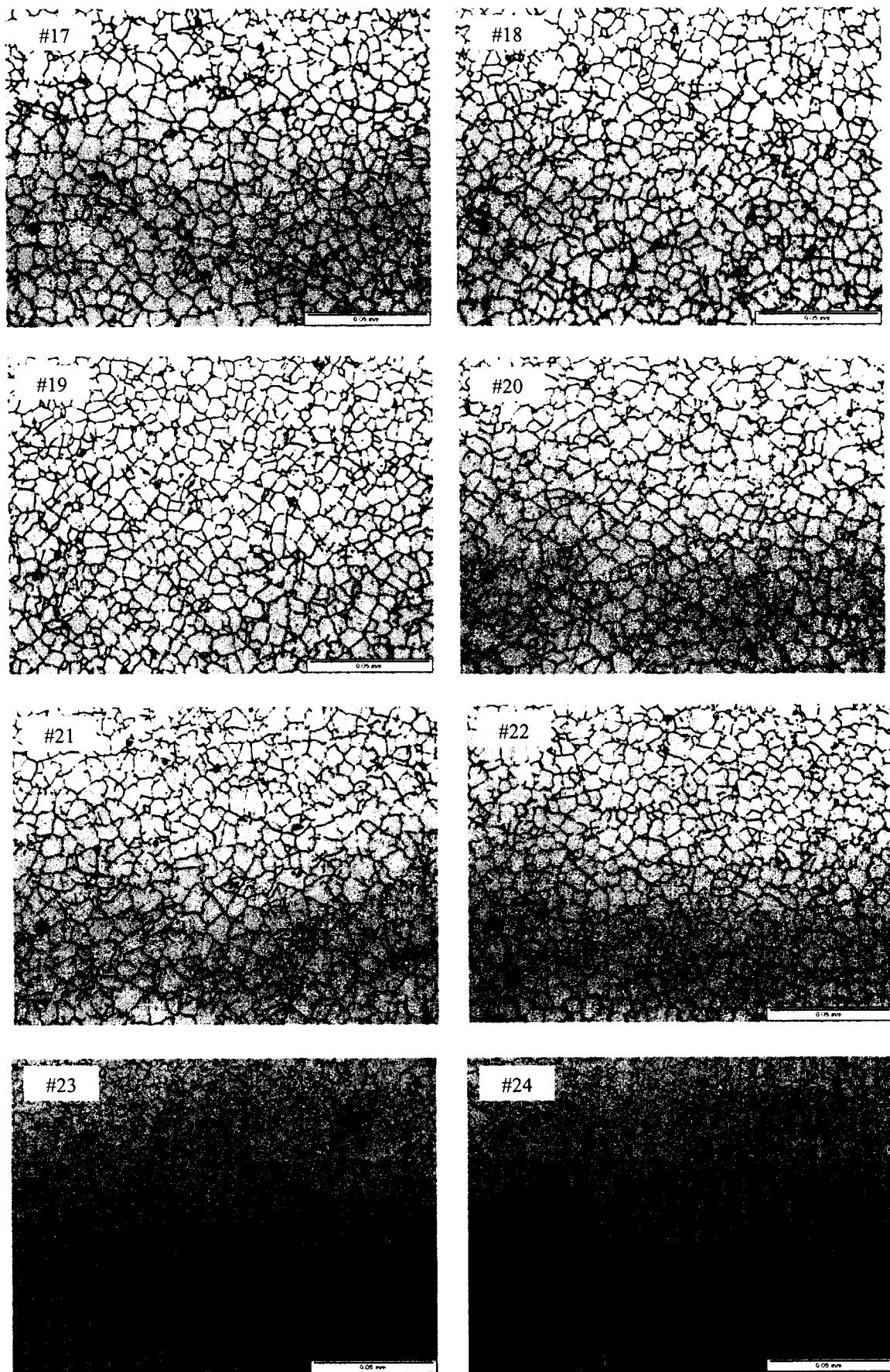
Figure 4.4.5 – FZ Microstructure for the Repeated Samples
