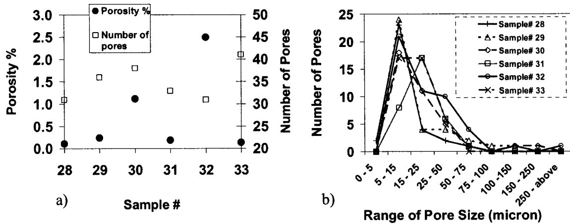
Figure 4.5.10 – Porosity Formation during Laser Welding of 6 mm Plates a) Porosity Area Percentage b) Pores Distribution
