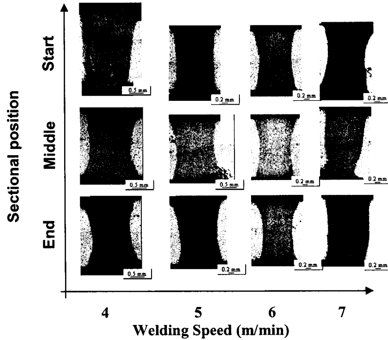
Figure 4.1.1 – Effect of Welding Speed on Weld Geometry.
