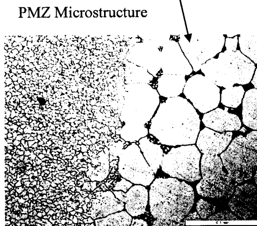
PMZ Microstructure
