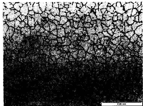
FZ Microstructure - B
