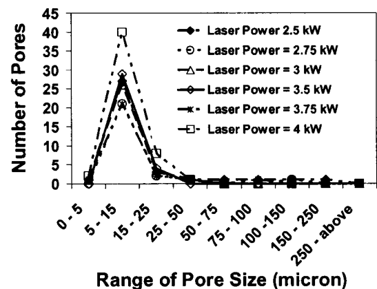
Figure 4.3.6 – Porosity Distribution
