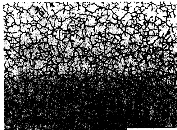
FZ Microstructure - C
