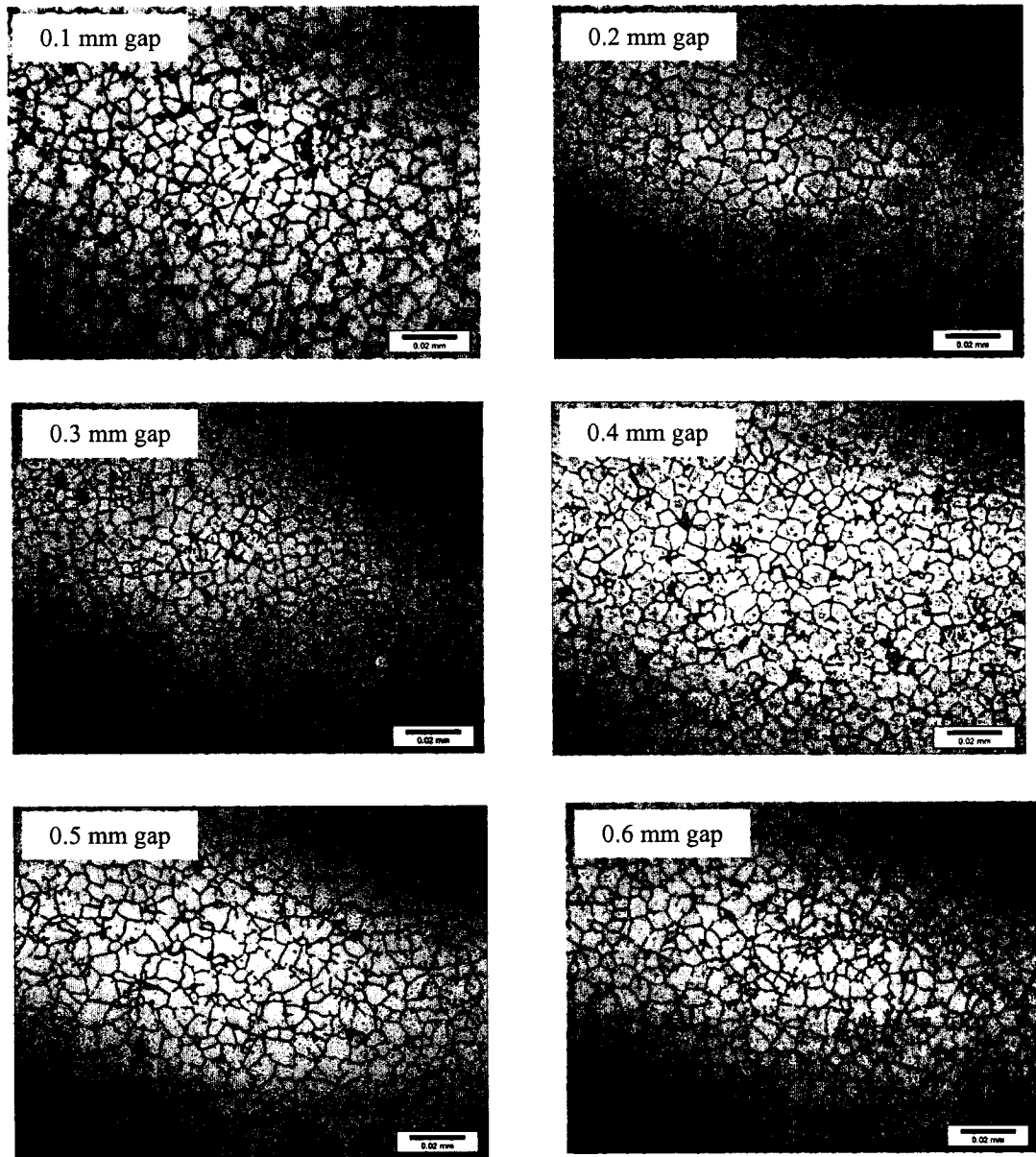
Figure 4.2.4 – Effect of gap size on the FZ microstructure
