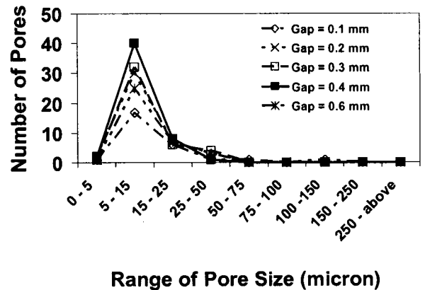
Figure 4.2.6 – Porosity distribution.
