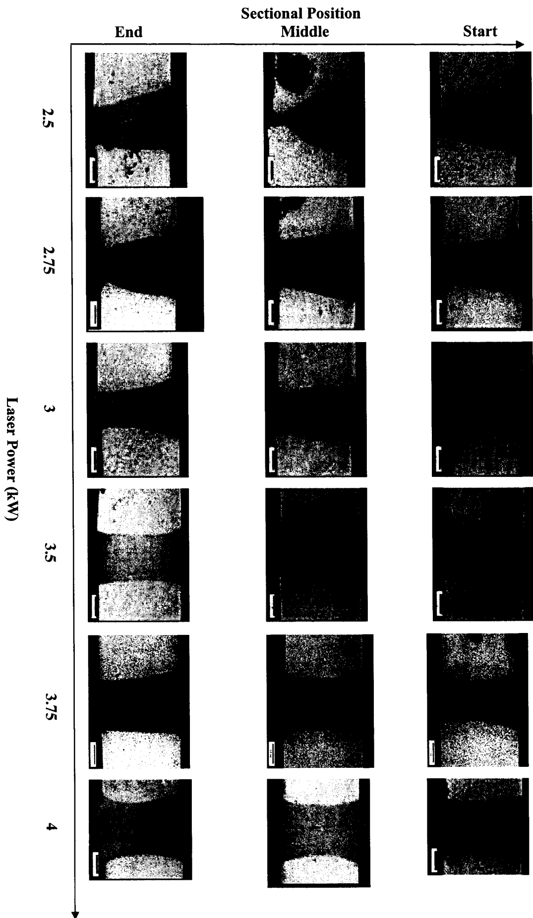
Figure 4.3.2 – Effect of Laser Power on Weld Geometry
