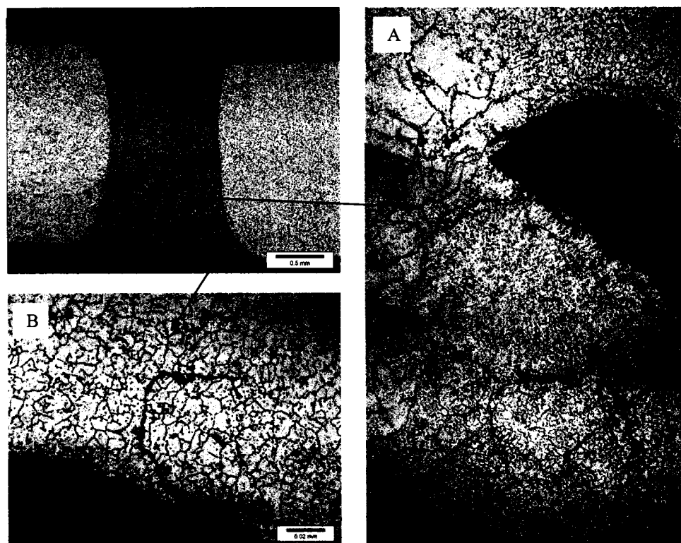
Figure 4.2.10 – Solidification Cracks in The Sample Welded at 0.2 mm gap – Middle Section
