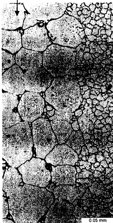
PMZ Microstructure
