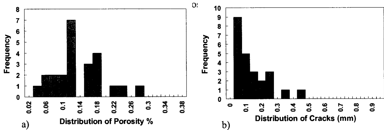
Figure 4.4.7 – Defects Distribution for the Repeated Laser Welded Samples a) Porosity Area Percentage b) Solidification Cracks Length
