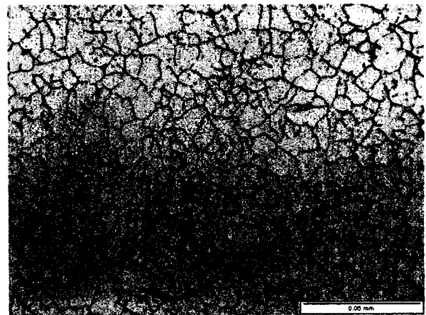
FZ Microstructure - A
