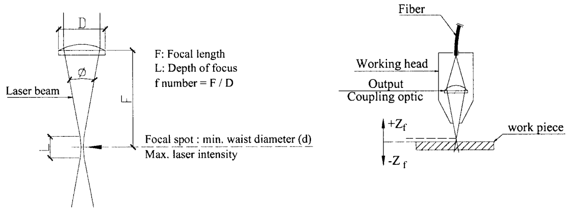
Figure 2.4 : Focusing parameters [19,20].
