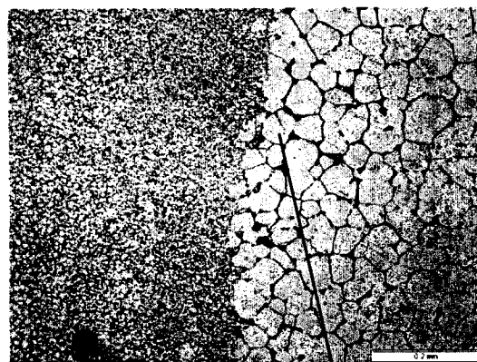
PMZ Microstructure
