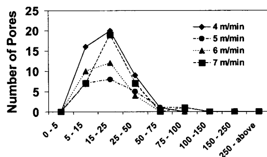
Figure 4.1.6 – Porosity Distribution
