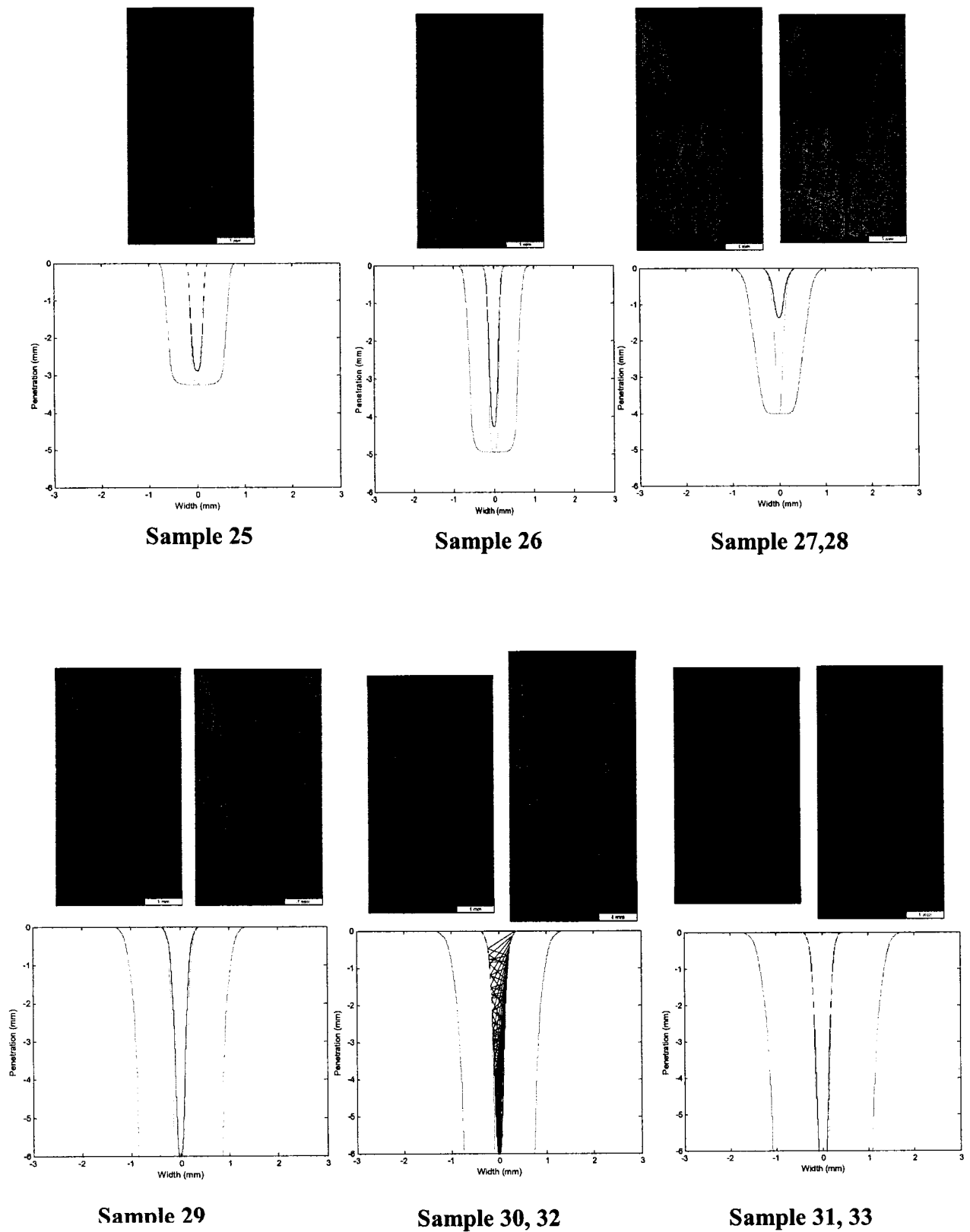
Figure 4.7.10 –Comparison between Experimental and Calculated Weld Geometry for the 6 mm Laser Welded Plates
