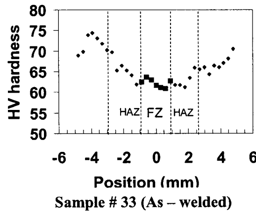
Figure 4.5.19 – Microhardness Profiles for the Full Penetrated 6 mm Laser Welded Plates in a) as – Welded Condition b) Heat Treated
