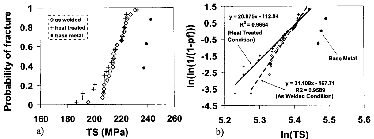
Figure 4.4.14 – Weibull Statistical Analysis for Tensile Strength a) Cumulative Plots of Tensile Strength b) Weibull Plots of Tensile Strength
