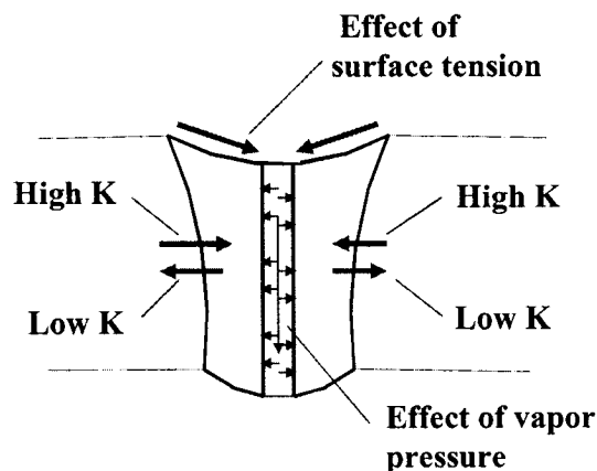
Figure 2.5: Schematic diagram for the effect of physical properties on weld geometry
