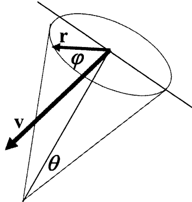
Figure 4.6.2 – Polar coordinate for the Keyhole and the Moving Line Source
