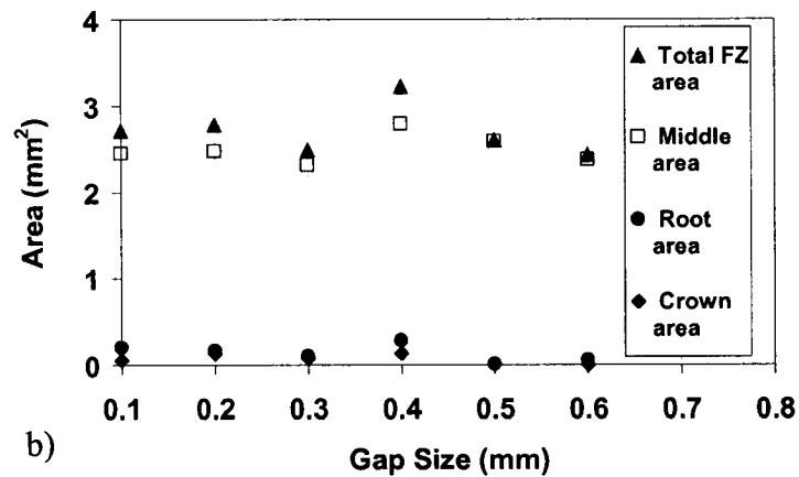
Figure 4.2.2 – Effect of Gap Size on (a) joint size and (b) weld area.
