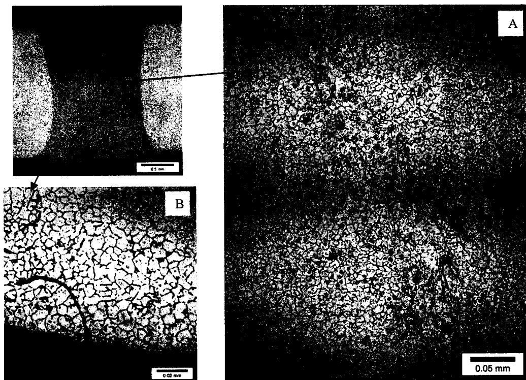
Figure 4.2.12 – Solidification Cracks in the Sample Welded at 0.4 mm gap – End Section
