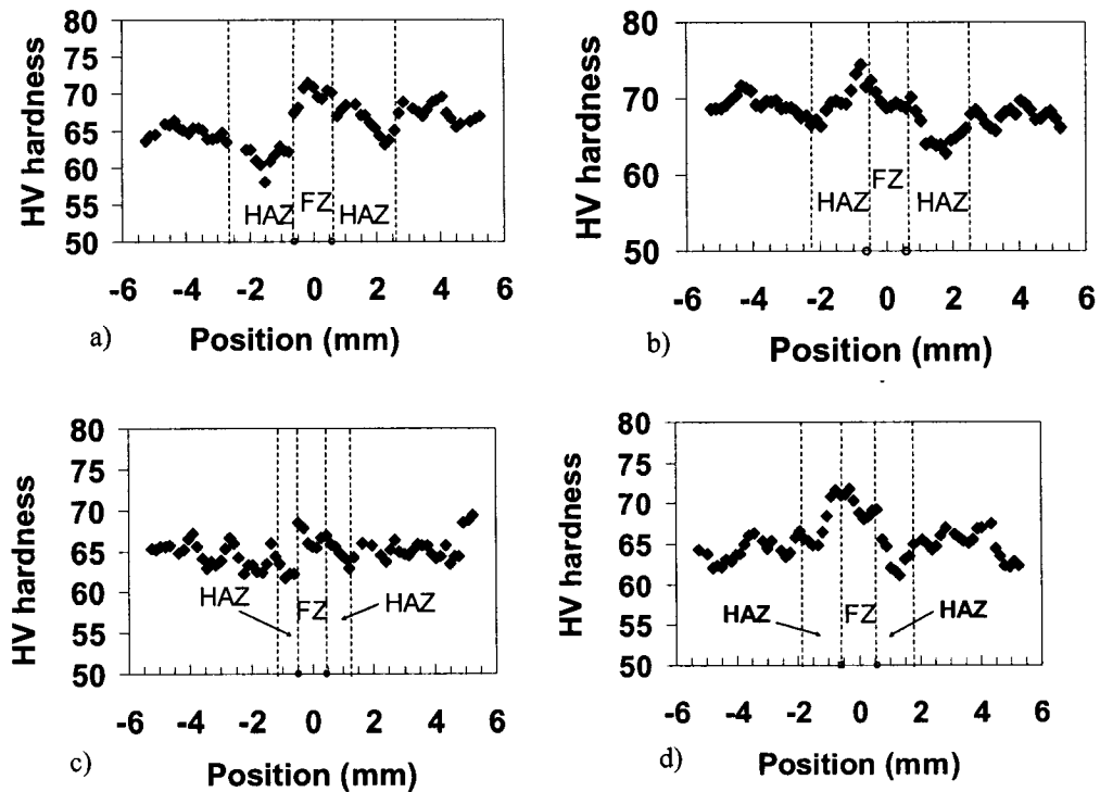
Figure 4.1.10 – Vickers Microindentation Hardness for Welding Speed at (a) 4, (b) 5, (c) 6, and (d) 7 m/min.
