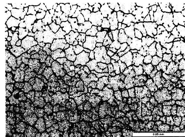
FZ Microstructure - C
