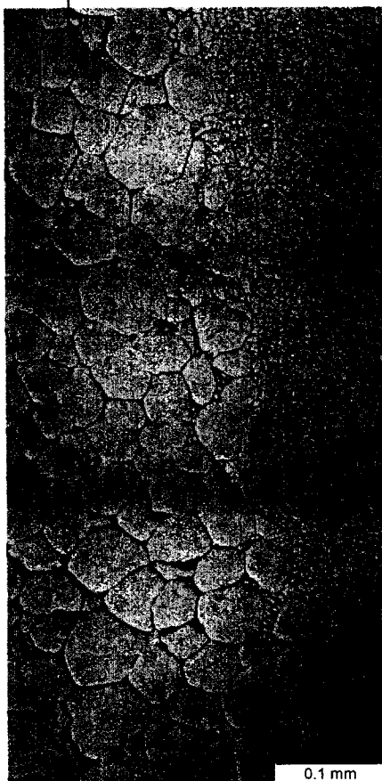
PMZ Microstructure
