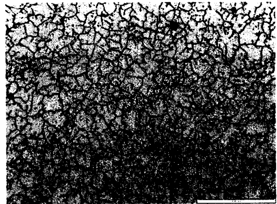
FZ Microstructure - A
