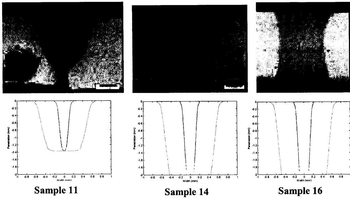
Figure 4.7.11 –Comparison between Experimental and Calculated Weld Geometry Showing the Effect of Laser Power on Laser Welding of the 2 mm Plates
