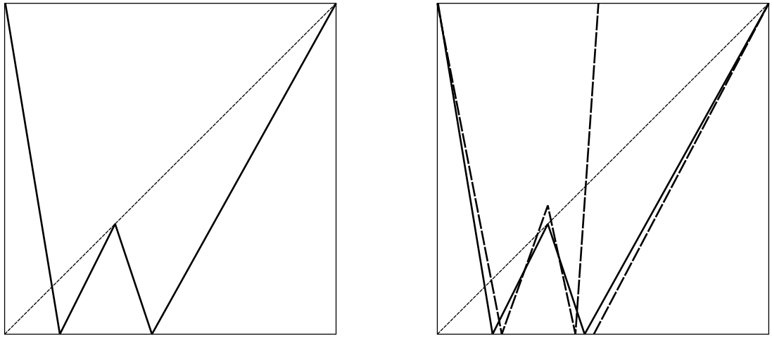
FIGURE 2. Example of W-map not in class C^{1+1} and its untypical perturbation.
