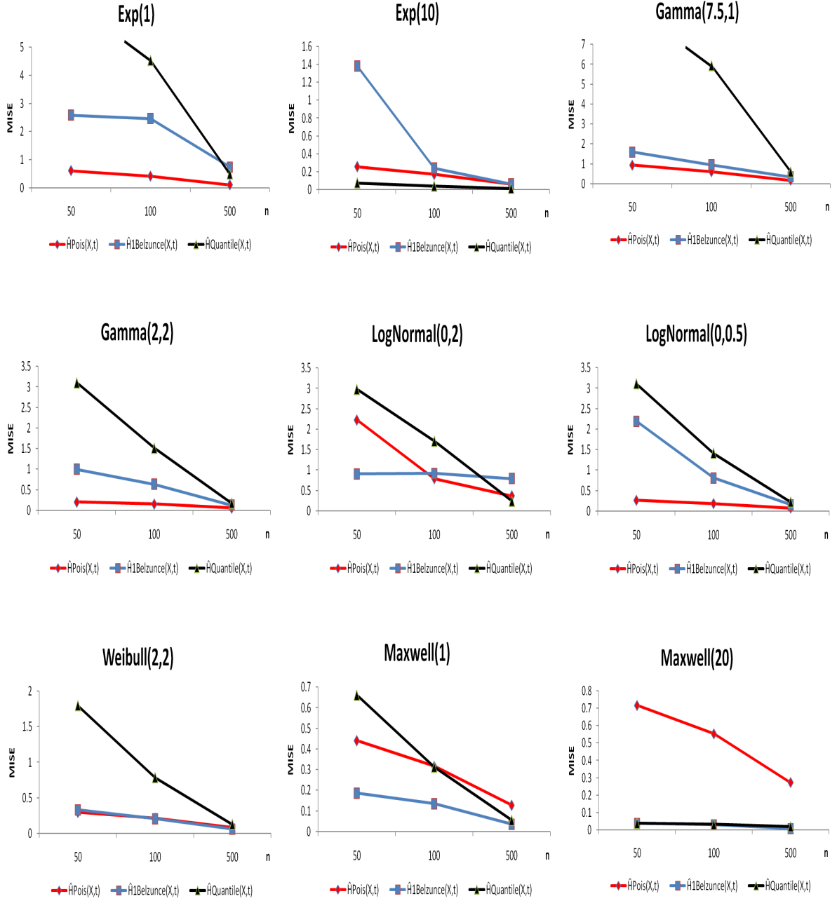
Figure 3: Residual entropy estimation MISE comparison with different sample size n = 50, 100 and 500 . Where diamond-red is \hat{H}^{Pois}(X, t) , square-blue is \hat{H}_1^{Belzunce}(X, t) , and triangle-black is \hat{H}^{Quantile}(X, t) .
