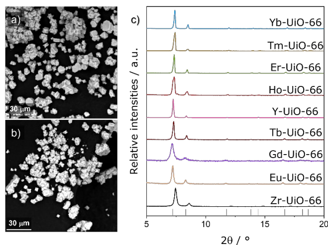
Fig. 2 : SEM image showing the polyhedral crystals for (a) Tm-UiO-66 and (b) Y-UiO-66; (c) Stacked PXRDs for all the RE-UiO-66 and Zr-UiO-66 for comparison. Vertical lines are the allowed reflections from the Tm-UiO-66 crystal structure.
