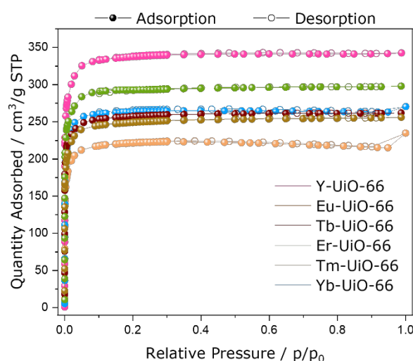
Fig. 3 Nitrogen adsorption-desorption isotherms for RE-UiO-66 (RE = Y, Eu, Tb, Er, Tm, Yb).
