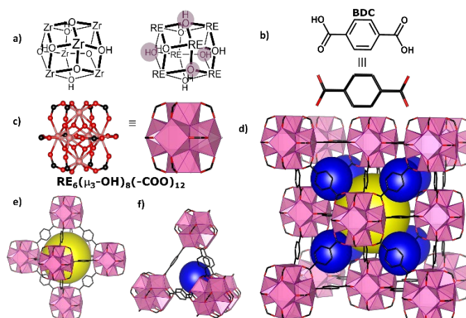
Fig. 1 Structure of RE-UiO-66. (a) Differences between Zr- and RE-hexanuclear cluster highlighted in pink. (b) Linear 1,4-benzenedicarboxylate (BDC) linkers will connect the (c) 12-c SBU to establish (d) RE-UiO-66 with fcu topology. Two kind of cages exist in the net, (e) the octahedral cage (yellow sphere), and (f) the tetrahedral cages (blue spheres).
