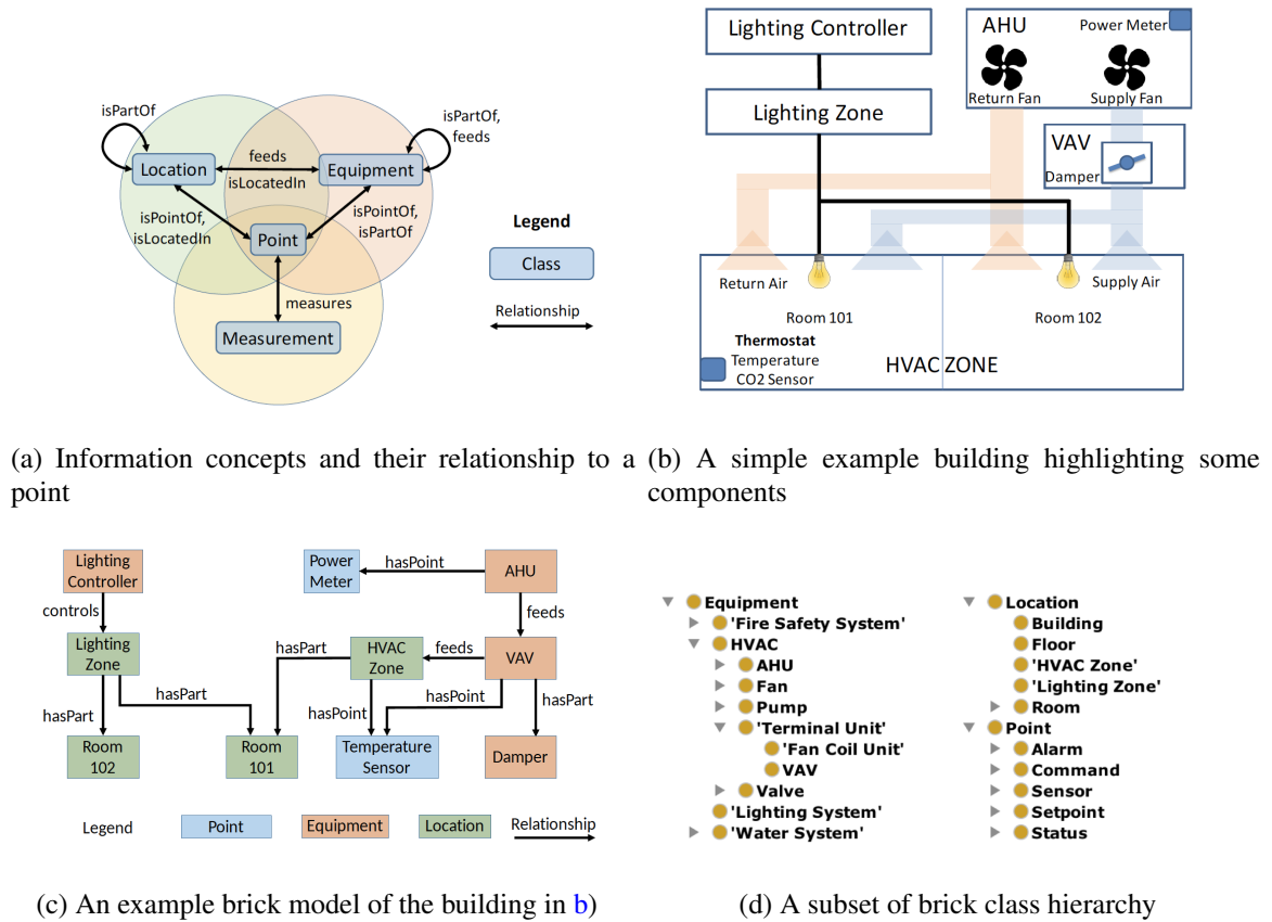
Figure 2.2: Brick information concepts and representations
