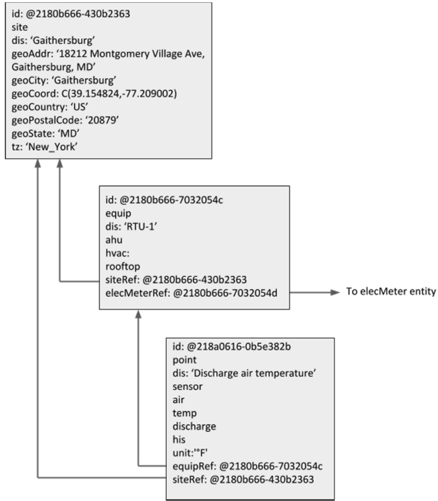
Figure 2.1: A Project Haystack sample project definition for a building in Gaithersburg Source: (Project Haystack, 2025a)
