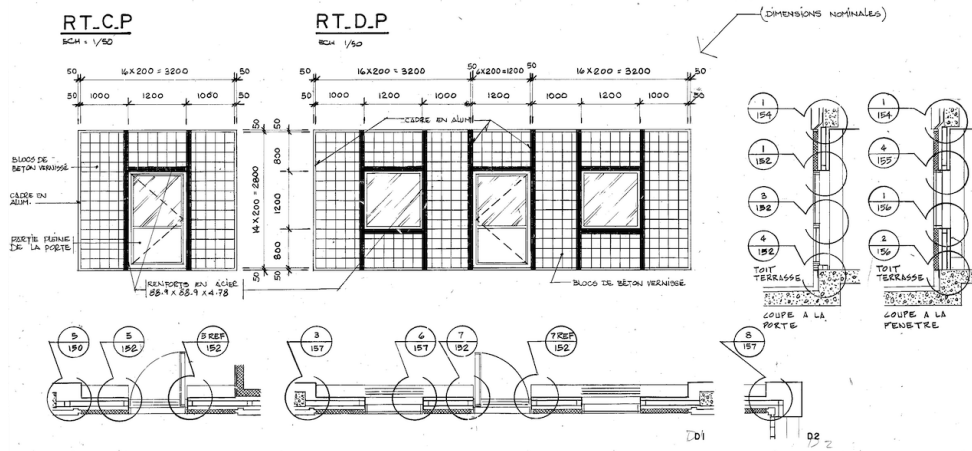
Figure 3.17: A section of the architectural drawings of the LB Building showing labelled (e.g., RT_D_P) block covers with their dimensions and further information (below the block covers) pointing to details of the layers.
