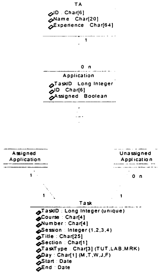
Figure 2.1 Database Abstraction in UML
