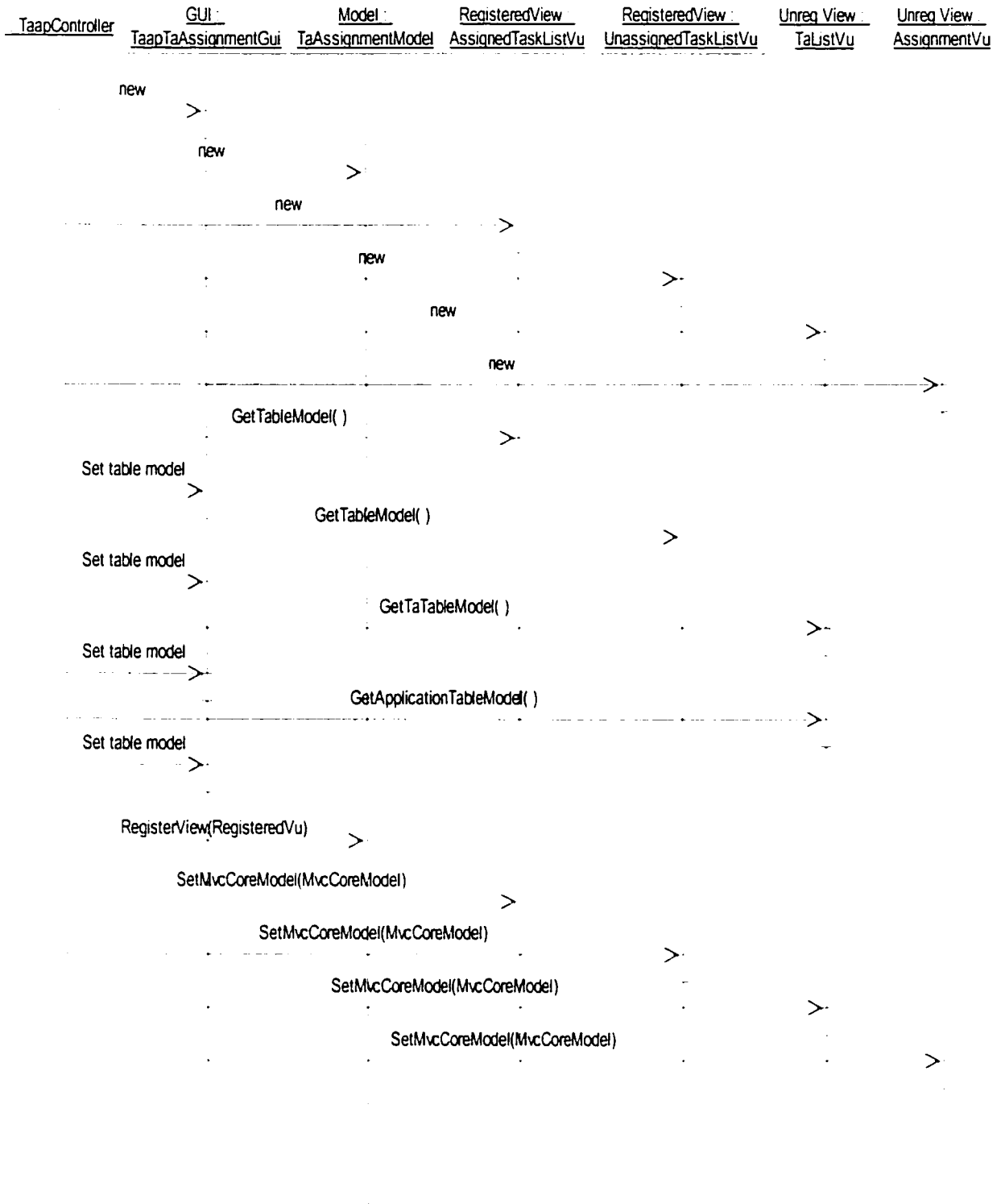
Figure 3.11 Sequence Diagram - Subsystem Initialization
