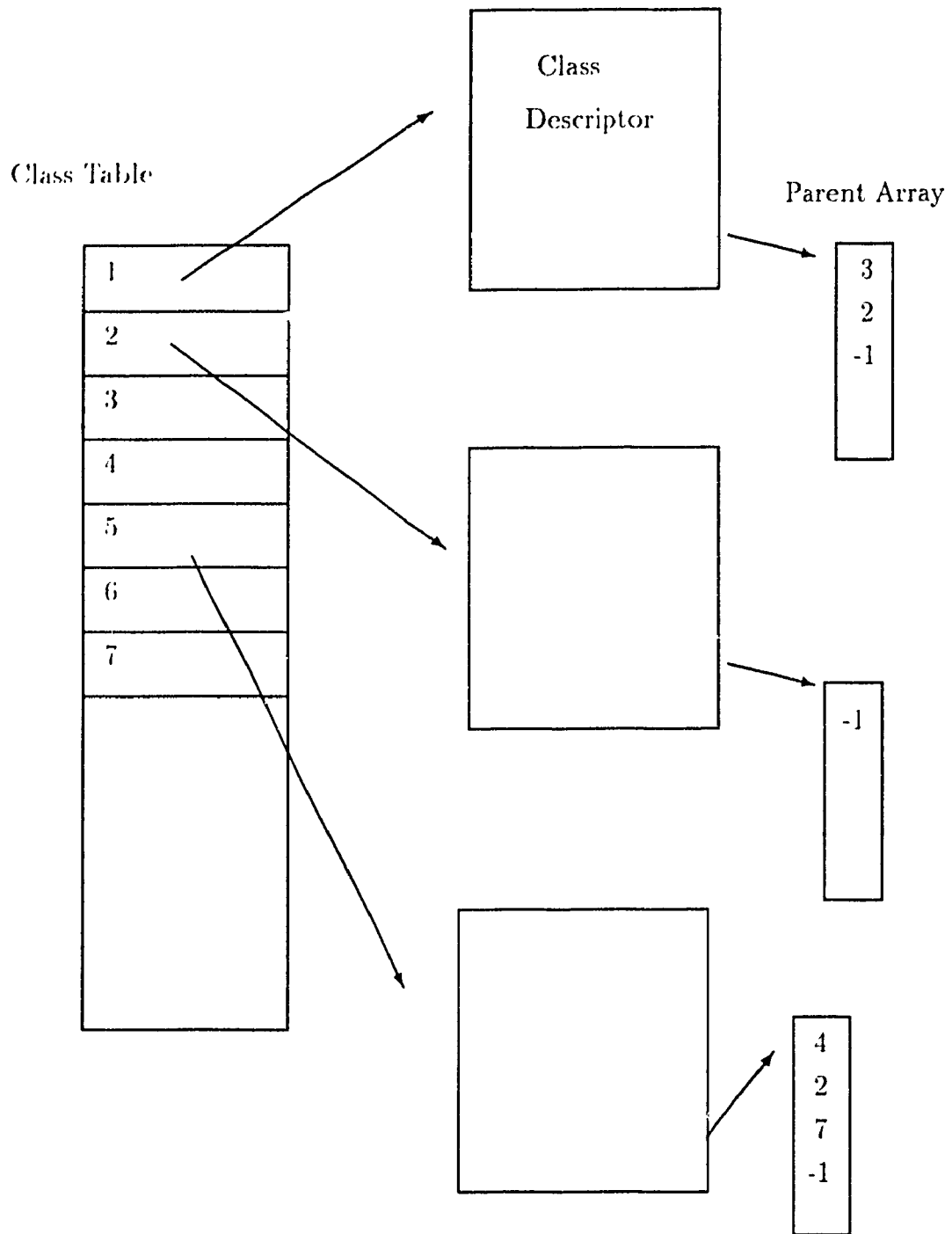
Figure 2.17: Runtime class inheritance graph data structures.
