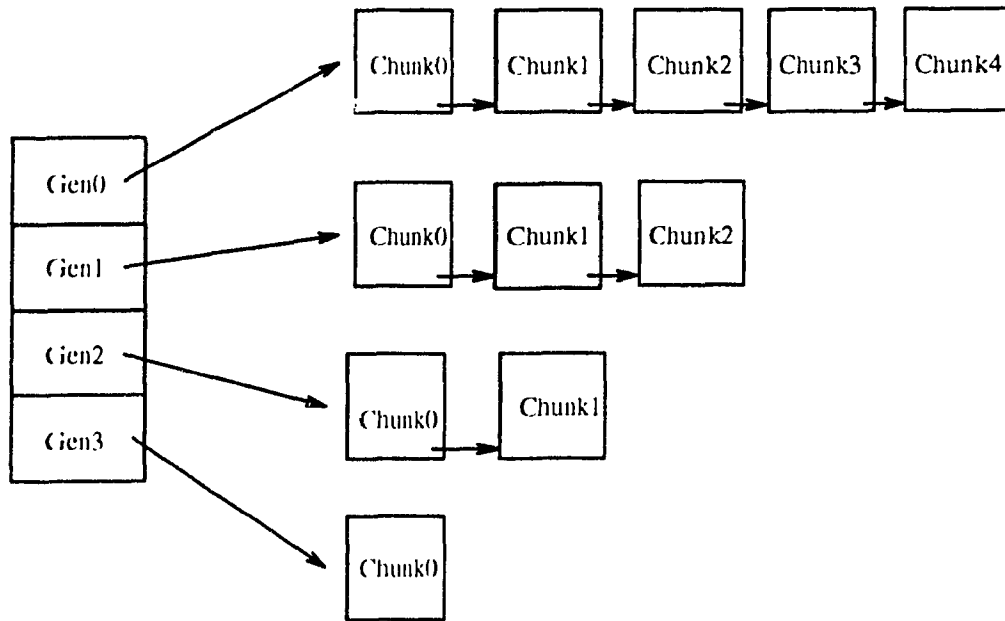
Figure 2.18: The memory management structures used by the collector and allocator. to satisfy the current call to Oballoc() 's needs, a new chunk is still allocated. This helps prevent the collector from being called too frequently as a result of only a small amount of memory being reclaimed.
