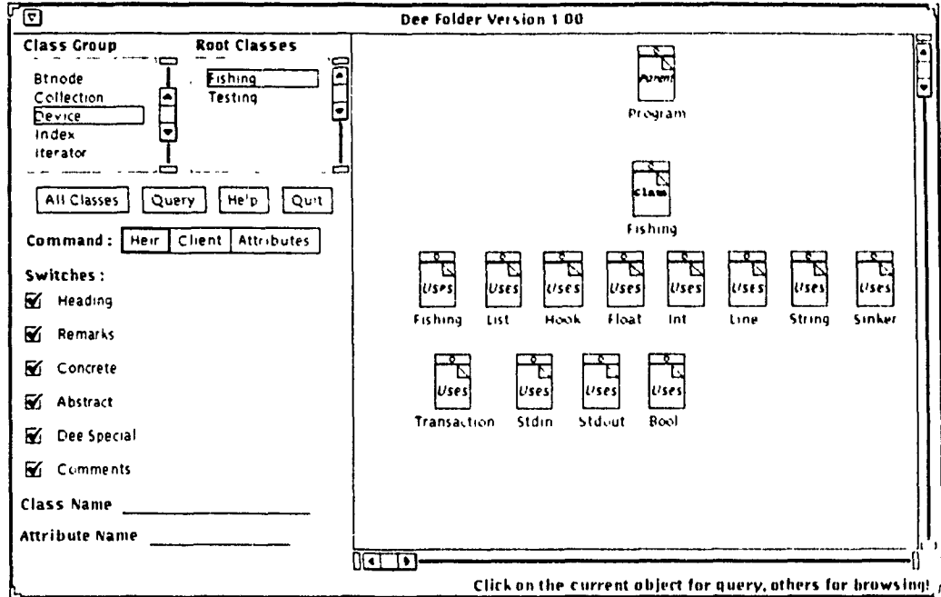
Figure 1.5: An X window running the Dfolder browser.
