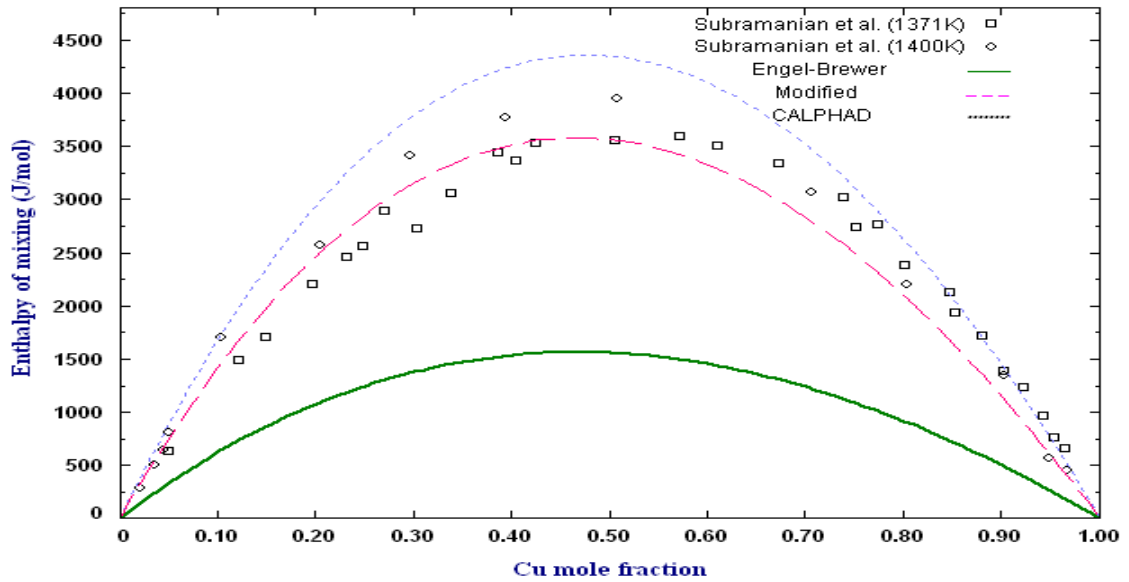
Figure 4-6. Enthalpy of mixing of liquid Ag-Cu at 1400K calculated using Engel-Brewer method — compared with CALPHAD results taken from SGTE database [116] ..... , the enthalpy of mixing obtained by modifying enthalpy parameters of Engel-Brewer method ---, and the experimental data of Subramanian et al. [140] ◊ , ◻
