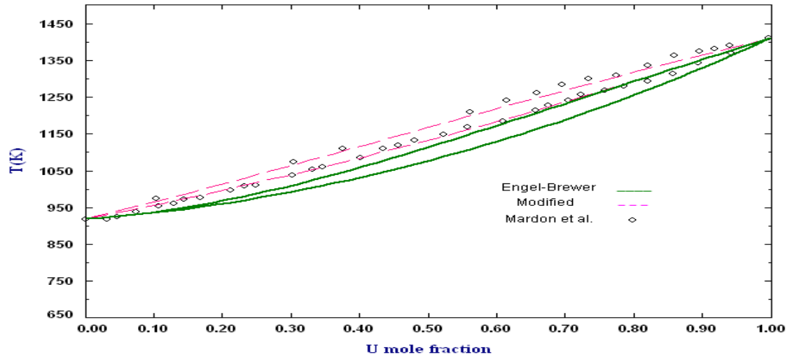
Figure 4-5. Phase diagram of the Np-U system predicted by Engel-Brewer method — compared with the phase diagram obtained by modifying enthalpy parameters of Engel-Brewer method and adding entropy parameters to the Redlich-Kister equation --- and the experimental data of of Mardon et al. [139] \diamond
