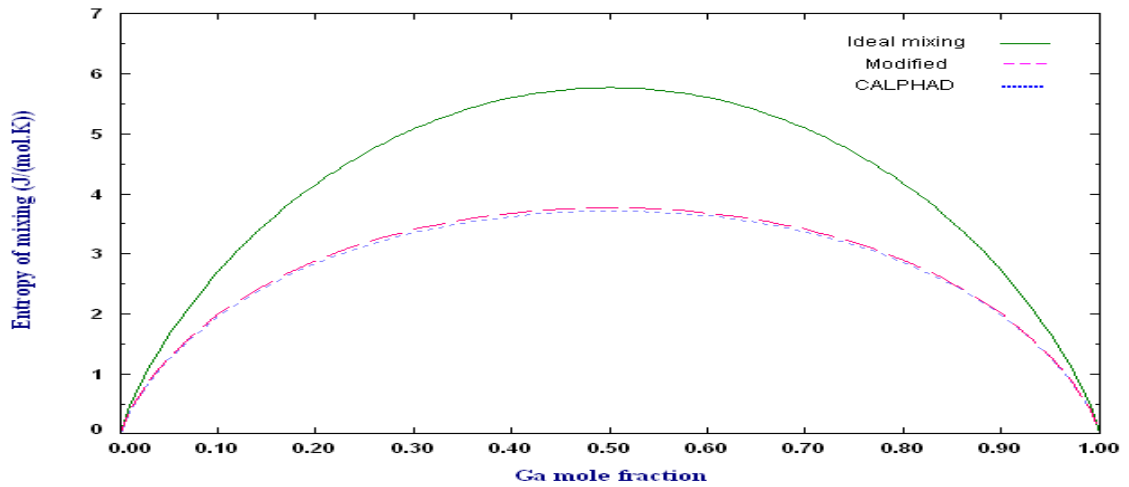
Figure 4-24. Entropy of mixing of the Al-Ga solid solution at 1073K obtained by adding entropy parameters to modified Engel-Brewer database ---, CALPHAD results taken from SGTE database [116] ..... and ideal mixing and the prediction of Engel-Brewer method —
