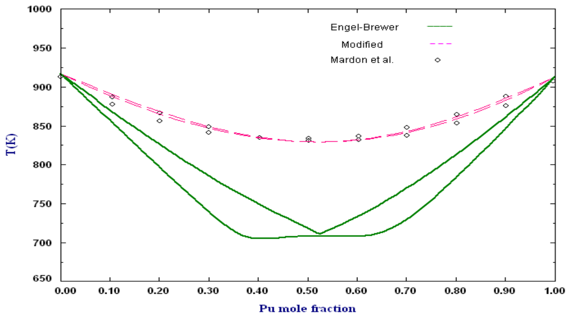
Figure 4-4. Phase diagram of the Np-Pu system predicted by Engel-Brewer method — compared with the phase diagram obtained by modifying enthalpy parameters of Engel-Brewer method and adding entropy parameters to Redlich-Kister equation --- and the experimental data of of Mardon et al. [138] o
