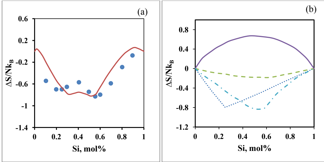
Figure 4-44. (a). Entropy of mixing of Pd-Si ( T=1873K ). \bullet is experimental data of Bergman et al. [181] and solid line is the calculation of Pasturel et al. [168]. (b) Individual contributions to the entropy of mixing calculated by Pasturel et al. [168]. .... is \Delta S^{el} , ..... is \Delta S^{pack} , -- is \Delta S^{gas} and solid line is \Delta S^{id} .
