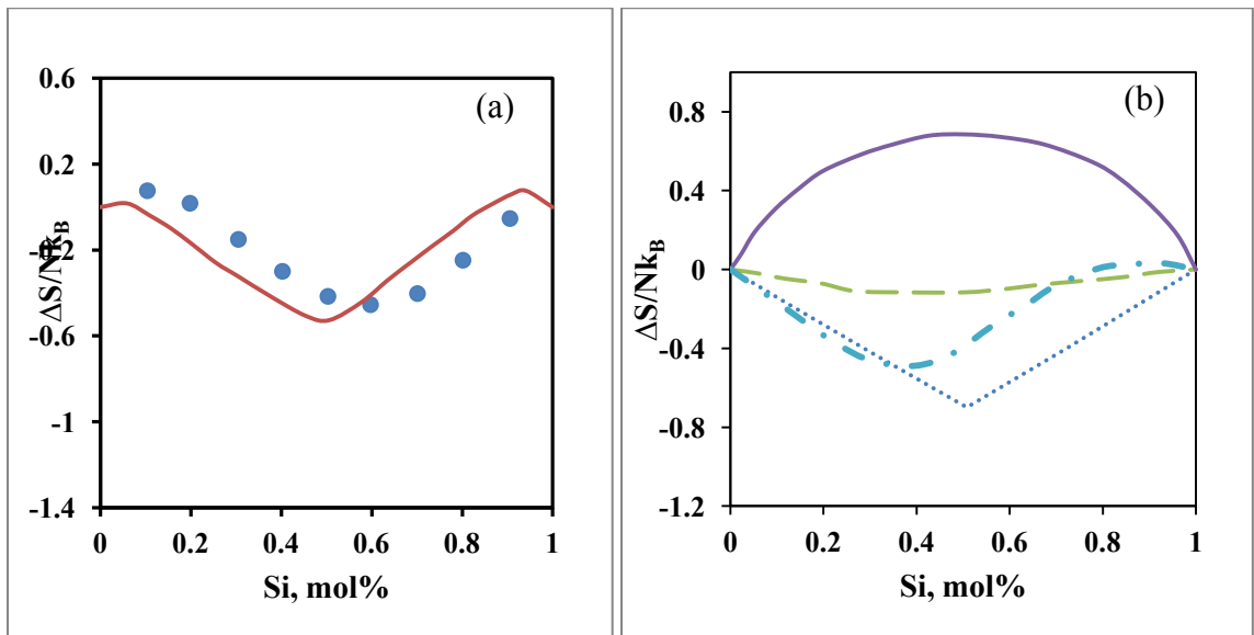
Figure 4-43. (a). Entropy of mixing of Fe-Si ( T=1773K ). \bullet is experimental data of Schwerdtfeger et al. [180] and solid line is the calculation of Pasturel et al. [168]. (b) Individual contributions to the entropy of mixing calculated by Pasturel et al. [168]. .... is \Delta S^{el} , - - - - is \Delta S^{pack} , - - is \Delta S^{gas} and solid line is \Delta S^{id} .
