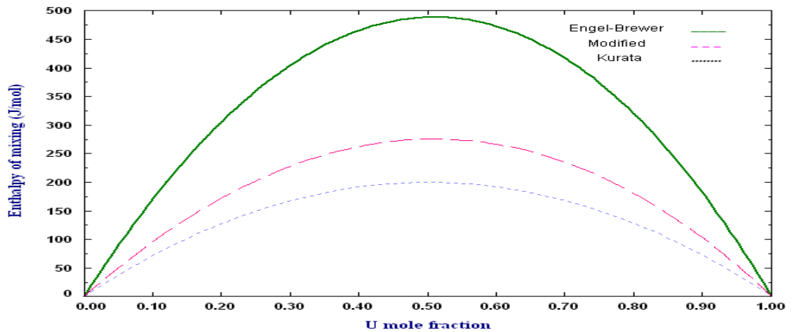
Figure 4-11. Enthalpy of mixing of the Np-U solid solution at 900K calculated using Engel-Brewer method compared with thermodynamic assessment of Kurata [129] and the enthalpy of mixing obtained by modifying enthalpy parameters of Engel-Brewer method ---
