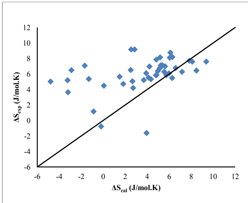
Figure 4-38. Calculated entropy of mixing using Sommer relation [27] compared with the experimental entropy of mixing at equiatomic composition for liquid alloys of the 49 binary systems listed in Table 4-6.
