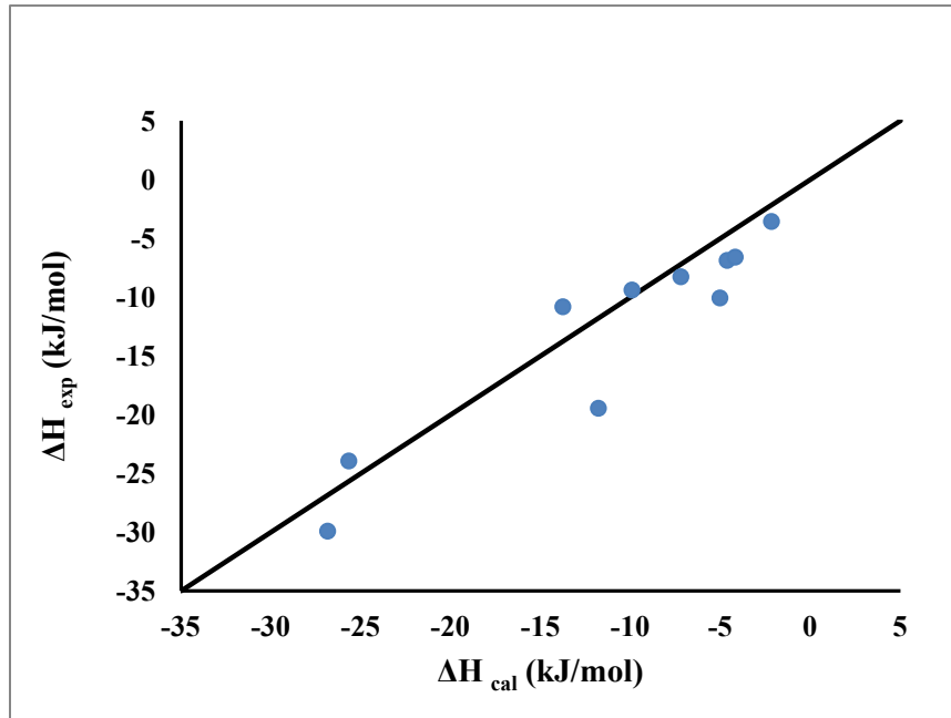
Figure 4-31. Extremum enthalpy of mixing calculated using Miedema model compared with the experimental enthalpy of mixing for the liquid phase of p-metals alloyed with d^{10} transition metals listed in Table 4-3.
