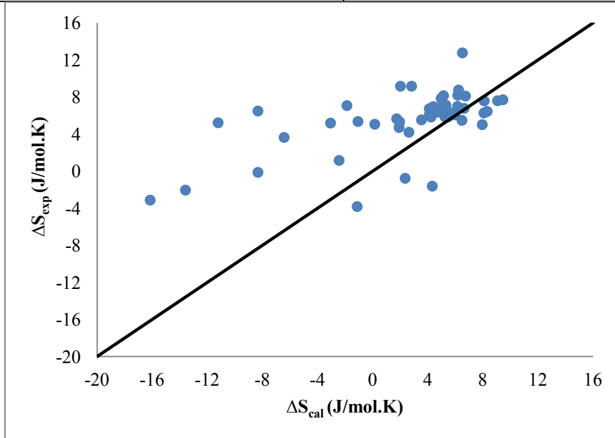
Figure 4-39. Calculated entropy of mixing using \Delta H_{exp} . instead of \Delta H_{Miedema} in Sommer relation [27] compared with the experimental entropy of mixing at equiatomic composition for liquid alloys of the 49 binary systems listed in
