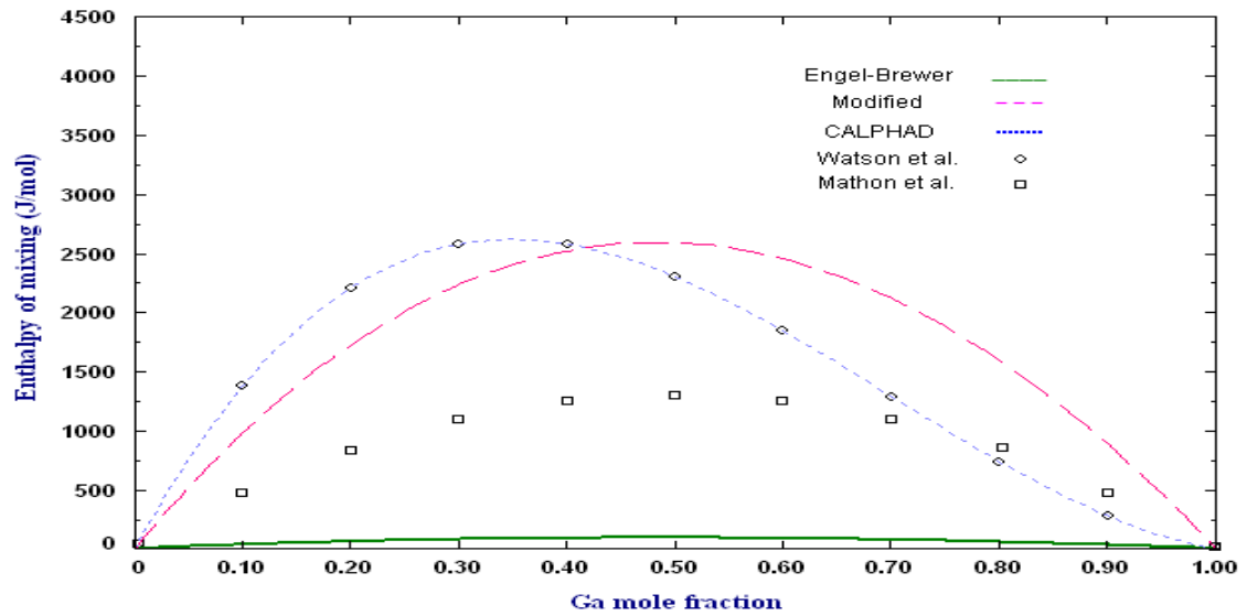
Figure 4-9 show that for the Al-Ga system, the enthalpy of mixing for the liquid and the solid solutions is asymmetric. Since Engel-Brewer method does not take into account size mismatch in alloying, it is not able to predict asymmetry.
