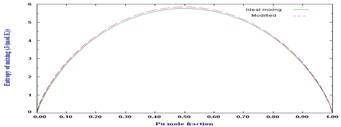
Figure 4-19. Entropy of mixing of the Np-Pu solid solution at 850K obtained by adding entropy parameters to modified Engel-Brewer database ---, ideal mixing and the prediction of Kurata [129] and Engel-Brewer method —
