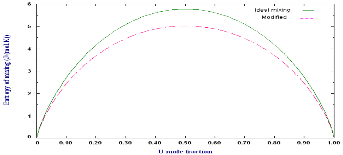
Figure 4-20. Entropy of mixing of the Pu-U solid solution at 900K obtained by adding entropy parameters to modified Engel-Brewer database ---, ideal mixing and the prediction of Kurata [128] and Engel-Brewer method —
