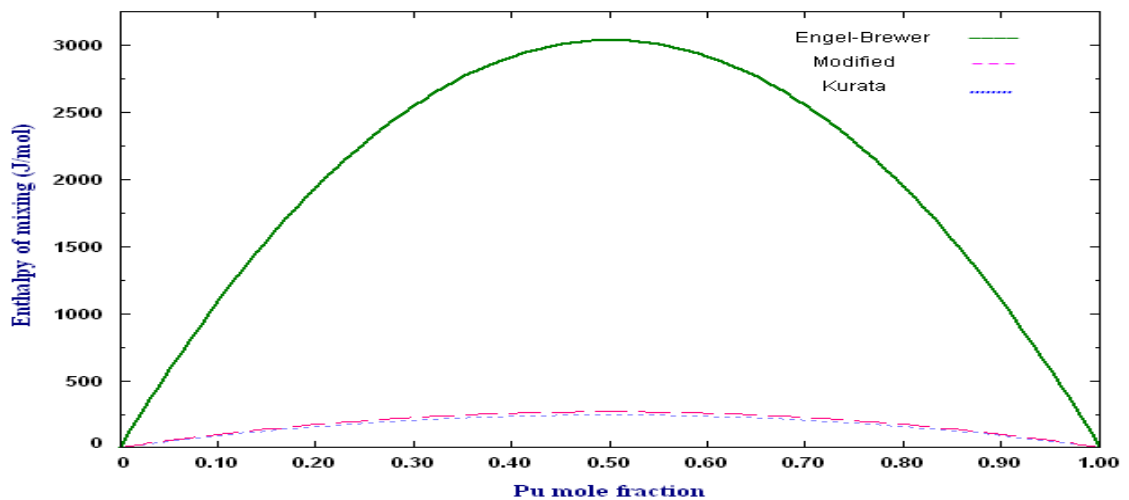
Figure 4-13. Enthalpy of mixing of Np-Pu solid solution at 850K calculated using Engel-Brewer method — compared with thermodynamic assessment of Kurata [129] ..... and the enthalpy of mixing by modifying enthalpy parameters of Engel-Brewer method [129] ---
