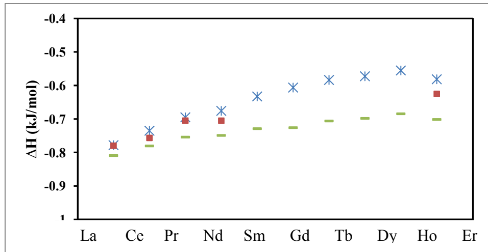
Figure 4-34. Predicted enthalpy of mixing of Zn-RE liquid alloys at x_{RE}=0.005 using modified Miedema hybridization parameters, proposed by Colinet et al. [153] compared with the experimental data and classical Miedema parameters. ■ is the experimental data of [156-158] . * is calculated enthalpy of mixing at x_{RE} = 0.005 at% using new Miedema hybridization parameters and - is calculations with classical Miedema parameters.
