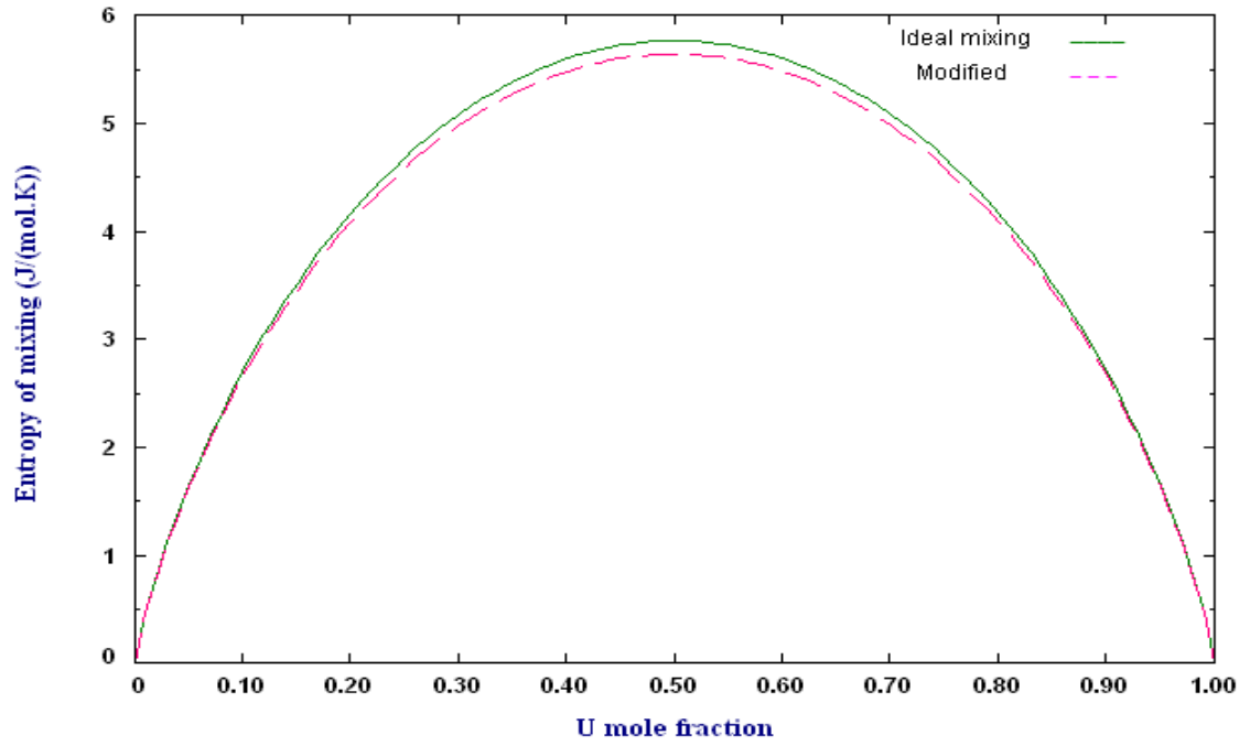
Figure 4-16. Entropy of mixing of liquid Np-U at 1500K obtained by adding entropy parameters to modified Engel-Brewer database ---, ideal mixing and the prediction of Kurata [129] and Engel-Brewer method —
