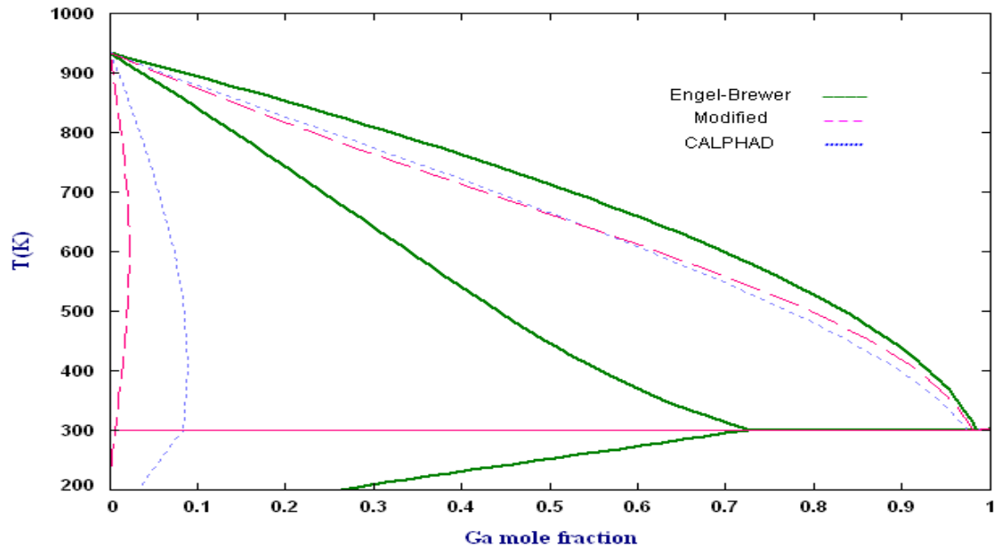
Figure 4-2. Phase diagram of the Al-Ga system predicted by Engel-Brewer method — compared with the phase diagram obtained by modifying enthalpy parameters of Engel-Brewer method and adding entropy parameters to the Redlich-Kister equation --- and CALPHAD results taken from SGTE database [116] ....
