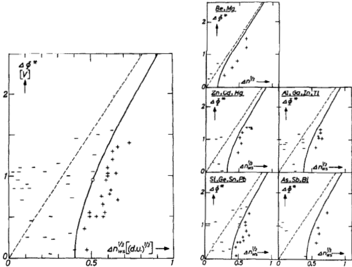
Figure 2-4. The sign of heat of mixing for liquid binary alloys of transition metals with non-transition metals at equiatomic composition. The - sign means \Delta H_{mix} < -2511 \frac{\text{kJ}}{\text{mol}} (-600 \frac{\text{cal}}{\text{mol}}) and the + sign means \Delta H_{mix} > 2511 \frac{\text{kJ}}{\text{mol}} (+600 \frac{\text{cal}}{\text{mol}}) or the solubility of one of the metals is very small at temperatures near 1000K or higher. The dashed line represents chemical contribution without considering the R term and the curve represents chemical contribution after R term. [75]
