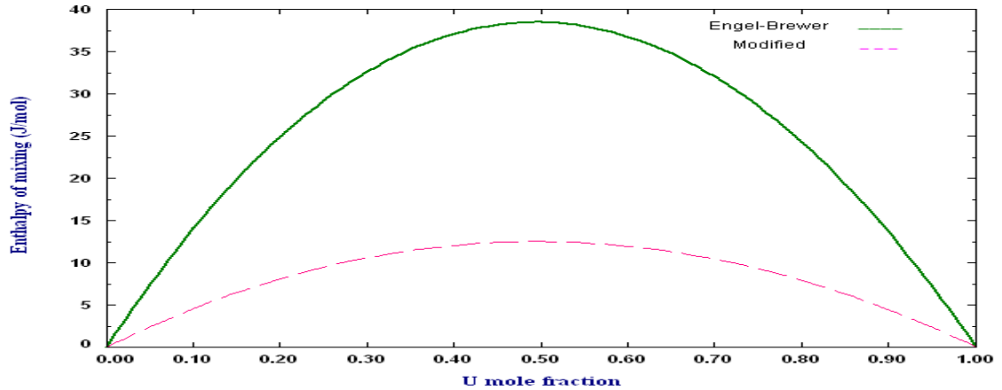
Figure 4-10. Enthalpy of mixing of liquid Np-U at 1500K calculated using Engel-Brewer method — compared with the enthalpy of mixing obtained by modifying enthalpy parameters of Engel-Brewer method ----. For this phase, Kurata [129] predicted ideal enthalpy of mixing —
