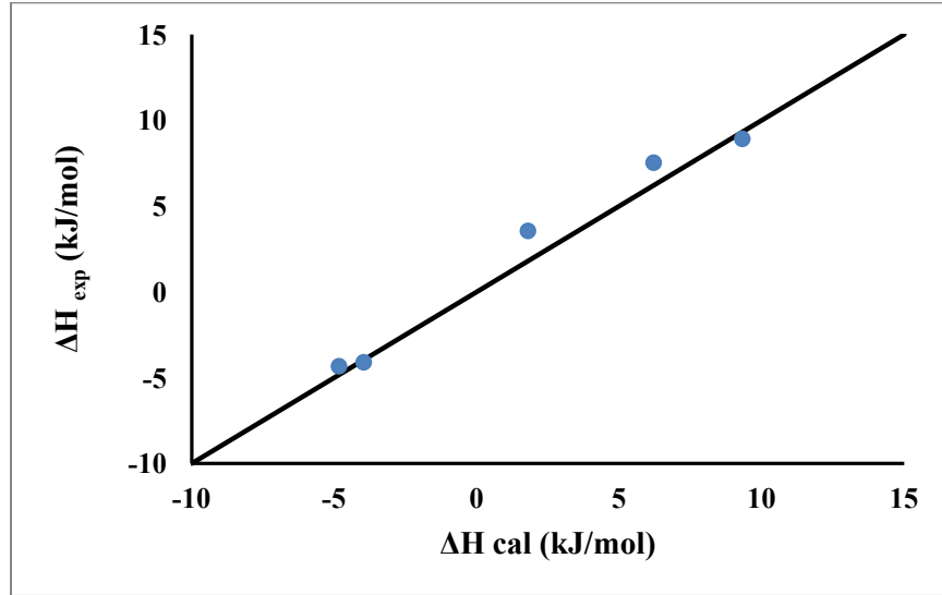
Figure 4-28. Extremum enthalpy of mixing calculated using Miedema model compared with the experimental enthalpy of mixing for the liquid phase of transition metals alloys listed in Table 4-3.
