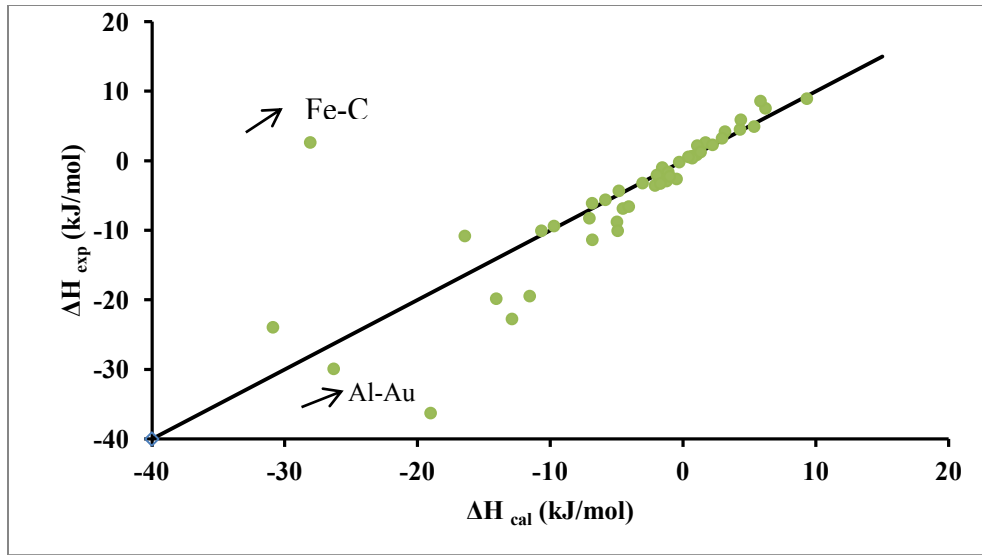
Figure 4-26. Extremum enthalpy of mixing calculated using Miedema model compared with the experimental enthalpy of mixing for liquid alloys of 50 binary systems listed in Table 4-2.
