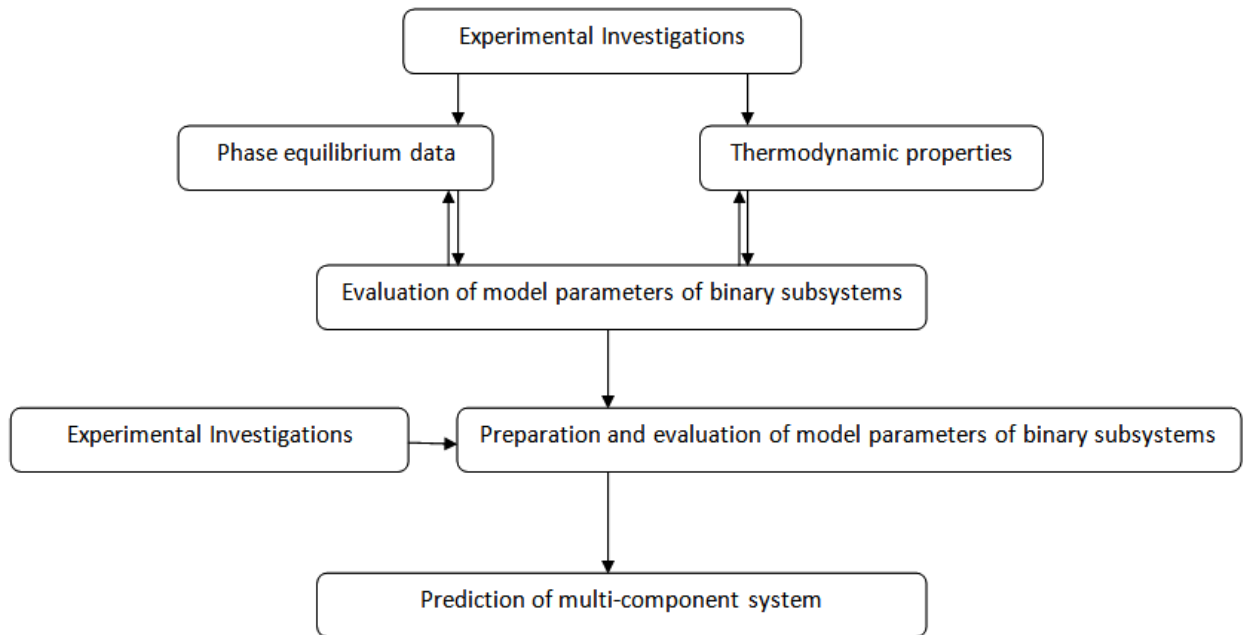
Figure 1-1. Schematic of the CALPHAD method
