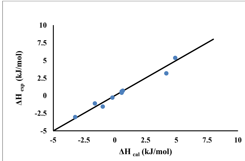
Figure 4-30. Extremum enthalpy of mixing calculated using Miedema model compared with the experimental enthalpy of mixing for the liquid phase of p -metals alloyed with other p -metals listed in Table 4-3.
