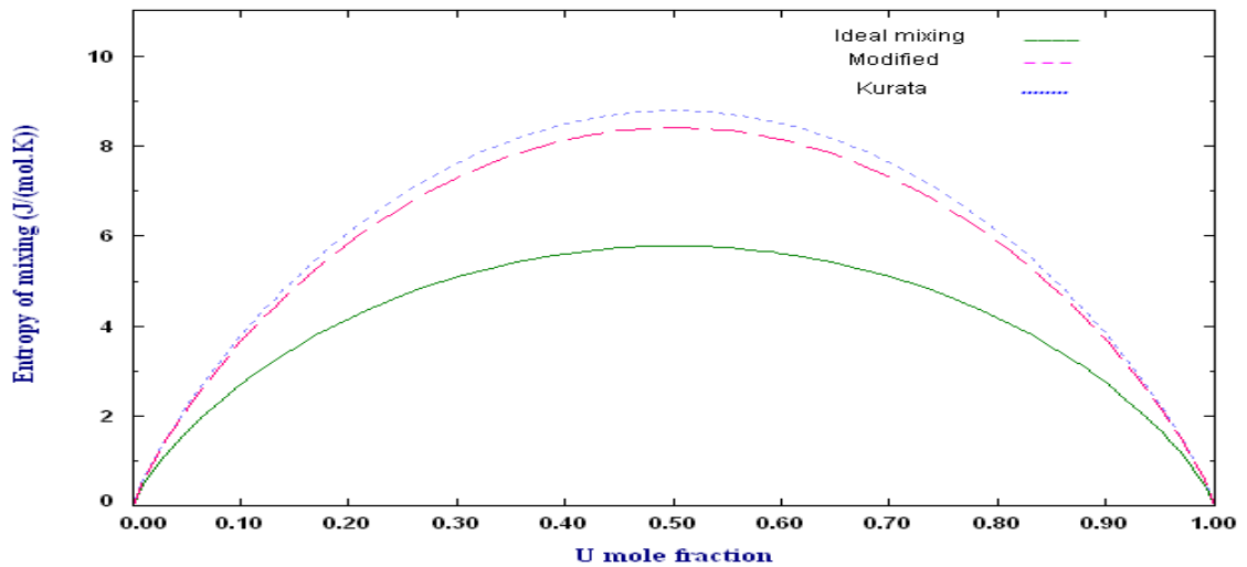
Figure 4-21. Entropy of mixing of liquid Pu-U at 1050K calculated obtained by adding entropy parameters to modified Engel-Brewer database ---, thermodynamic assessment of Kurata [128] ..... and ideal mixing and the prediction of Engel-Brewer method —
