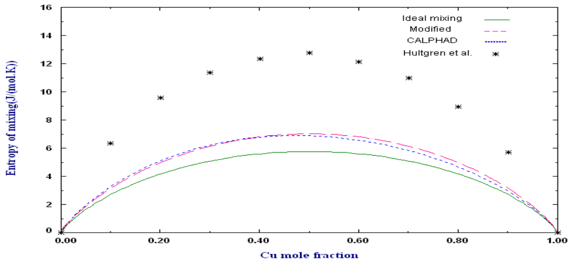
Figure 4-22. Entropy of mixing of liquid Ag-Cu at 1400K obtained by adding entropy parameters to modified Engel-Brewer database ---, CALPHAD results taken from SGTE database [116] ....., thermodynamic assessment of Hultgren et al. [141] * and ideal mixing and the prediction of Engel-Brewer method —
