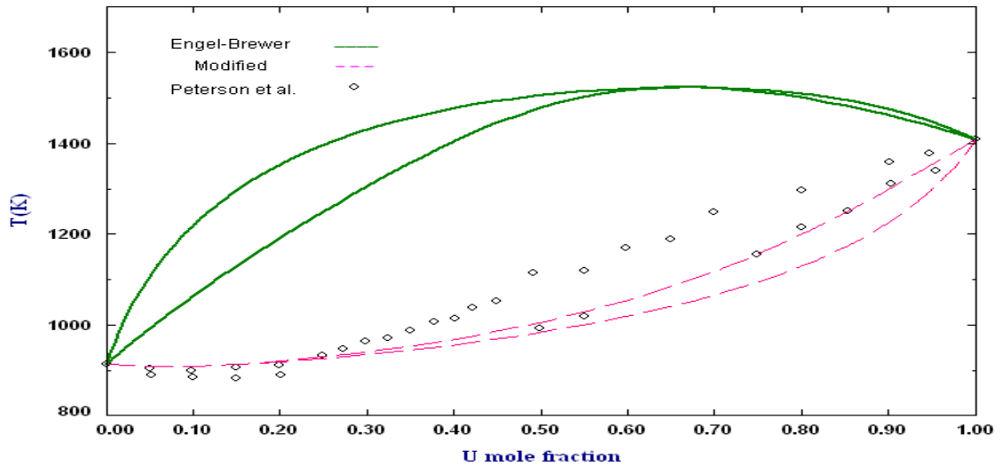
Figure 4-3. Phase diagram of the Pu-U system predicted by Engel-Brewer method — compared with the phase diagram obtained by modifying enthalpy parameters of Engel-Brewer method and adding entropy parameters to the Redlich-Kister equation --- and the experimental data of Peterson et al. [137] o
