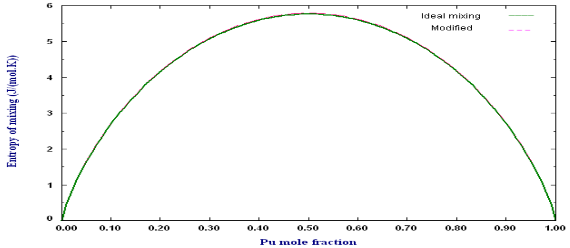
Figure 4-18. Entropy of mixing of liquid Np-Pu at 1050K obtained by adding entropy parameters to modified Engel-Brewer database ---, ideal mixing and the prediction of Kurata [129] and Engel-Brewer method —
