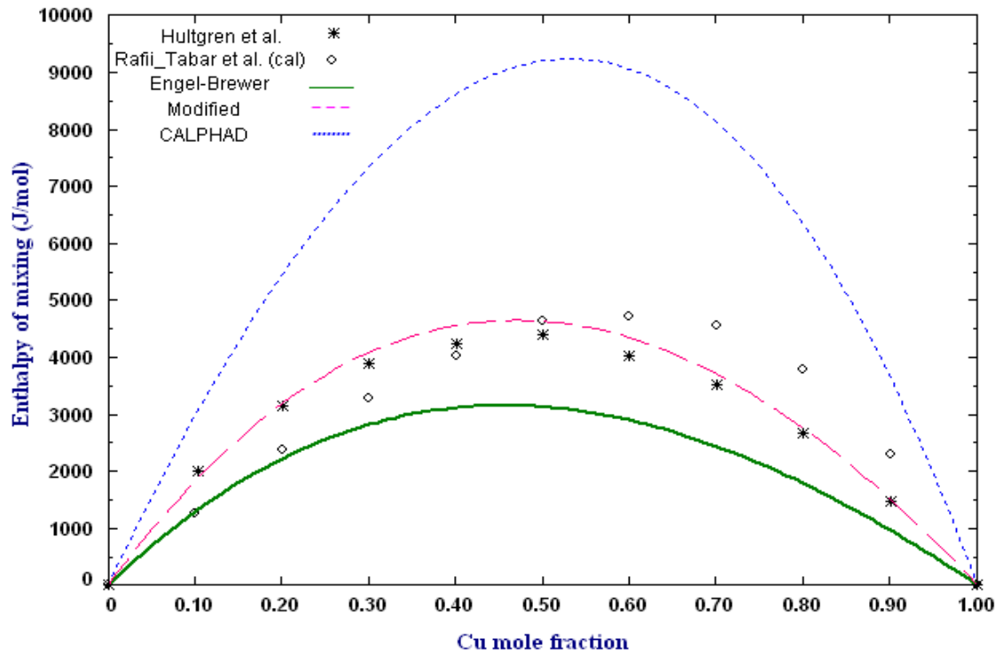
Figure 4-7. Enthalpy of mixing of the the Ag-Cu solid solution at 300K calculated using Engel-Brewer method — compared with CALPHAD results taken from SGTE database [116] ....., the enthalpy of mixing obtained by modifying enthalpy parameters of Engel-Brewer method ---, and thermodynamic assessment of Hultgren et al. * [141] and Rafii-Tabar et al. [142] ◇
