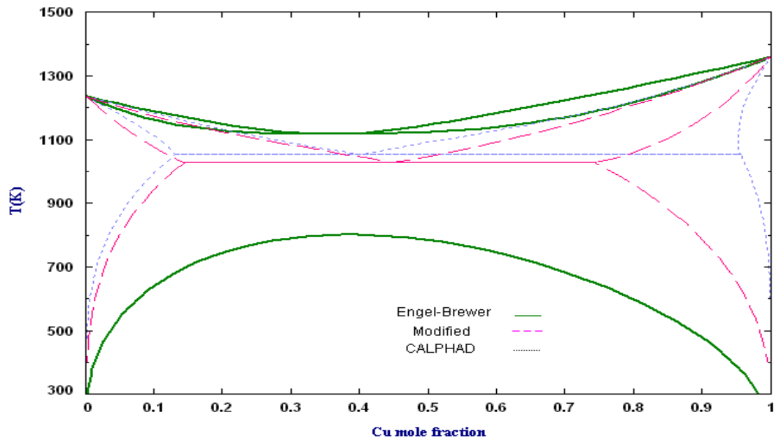
Figure 4-1. Phase diagram of the Ag-Cu system predicted by Engel-Brewer method — compared with the phase diagram obtained by modifying enthalpy parameters of Engel-Brewer method and adding entropy parameters to the Redlich-Kister equation --- and CALPHAD results taken from SGTE database [116] ....
