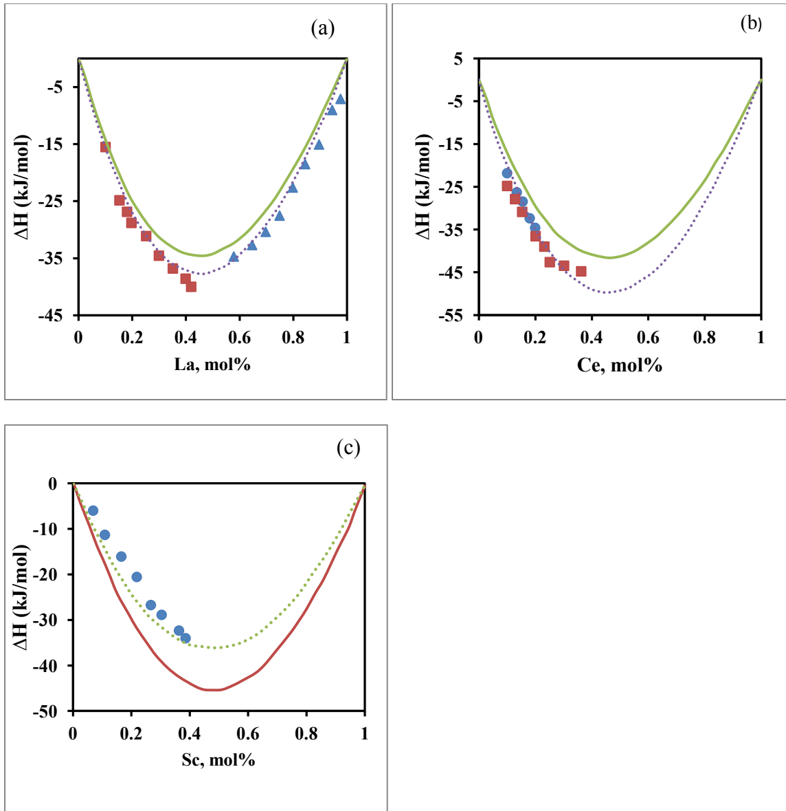
Figure 4-35. Comparison of enthalpy of mixing of Al-RE systems calculated with classical Miedema parameters and modified Miedema parameters with the experimental data. — is calculations by classical Miedema parameters and .... is calculations using new Miedema parameters by Zhan et al. [159] (a) Al-La system. ■ is the experimental data of Esin et al. [160] at 1920K, ▲ is the experimental data of Sommer et al. [161] at 1200K, (b) Al-Ce system. ■ is the experimental data of Esin et al. [162] at 1870K, ● is the experimental data of Zviadadze et al. [163] at 1250K. (c) Al-Sc system, ● is the experimental data of Litovskii et al. [164] at 1873K
