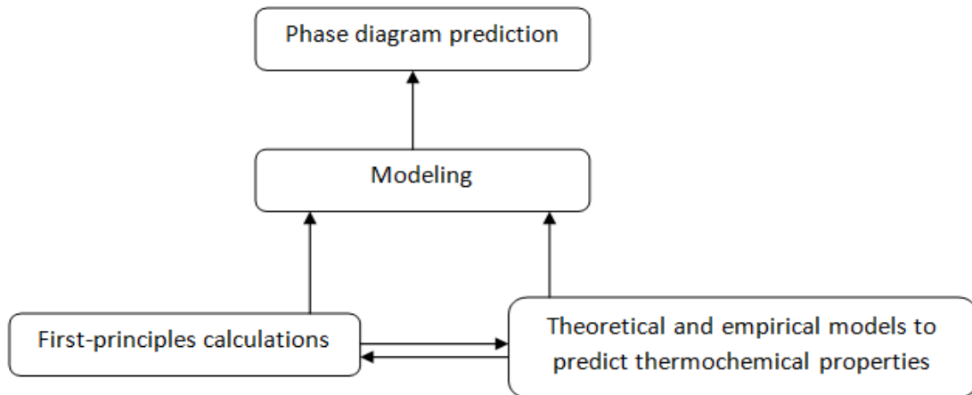
Figure 1-2. Methodology of phase diagram prediction for systems lacking experimental phase equilibrium data and thermodynamic properties data
