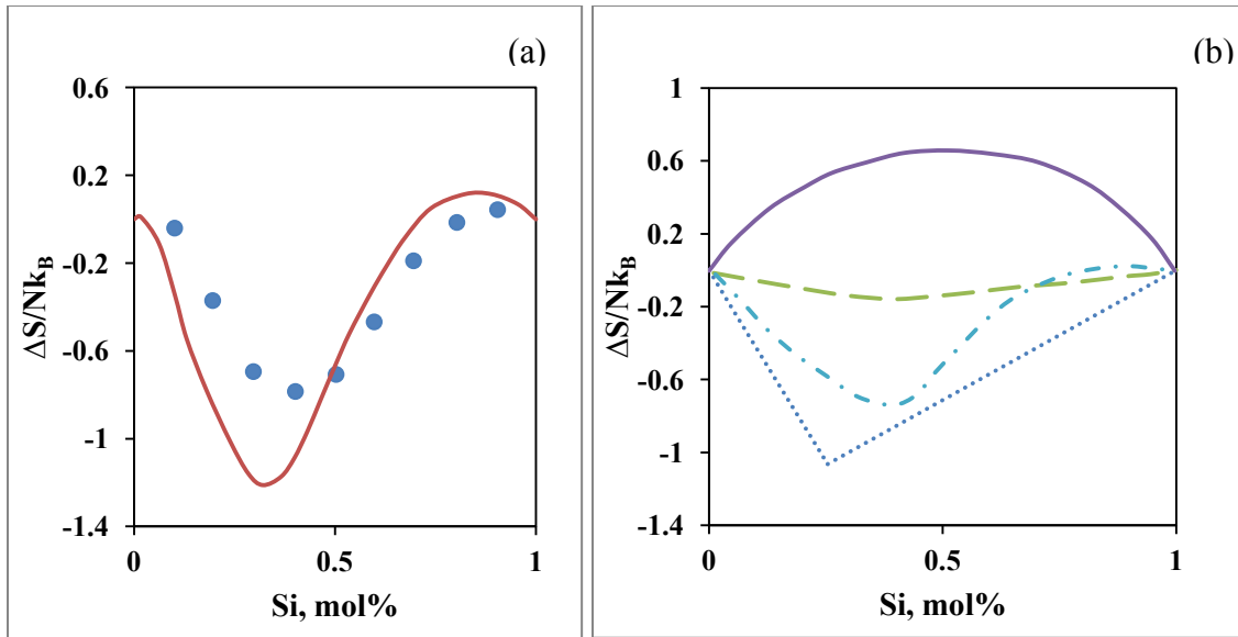
Figure 4-42. (a). Entropy of mixing of Ni-Si ( T=1773K ). \bullet is experimental data of Schwerdtfeger et al. [179] and solid line is the calculation of Pasturel et al. [168]. (b) Individual contributions to the entropy of mixing calculated by Pasturel et al. [168]. .... is \Delta S^{el} , - - - - is \Delta S^{pack} , - - is \Delta S^{gas} and solid line is \Delta S^{id} .
