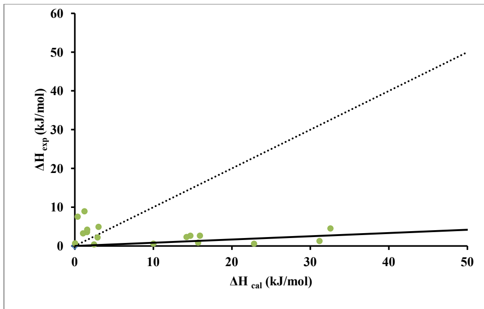
Figure 4-27. Extremum enthalpy of mixing calculated using Engel-Brewer method compared with the experimental enthalpy of mixing for liquid alloys of 20 binary systems listed in Table 4-2.
