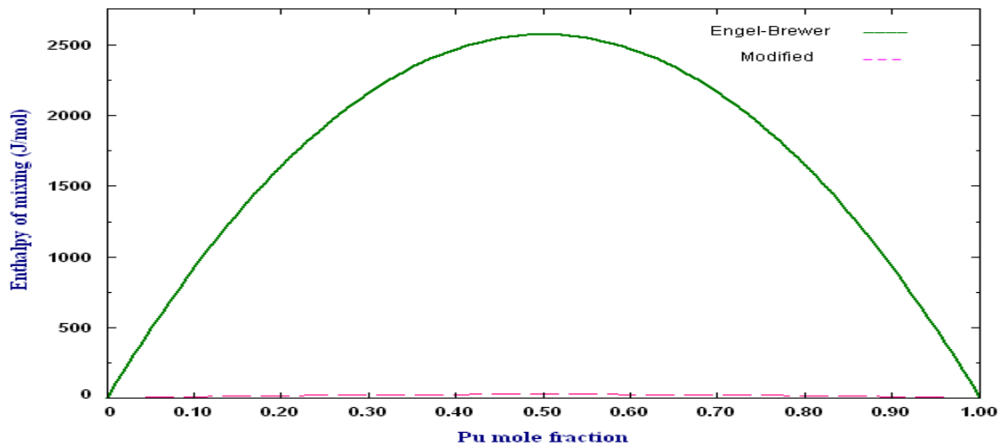
Figure 4-12. Enthalpy of mixing of liquid Np-Pu at 1050K calculated using Engel-Brewer method — compared with enthalpy of mixing obtained by modifying enthalpy parameters of Engel-Brewer method ---. For this phase Kurata [129] predicted ideal enthalpy of mixing —
