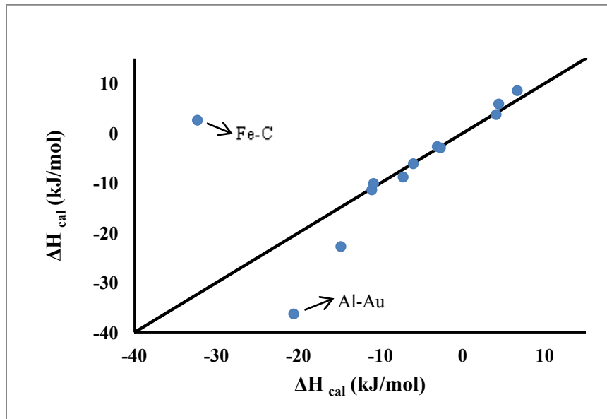
Figure 4-28. Extremum enthalpy of mixing calculated using Miedema model compared with the experimental enthalpy of mixing for the liquid phase of transition metals alloys listed in Table 4-3.
