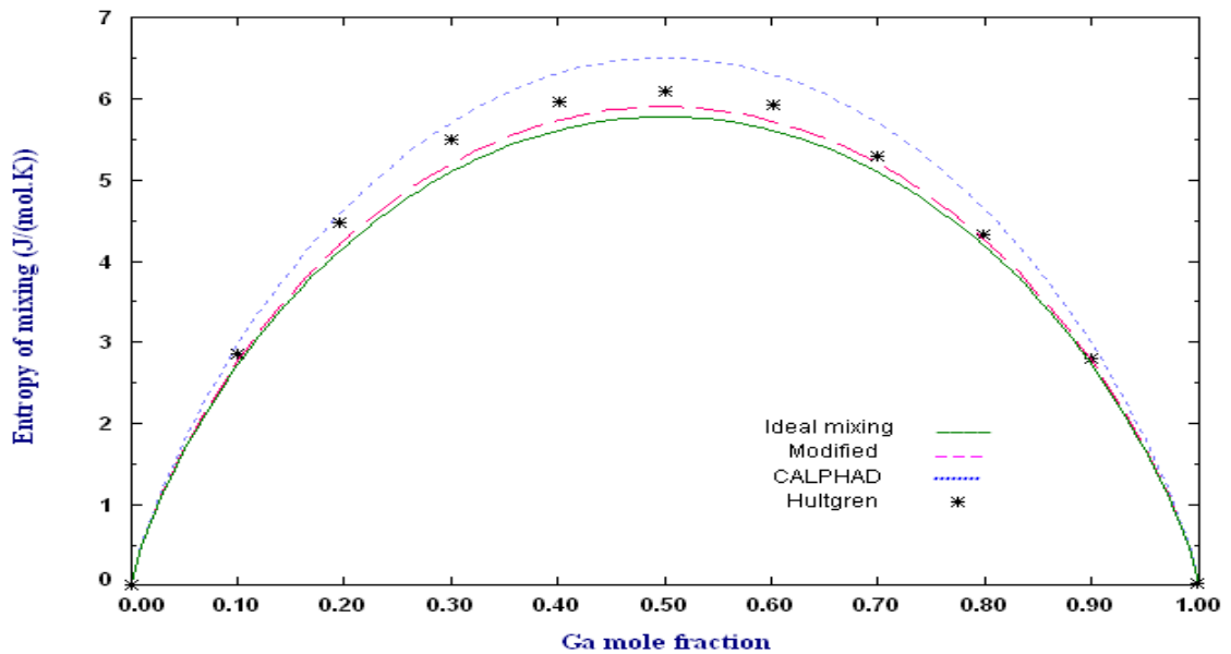
Figure 4-25. Entropy of mixing of liquid Al-Ga at 1073K obtained by adding entropy parameters to modified Engel-Brewer database ---, CALPHAD results taken from SGTE database [116] ....., assessment of Hultgren et al. [141] * and ideal mixing and the prediction of Engel-Brewer method —
