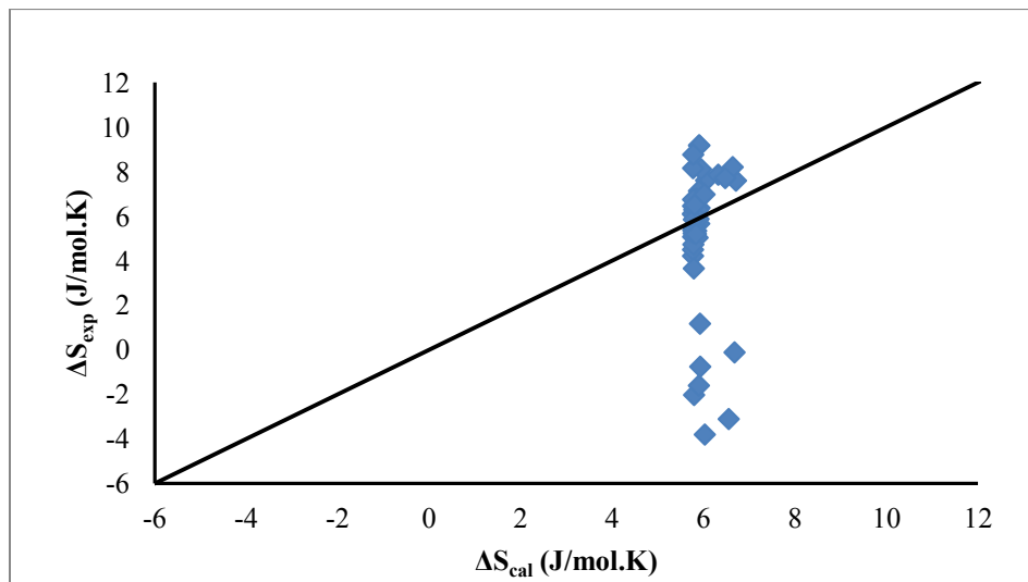
Figure 4-36. Calculated entropy of mixing by Faber relation [24] compared with the experimental entropy of mixing at equiatomic composition for liquid alloys of 49 binary systems listed in Table 4-6.
