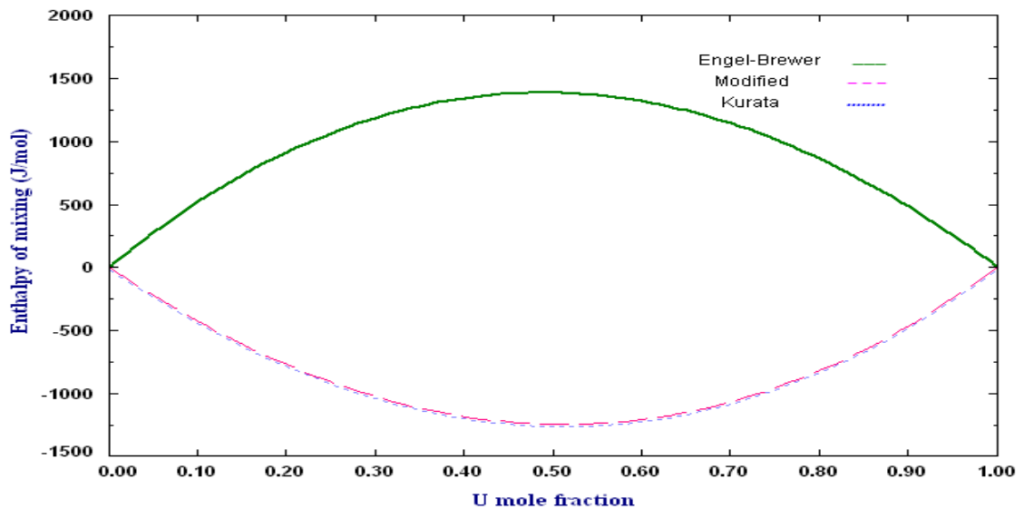
Figure 4-15. Enthalpy of mixing of the Pu-U solid solution at 900K calculated using Engel-Brewer method — compared with thermodynamic assessment of Kurata [128] .... and the enthalpy of mixing obtained by modifying enthalpy parameters of Engel-Brewer method to reproduce the phase diagram reported by Kurata [128] ---
