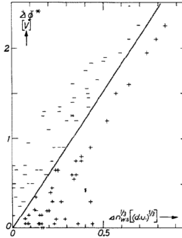
Figure 2-3. The sign of heat of mixing for binary liquid alloys of two non-transition metals at equiatomic composition plotted as a function of \Delta\phi^* and \Delta n_{ws} . The - sign means \Delta H_{mix} < -2511 \frac{\text{kJ}}{\text{mol}} (-600 \frac{\text{cal}}{\text{mol}}) and the sign + means \Delta H_{mix} > 2511 \frac{\text{kJ}}{\text{mol}} (+600 \frac{\text{cal}}{\text{mol}}) or the solubility of one of the metals is very small at temperatures near 1000K or higher [75]
