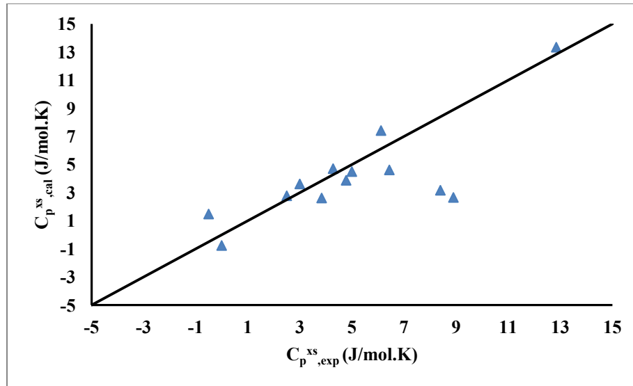
Figure 4-41. Heat capacities of binary liquid alloys calculated by Wituciewicz relation [31] and compared with the experimental data listed in Table 4-7. Enthalpy of mixing used in the calculations are obtained from Miedema model.
