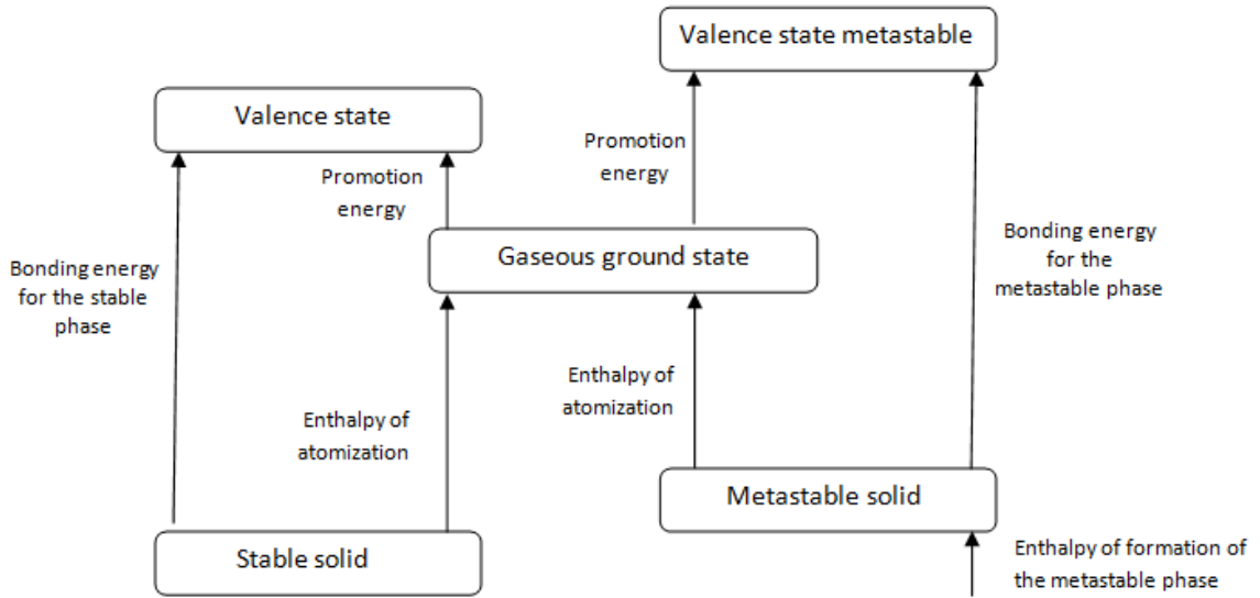
Figure 2-1. Modified Born-Haber cycle for metallic elements [47]
