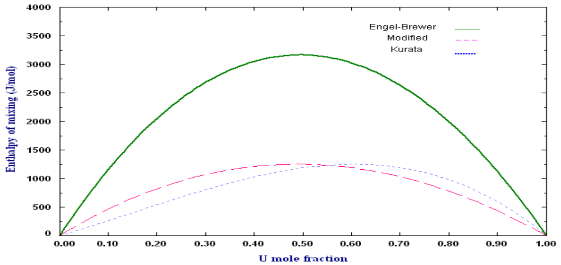
Figure 4-14. . Enthalpy of mixing of liquid Pu-U at 1500K calculated using Engel-Brewer method — compared with thermodynamic assessment of Kurata [128] .... and the enthalpy of mixing obtained by modifying enthalpy parameters of Engel-Brewer method ---
