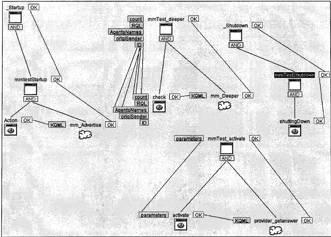
Figure 5.7: Plan file of provider agent.
