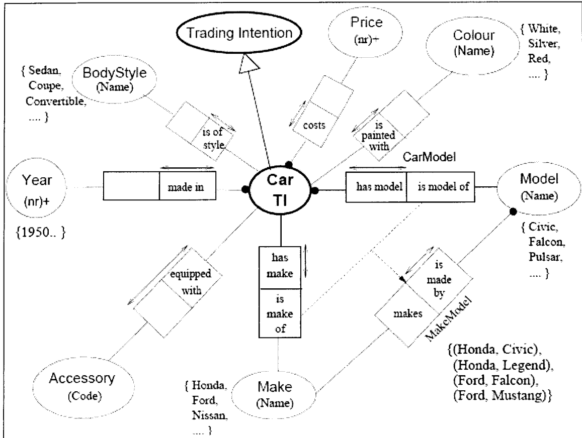
Figure 7.1: Schema for Trading Intentions for Cars [34].
