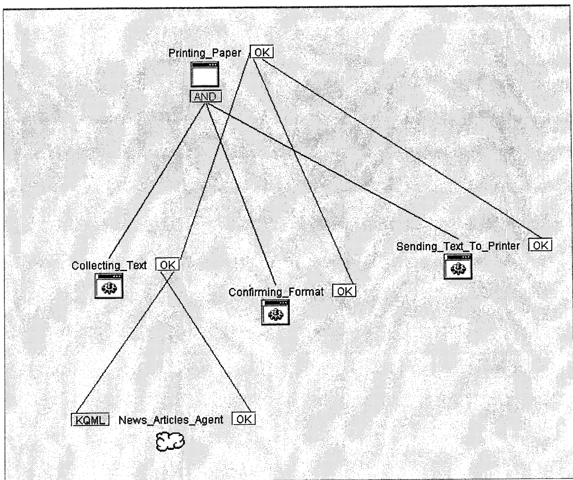
Figure 5.2: Plan file for the printing example.
