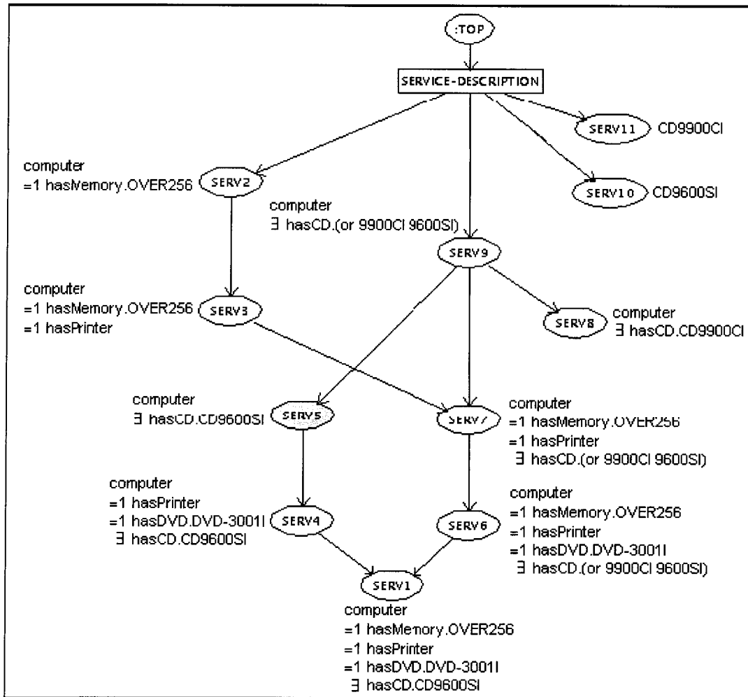
Figure 7.3: Service description branch of the subsumption tree [35].
