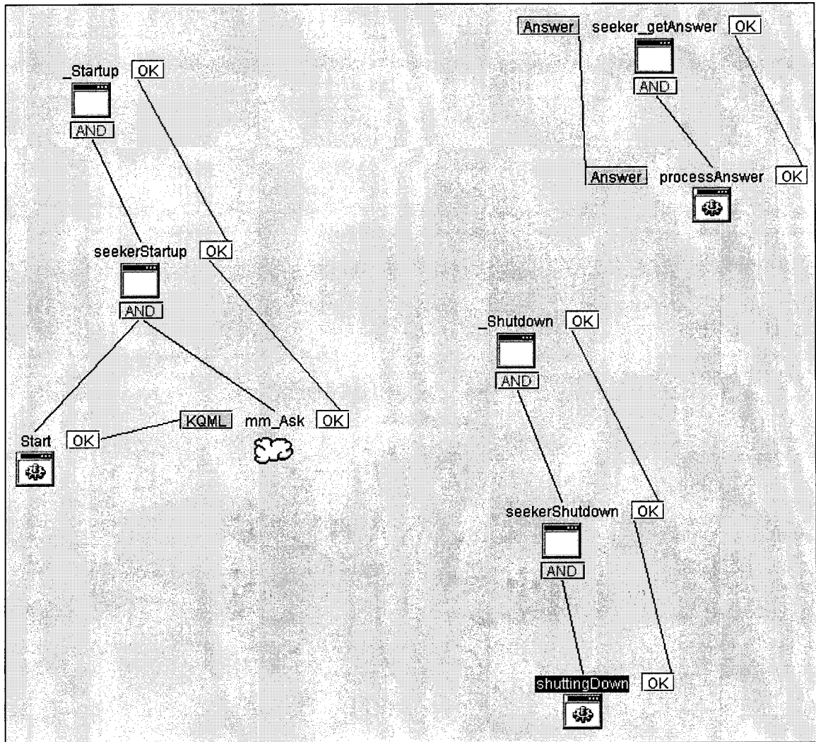
Figure 5.8: Seeker's plan file
