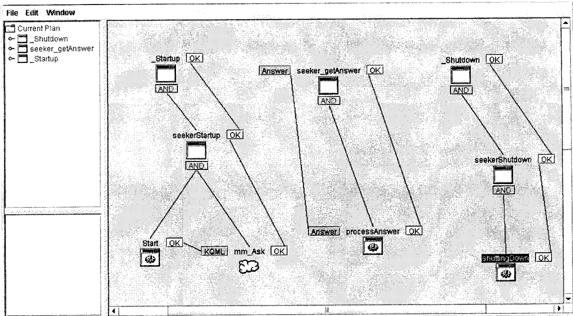
Figure 3.9: Example of a plan file
