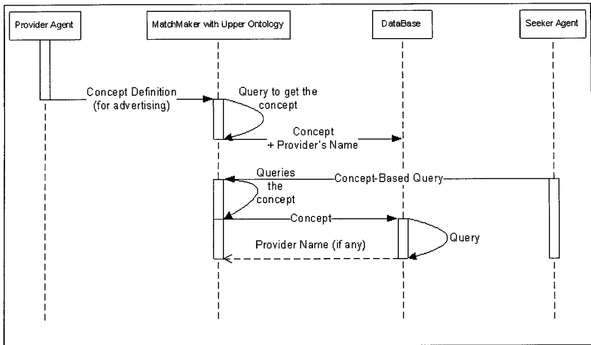
Figure 5.6: Sequence diagram for the upper ontology
