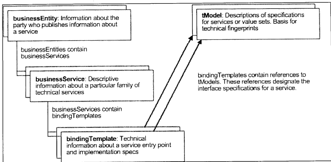
Figure 2.1: UDDI's core data types [42]
