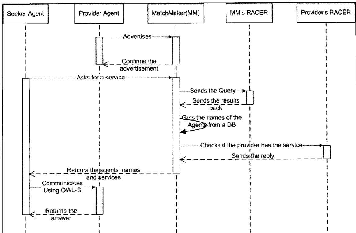
Figure 5.3: Sequence diagram illustrating the agent communication
