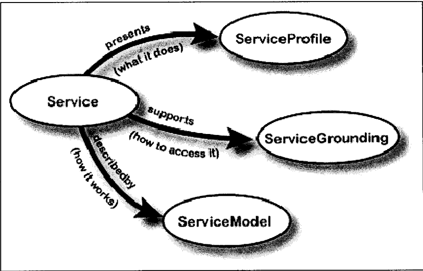
Figure 3.6: Top level of the service ontology [25]
