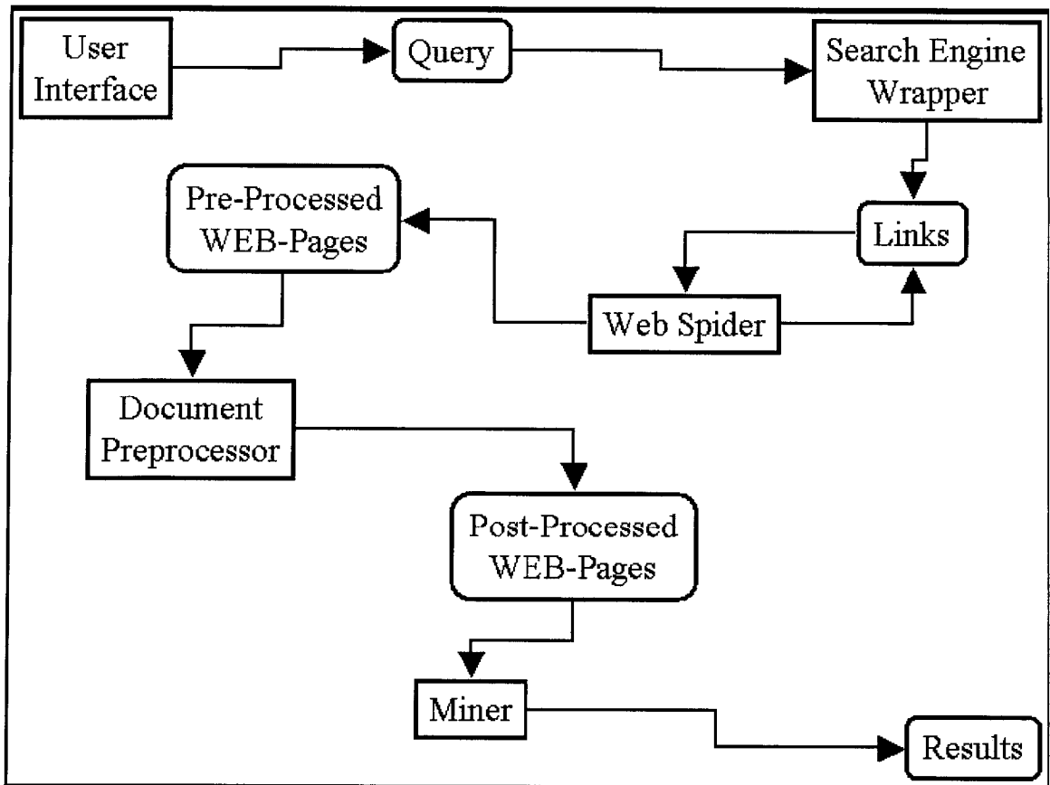
Figure 7.4: High level system architecture [39].
