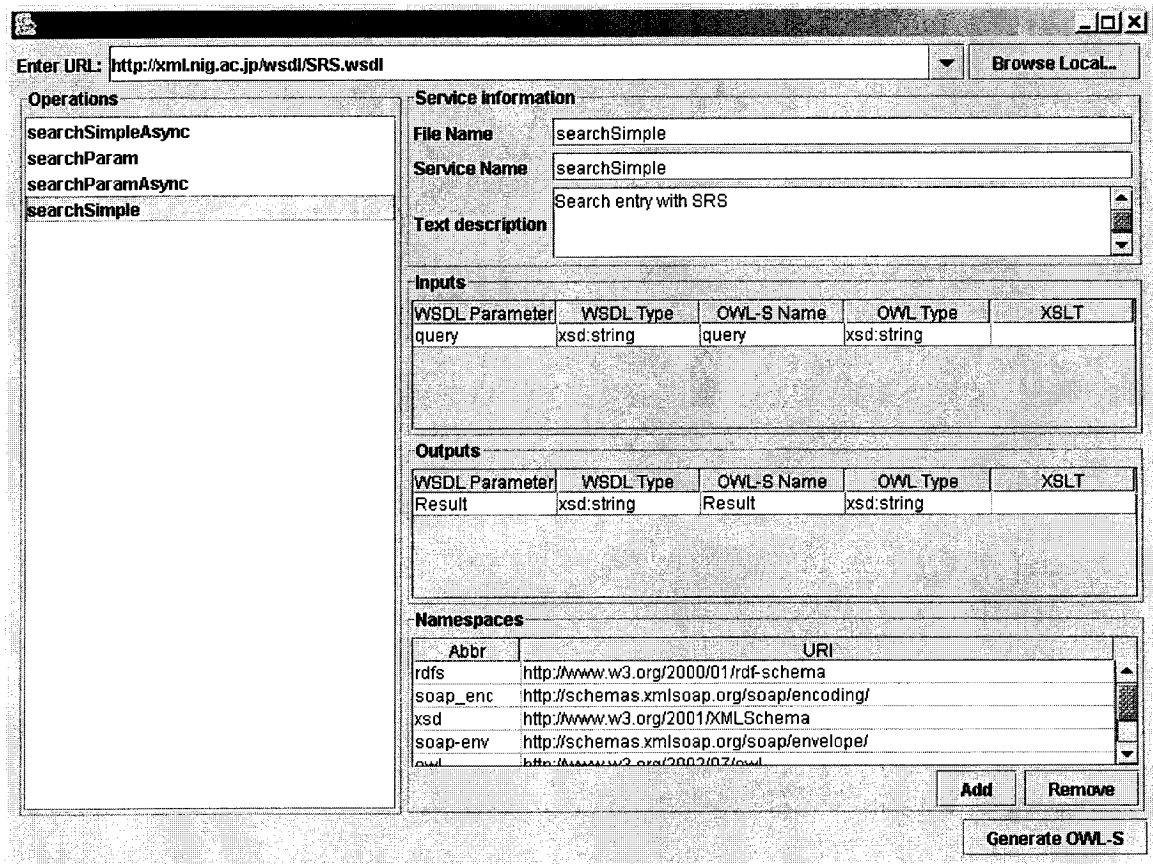
Figure B.3. OWL-S API Tool
