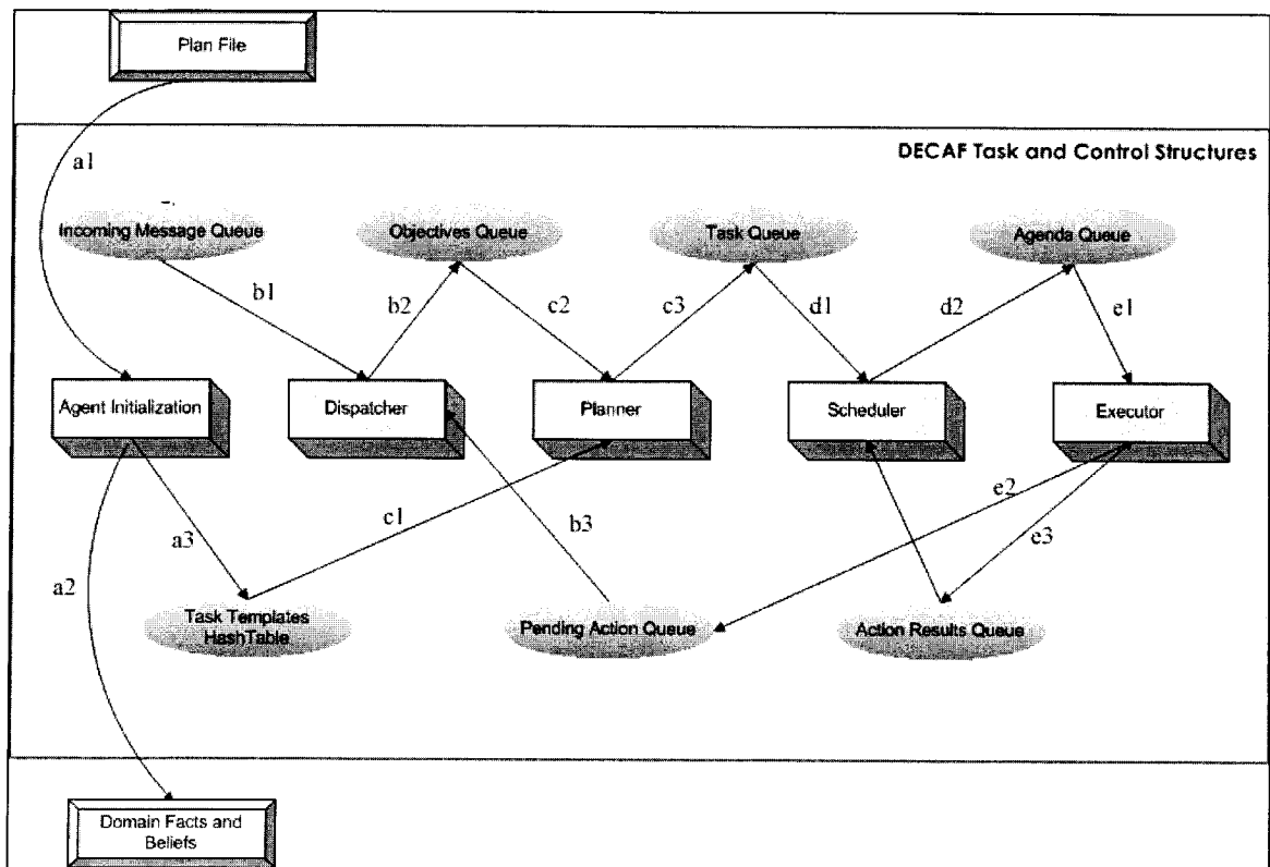
Figure 3.7: DECAF architecture view
