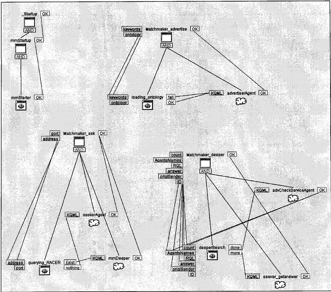
Figure 5.5: Plan file of the Matchmaker
