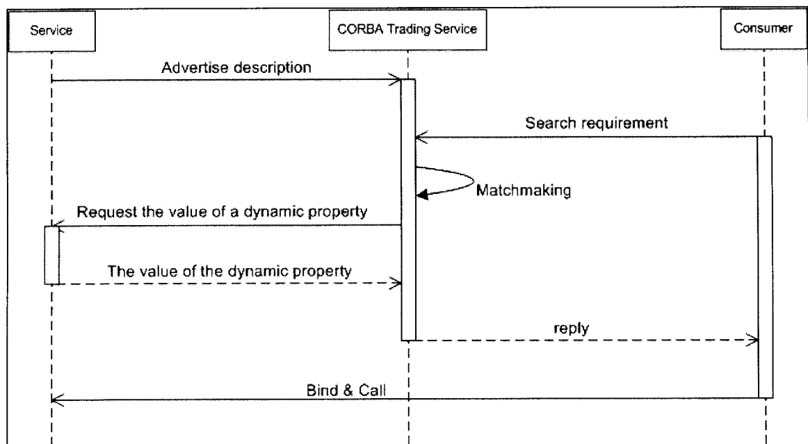
Figure 2.2: Sequence diagram of CORBA matchmaking
