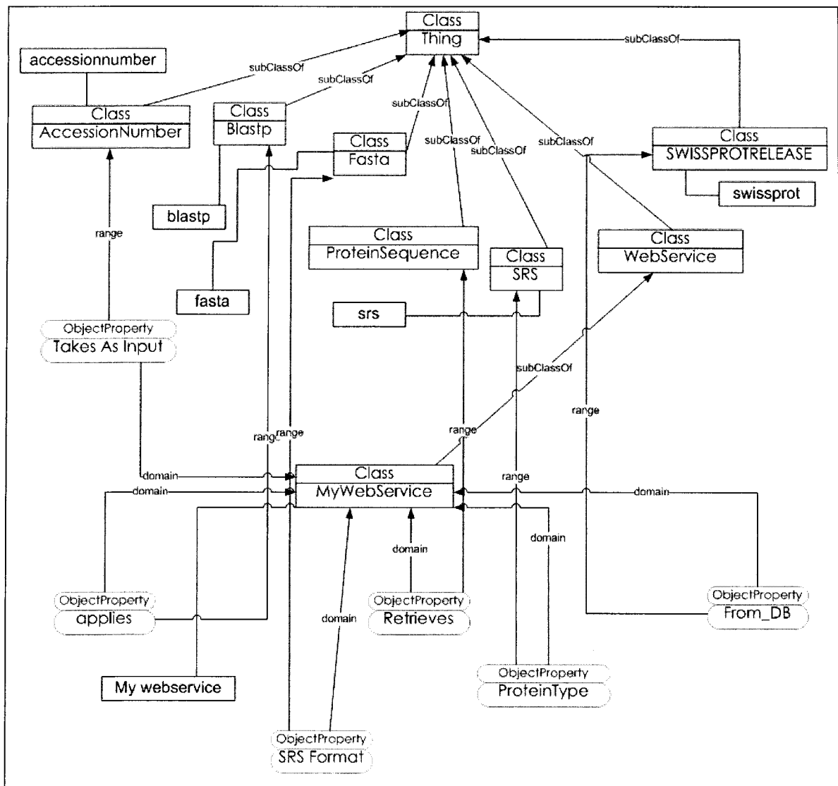
Figure B.2. The provider agent's ontology.
