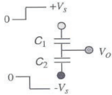
Fig. 7. 13: Equivalent electrical circuit of the accelerometer
