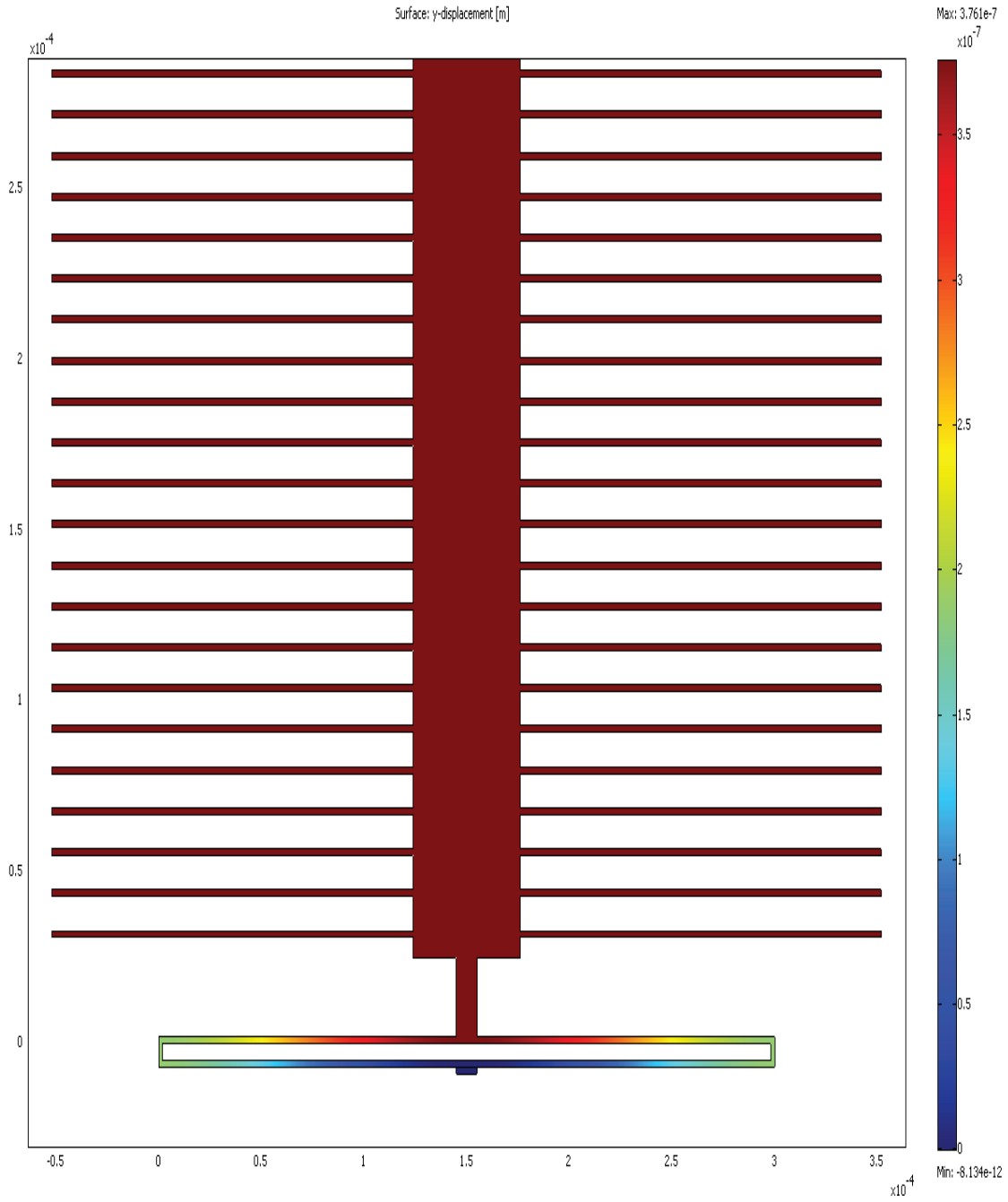
Fig. 7. 11: Expanded view of the spring deflection under 150 g force
