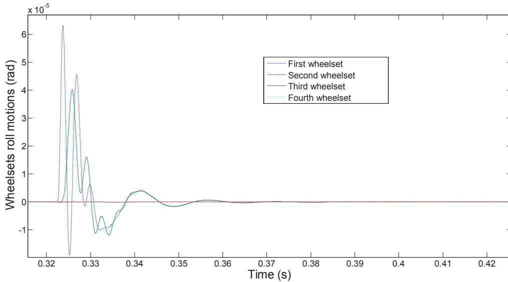
Fig. 4. 11: Time histories of all four wheelsets roll motions with left wheel flat in first wheelset
