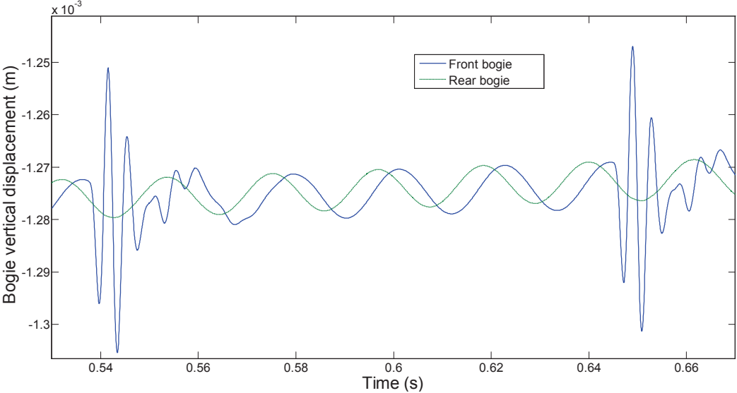
Fig. 4. 12: Time histories of bogie vertical displacement response with left wheel flat in first wheelset ( v = 100 km/h; L_f = 50 mm; D_f = 0.35 mm).
