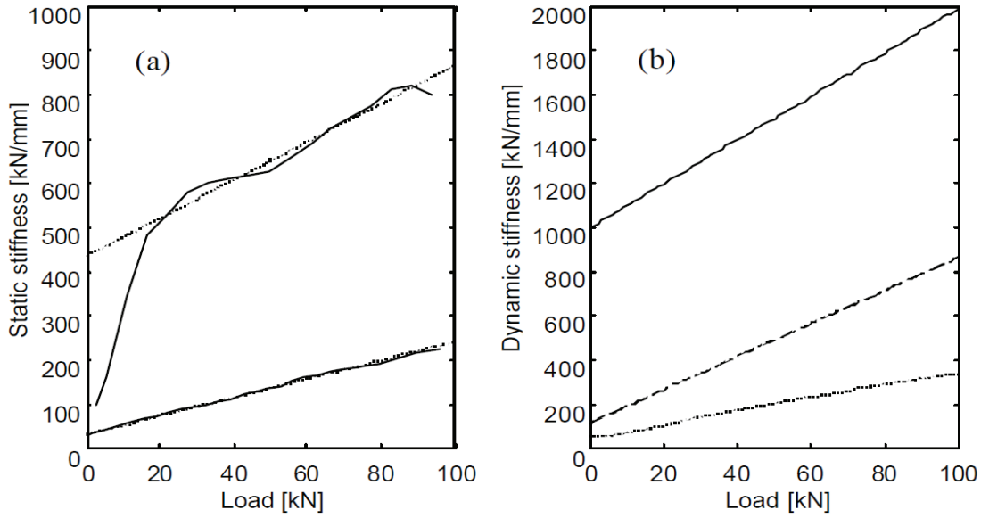
Fig. 1. 19: (a) static stiffness of non-linear pads, — measured , ···· approximated. The upper curves are for the stiff pad and the lower curves are for the medium pad; (b) dynamic stiffness of non-linear pads, — stiff pad, --- medium pad, ···· soft pad [105].
