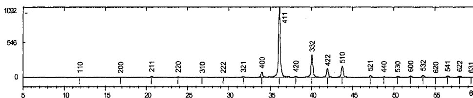
Figure A-21: Calculated XRD diffraction pattern for \gamma .
