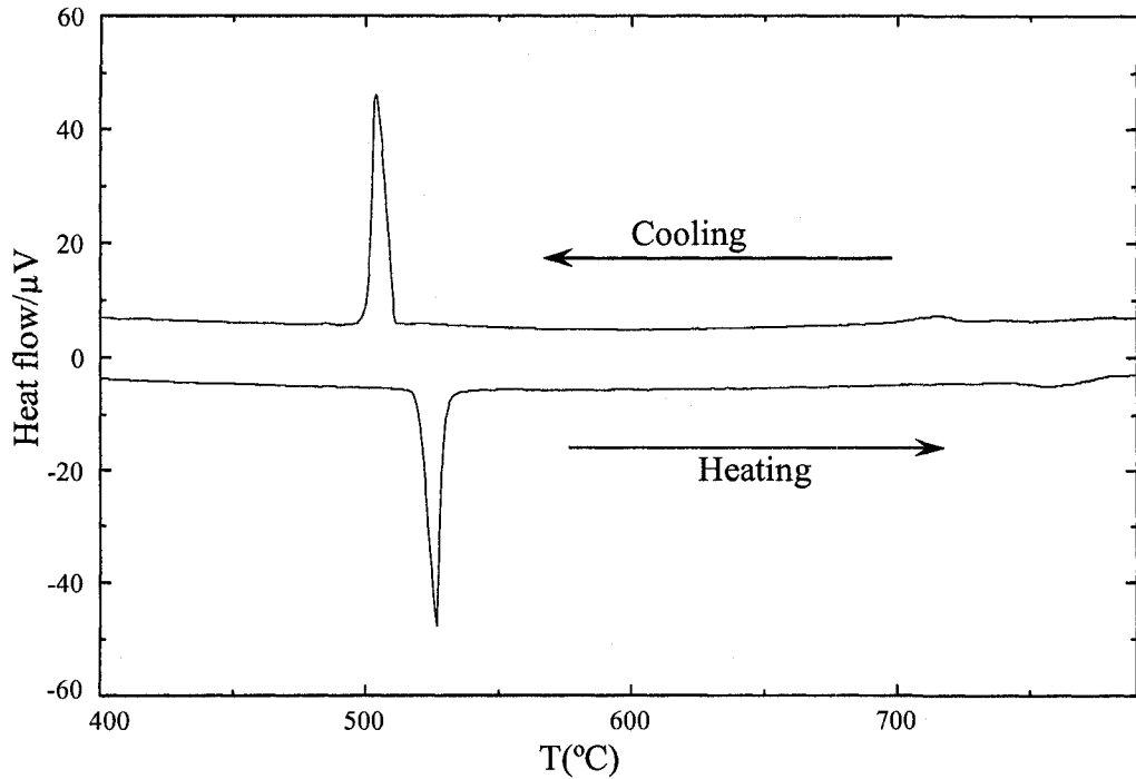
Figure 7.29: DSC spectra of sample 9 (43.9/26.7/29.4 wt.% Mg/Al/Ca) during heating and cooling.
