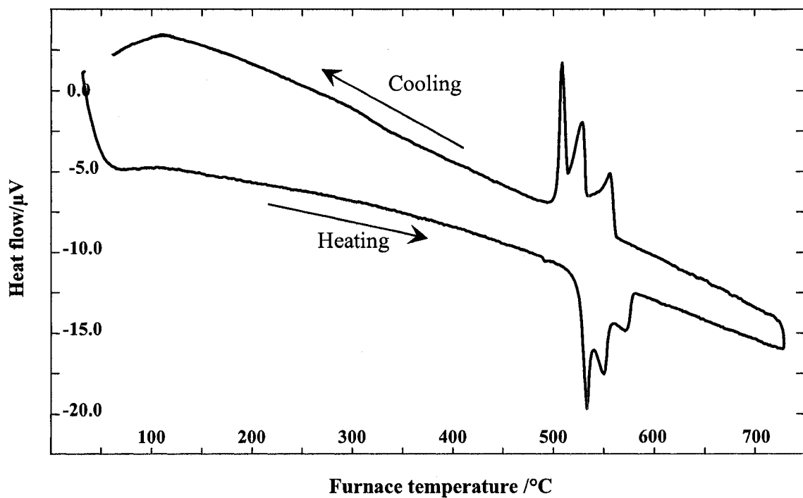
Figure 6.42: DSC spectra of sample 23 (78/12.4/9.6, Mg/Al/Sr) during heating and cooling.
