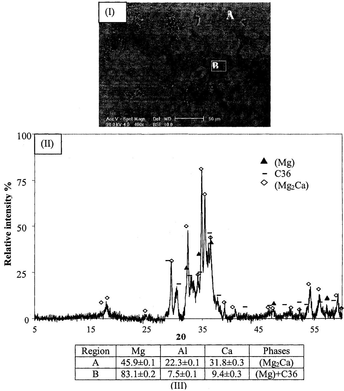
Figure 7.4: (I) SEM image; (II) XRD pattern and (III) EPMA analysis of composition I.
