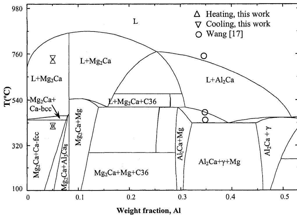
Figure 7.14: Calculated vertical section at 47 wt.% Mg with DSC signals from heating and cooling curves of sample 4.
