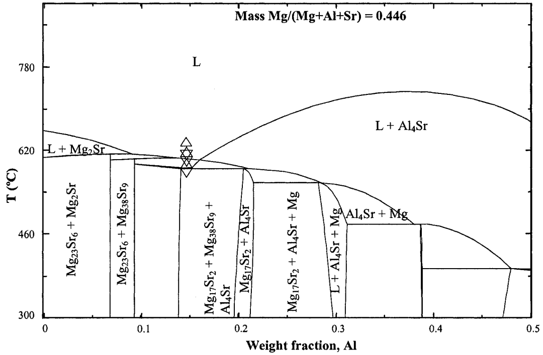
Figure 6.23: Calculated vertical section at 44.6 wt.% Mg with DSC signals from heating and cooling curves of sample 17.
