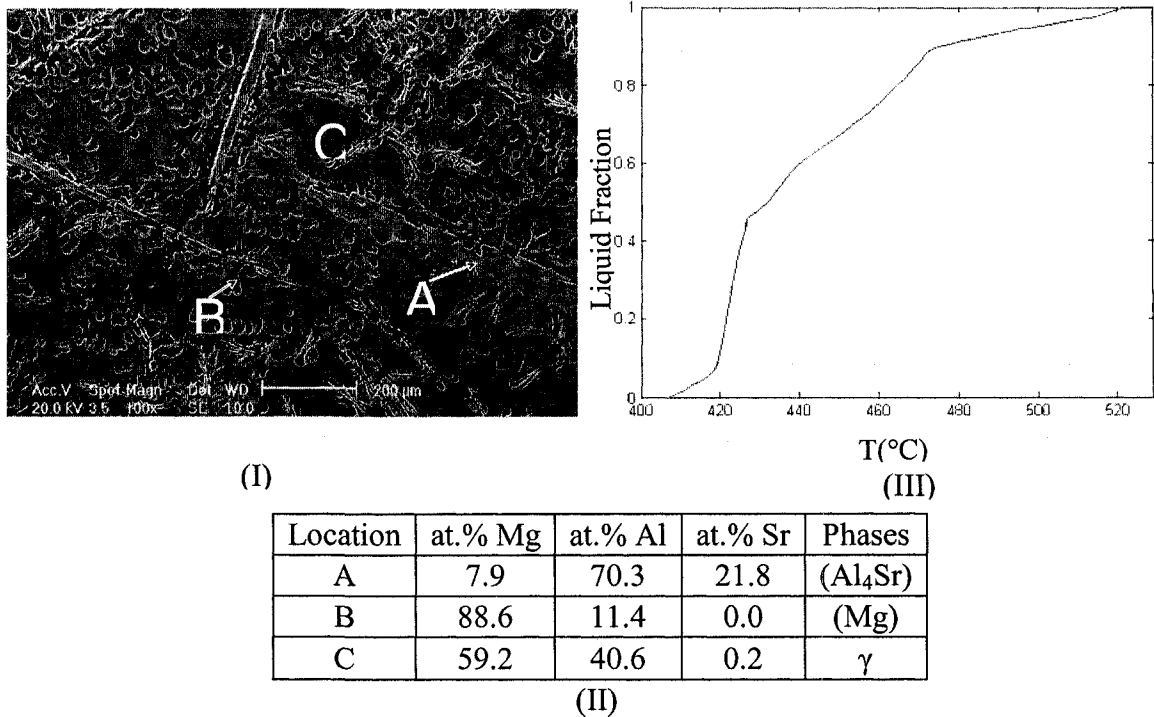
Figure 6.4: (I) SEM image; (II) EPMA analysis and (III) Solidification curve of composition 3.
