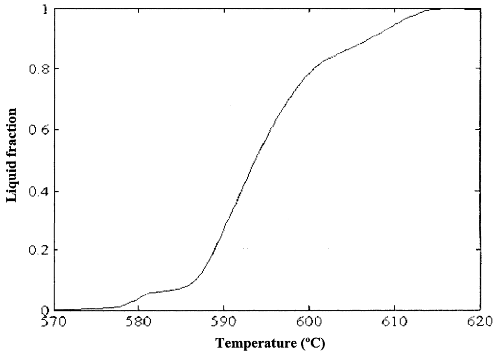
Figure 6.24: Solidification curve of sample 17.
