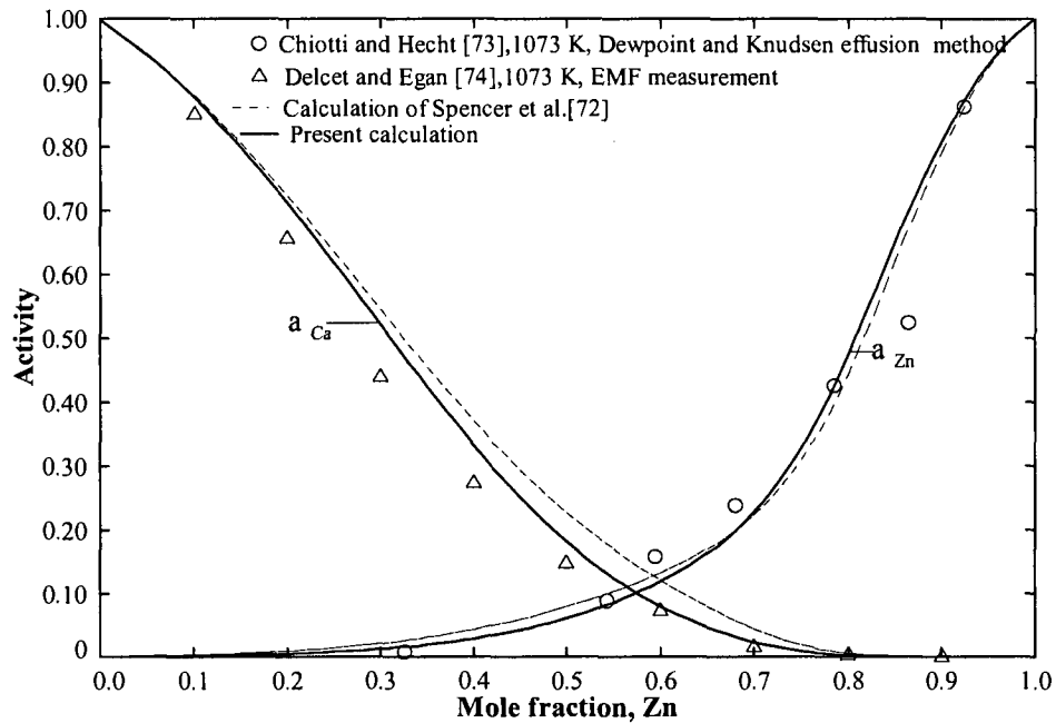
Figure 4.11: Calculated activities of Ca and Zn in the Ca-Zn liquid at 1073 K
