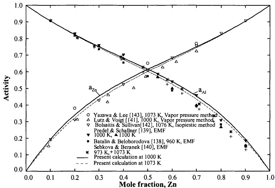
Figure 4.25: Calculated activity of Al and Zn in the liquid state at 1000 K and 1073K
