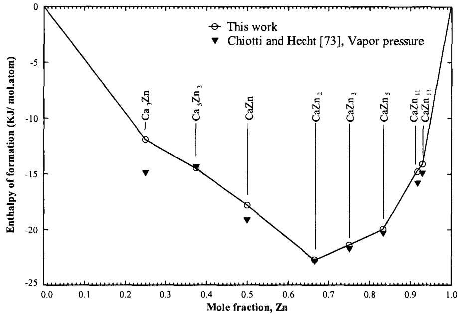
Figure 4.12: Calculated heat of formation for the intermediate phases at 298.15 K with the experimental data
