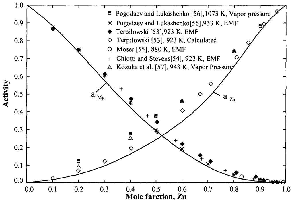
Figure 4.5: Calculated activity of Mg and Zn (relative to pure liquid Mg and Zn) in Mg-Zn alloys at 923 K and 1073 K, respectively
