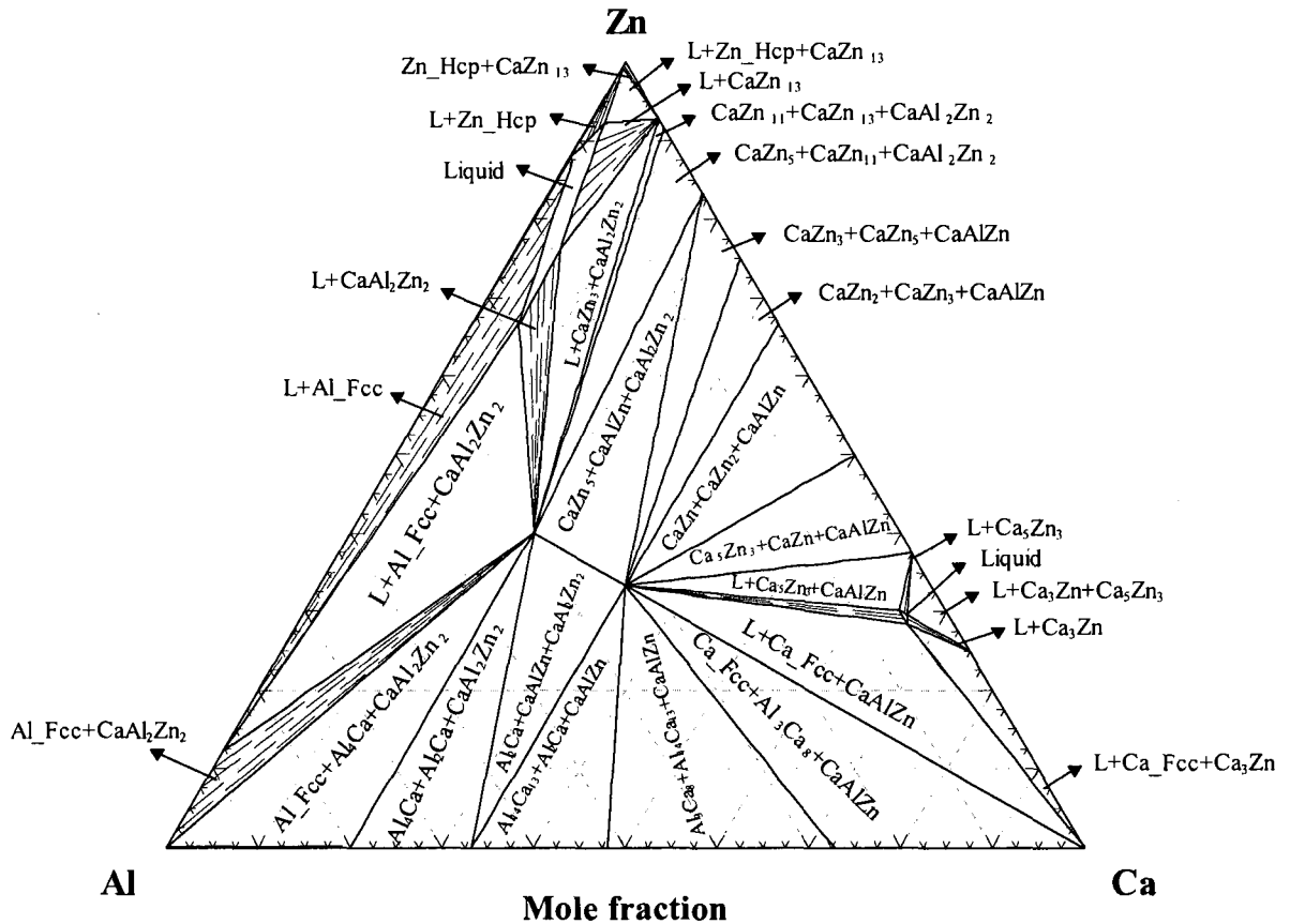
Figure 4.37: Calculated isothermal section of the Al-Ca-Zn system at 650 K with two ternary compounds where A denotes: \text{CaAlZn} and B denotes: \text{CaAl}_2\text{Zn}_2
