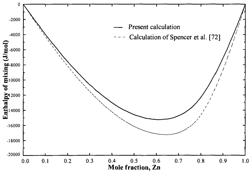
Figure 4.13: Calculated enthalpy of mixing in the Ca-Zn liquid at 1173 K
