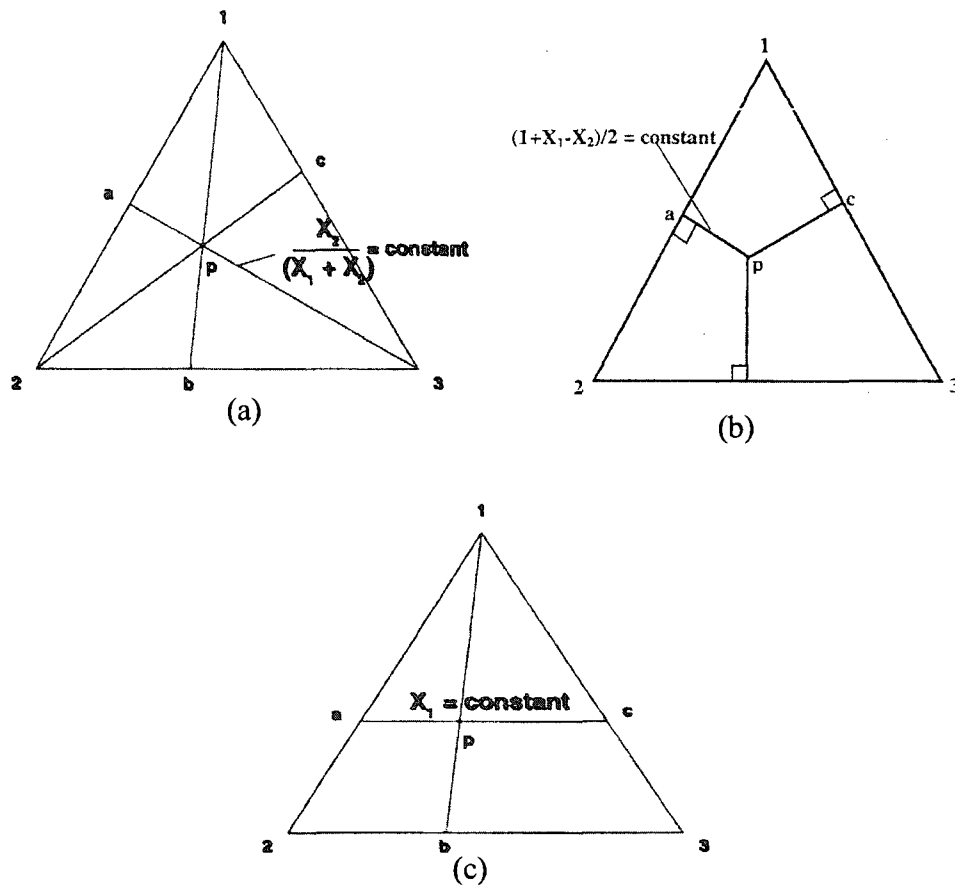
Figure 3.2: Different “geometric” models for ternary extrapolation: (a) Kohler (b) Muggianu and (c) Toop [166]
