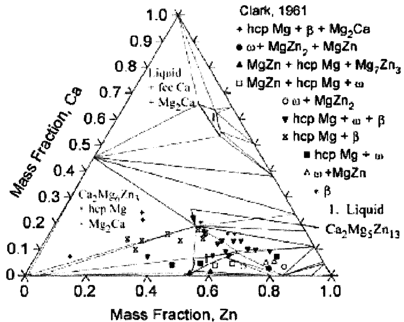
Figure 2.15: The calculated isothermal section at 608 K of the Mg-Ca-Zn ternary system with experimental result form literature [100]
