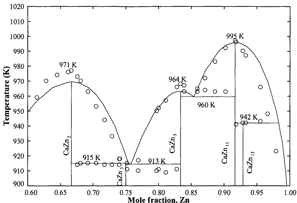
Figure 4.10: Enlarged portion of the Ca-Zn phase diagram (Zn-rich side)
