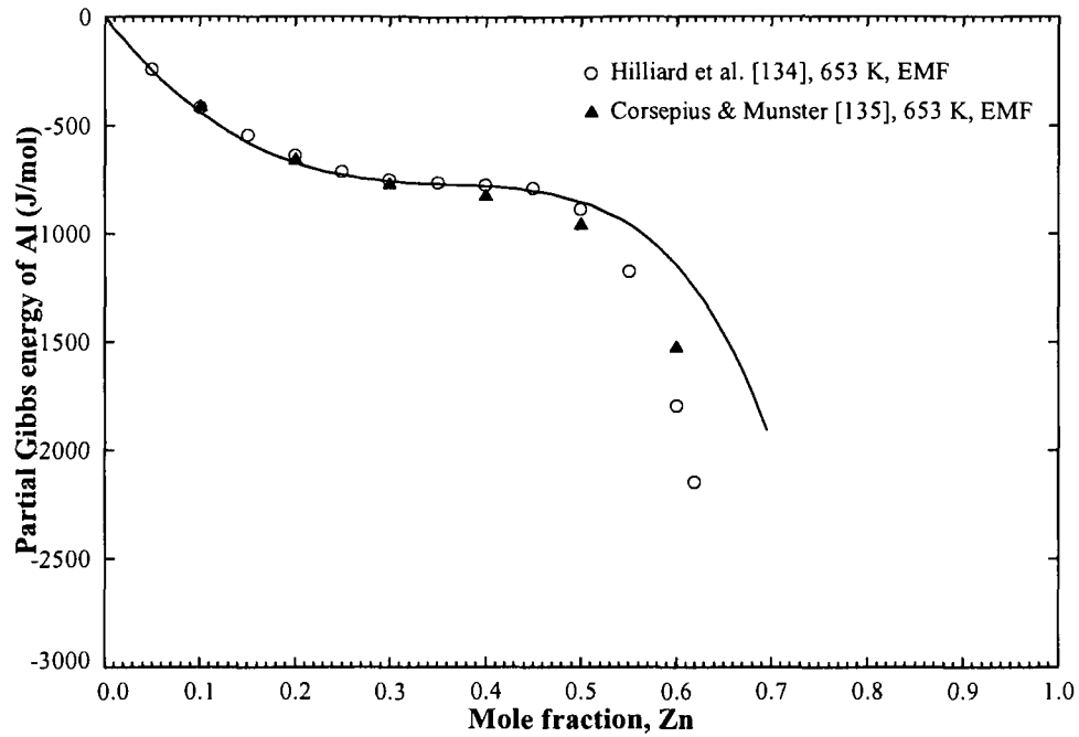
Figure 4.28: Calculated partial Gibbs energy of Al in the fcc phase at 653 K
