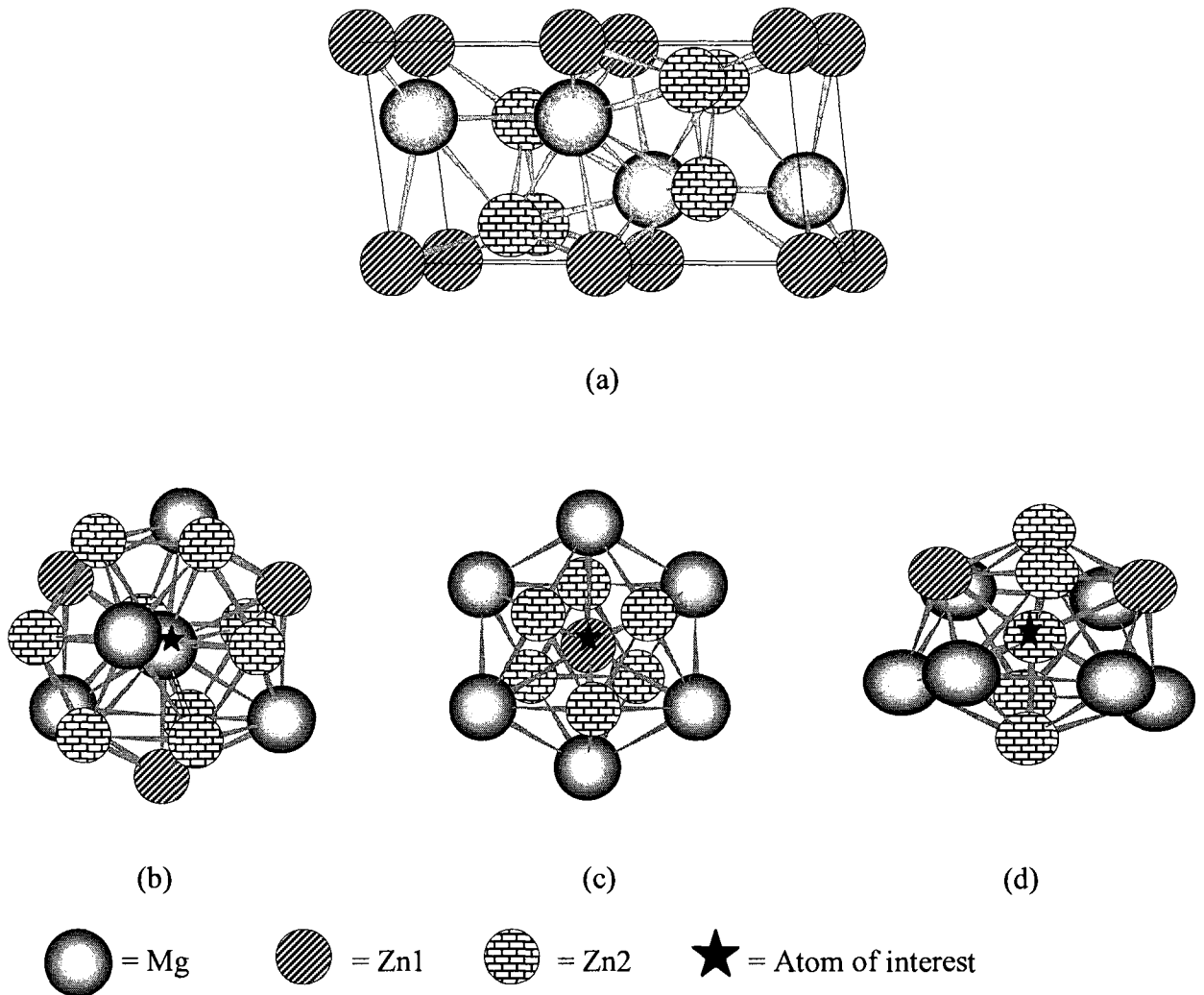
Figure 4.3: (a) Unit cell of MgZn_2 , Substructure of (b) Mg atom with CN=16 , (c) Zn1 atom with CN=12 and (d) Zn2 atom with CN=12
