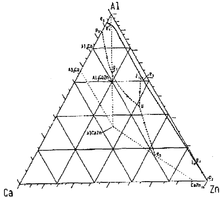
Figure 2.23: A tentative Al-Ca-Zn liquidus projection [154]
