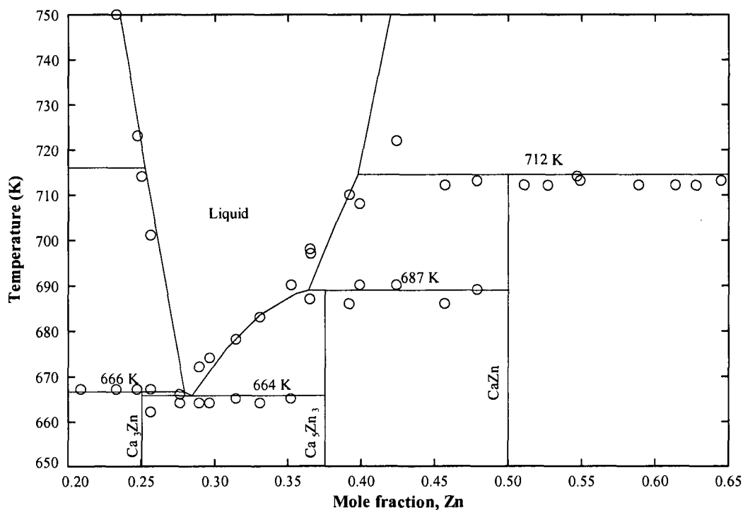
Figure 4.9: Enlarged portion of the Ca-Zn phase diagram (Ca-rich side)
