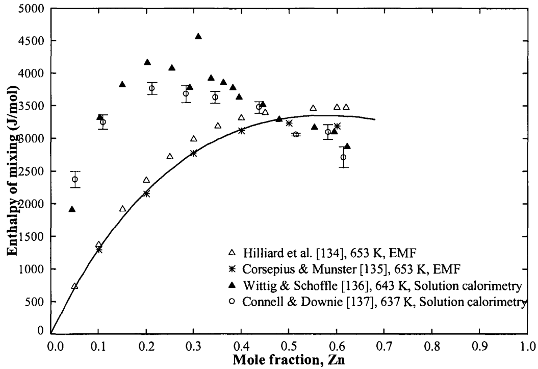
Figure 4.26: Calculated enthalpies of mixing in the Al fcc solid solution at 653 K in comparison with the experimental results
