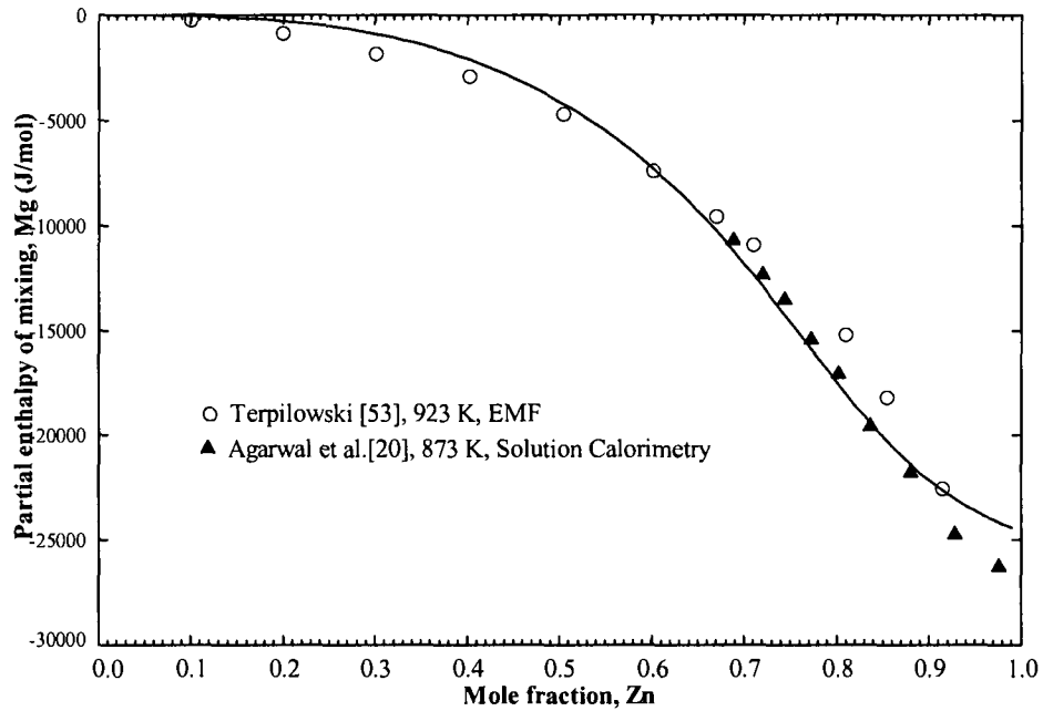
Figure 4.6: Calculated partial enthalpy of mixing of Mg in the Mg-Zn liquid at 923 K
