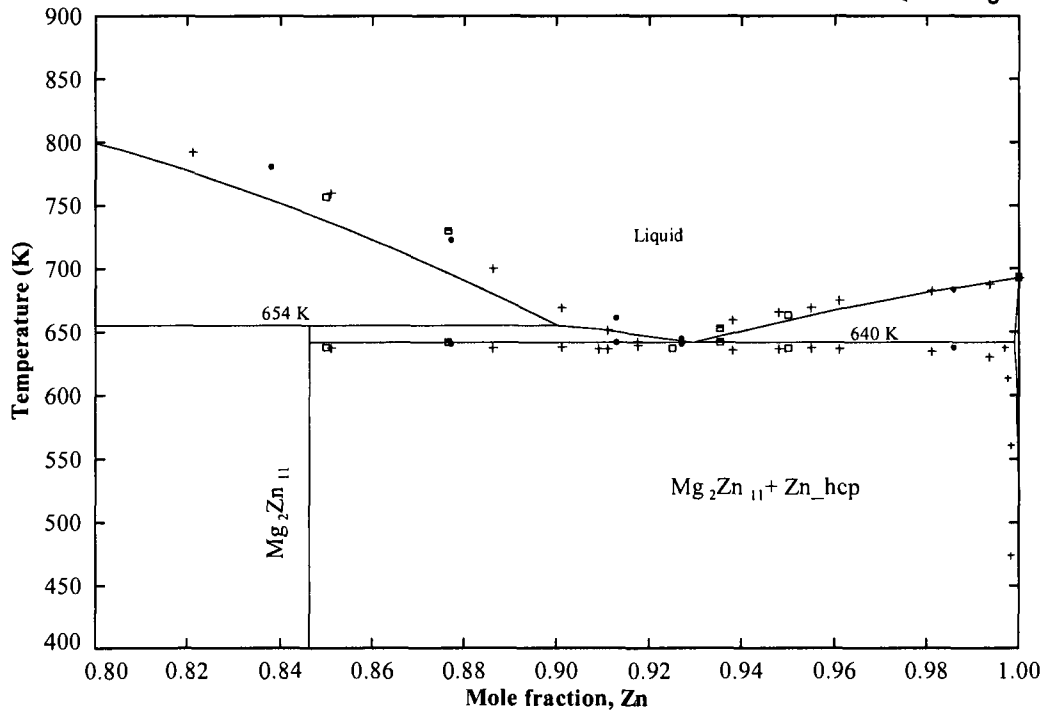
Figure 4.2: Calculated Zn-rich side of the Mg-Zn phase diagram with experimental results from literature
