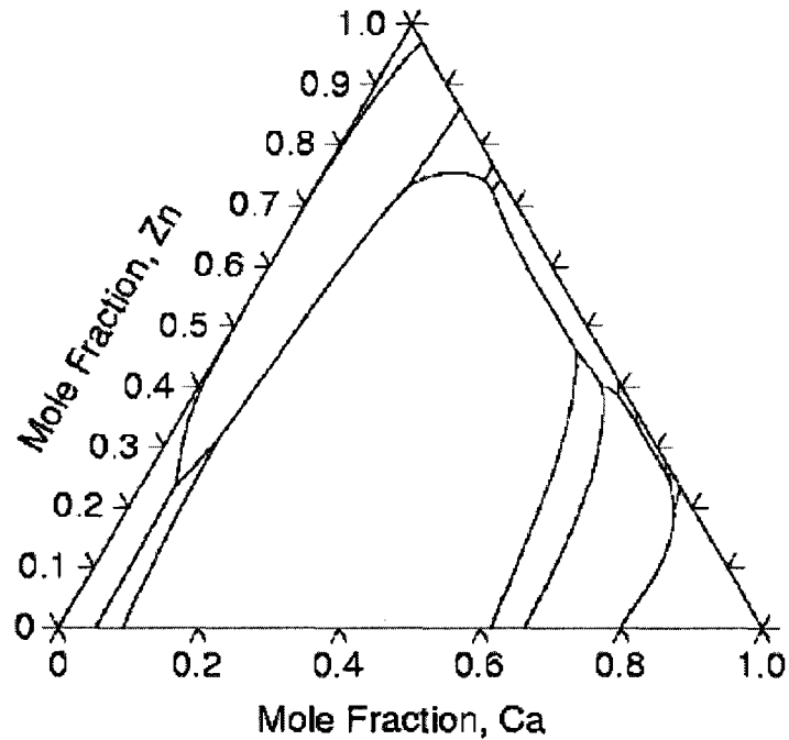
Figure 2.24: Liquidus projection of the Al-Ca-Zn system [157]
