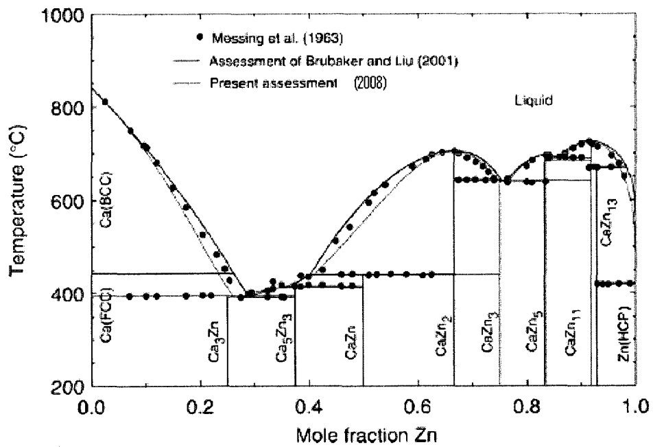
Figure 2.5: Calculated Ca-Zn phase diagram [72]
