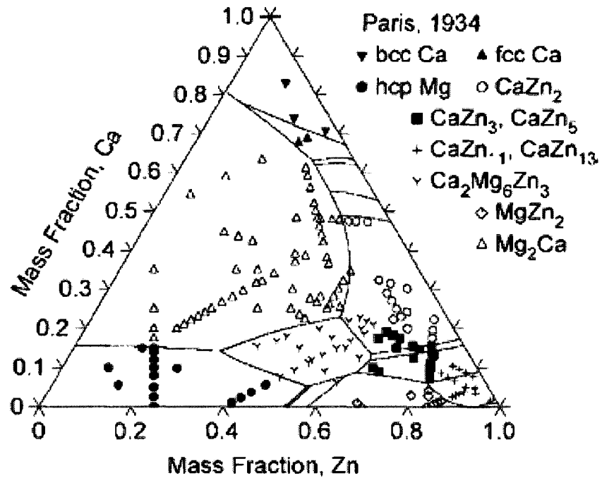
Figure 2.14: The calculated liquidus projection of the Mg-Ca-Zn ternary system with experimental result form literature [100]
