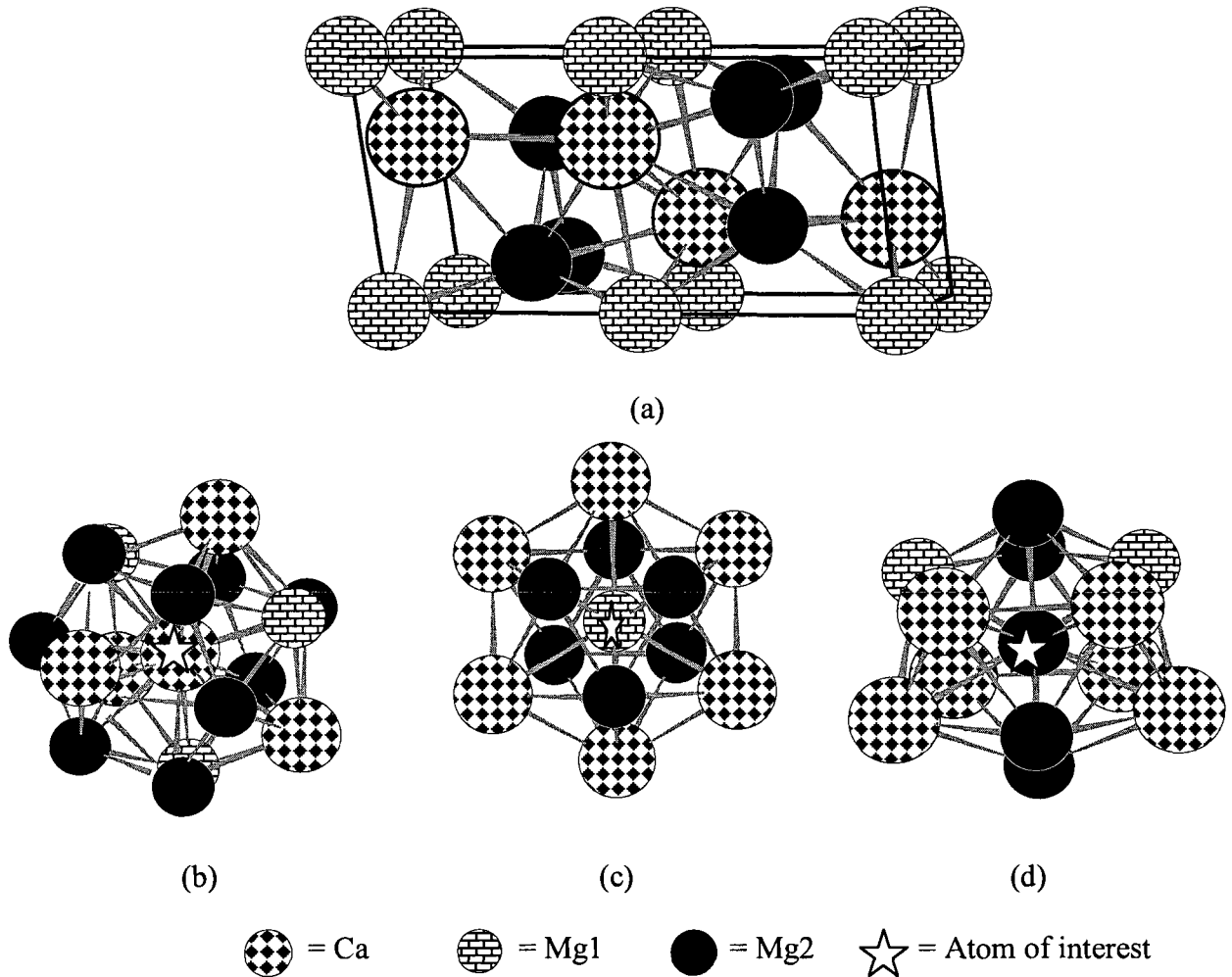
Figure 4.15: (a) Unit cell of Mg 2 Ca, Substructure of (b) Ca atom with CN=16, (c) Mg1 atom with CN=12 and (d) Mg2 atom with CN=12
