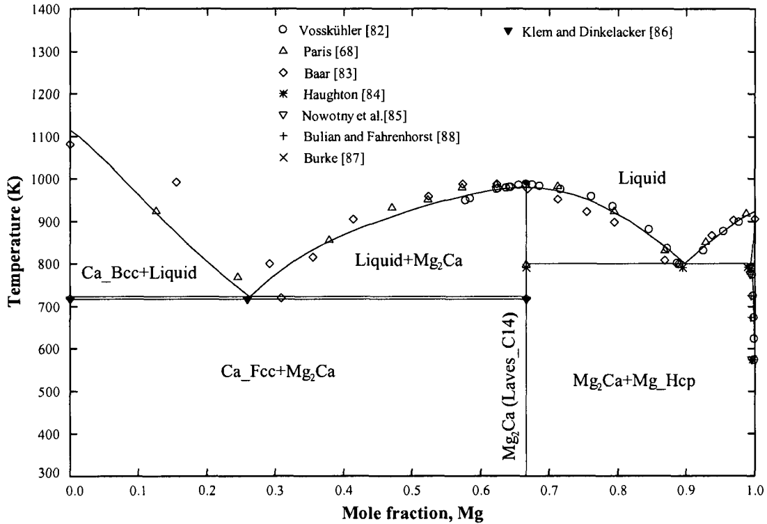
Figure 4.14: Calculated Mg-Ca phase diagram in comparison with experimental results from literature
