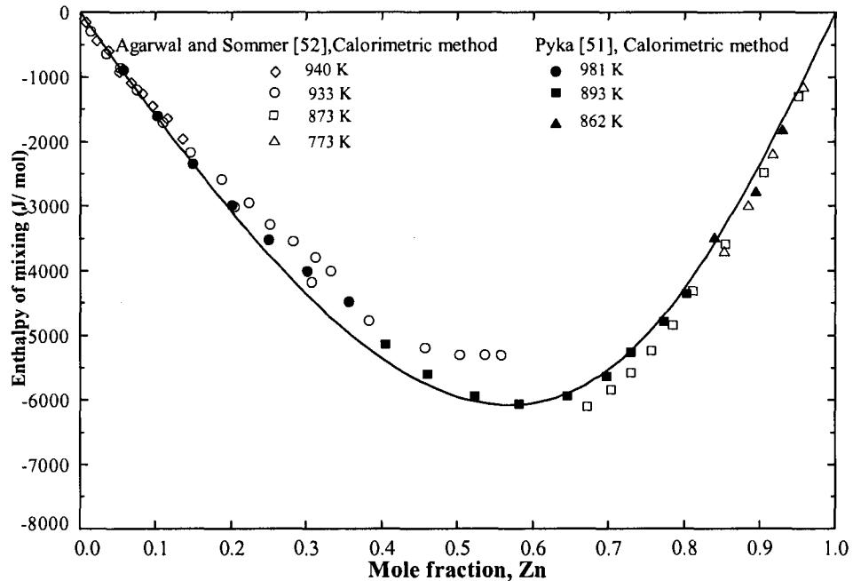
Figure 4.4: Calculated enthalpy of mixing of Mg-Zn liquid at 981 K
