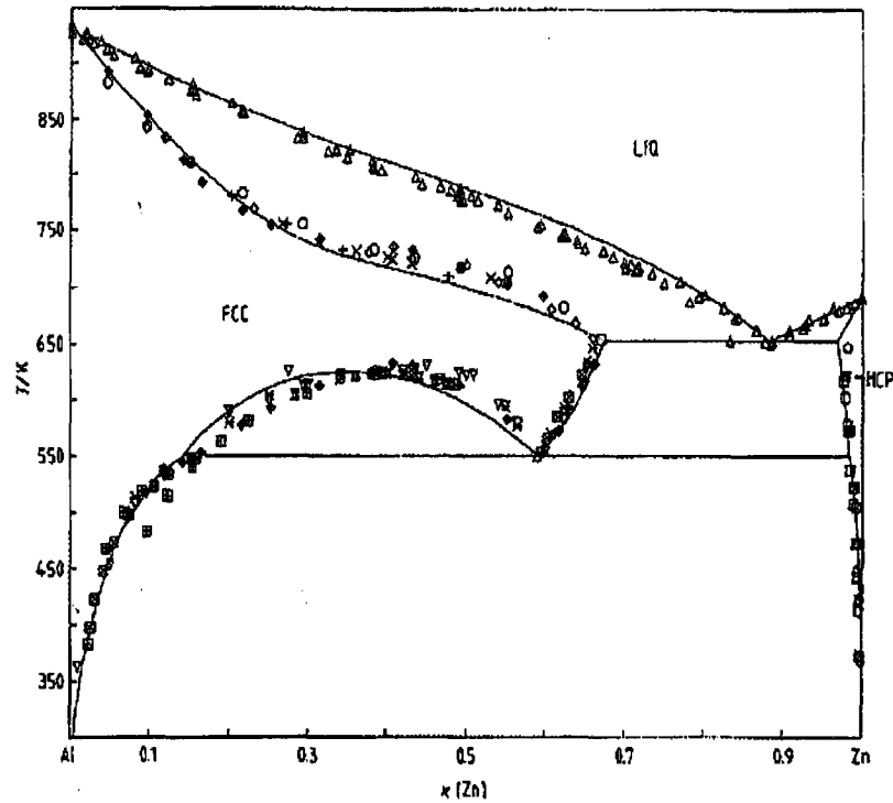
Figure 2.16: Calculated Al-Zn phase diagram [130]
