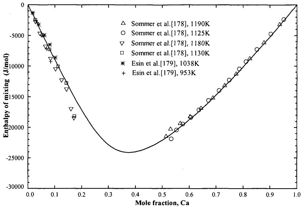
Figure 4.31: Calculated enthalpies of mixing of Al and Ca in liquid Al-Ca alloy at 1100 K in comparison with the experimental results
