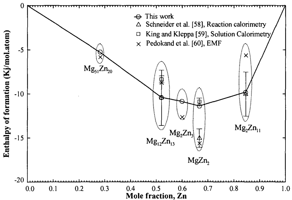
Figure 4.7: Calculated enthalpy of formation for the intermediate phases of the Mg-Zn system at 298.15 K
