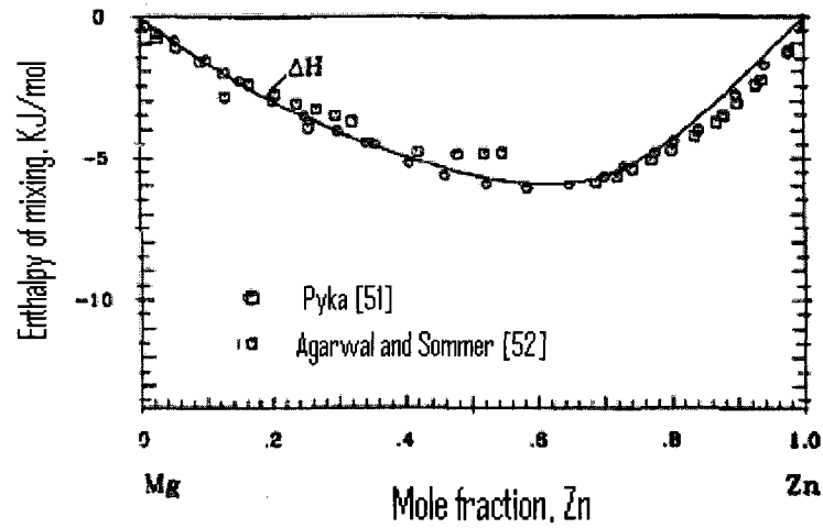
Figure 2.2: Calculated enthalpy of mixing for liquid phase in Mg-Zn system at 981K with the experimental data [6]
