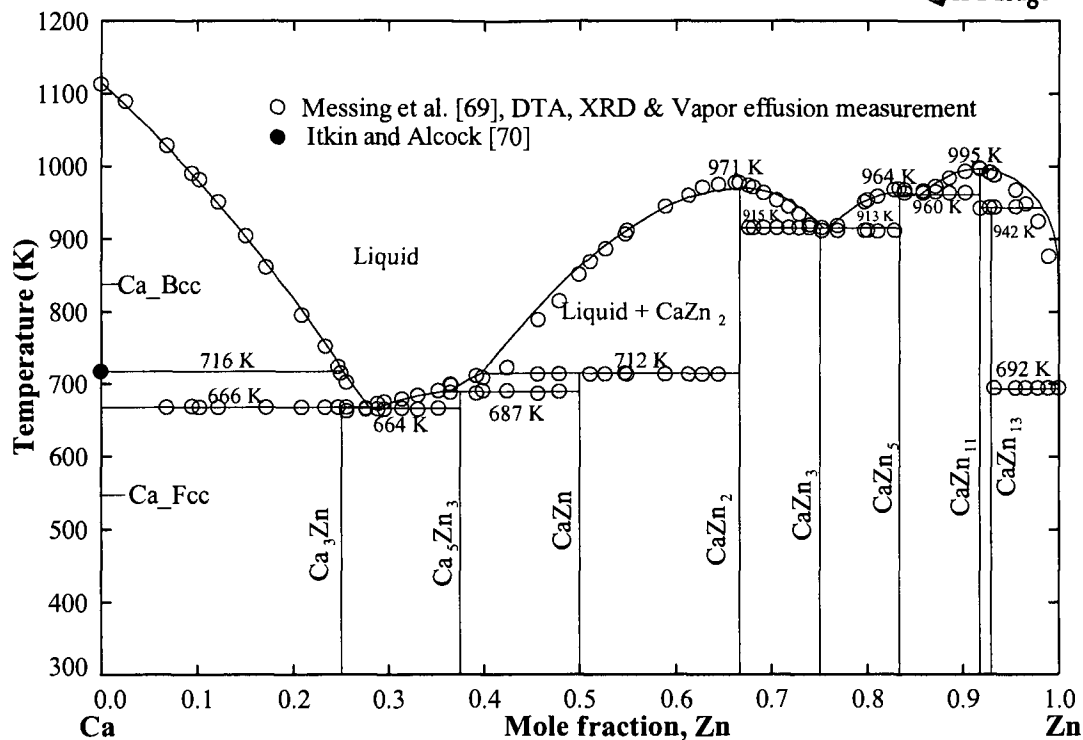
Figure 4.8: Calculated Ca-Zn phase diagram in comparison with experimental results from the literature
