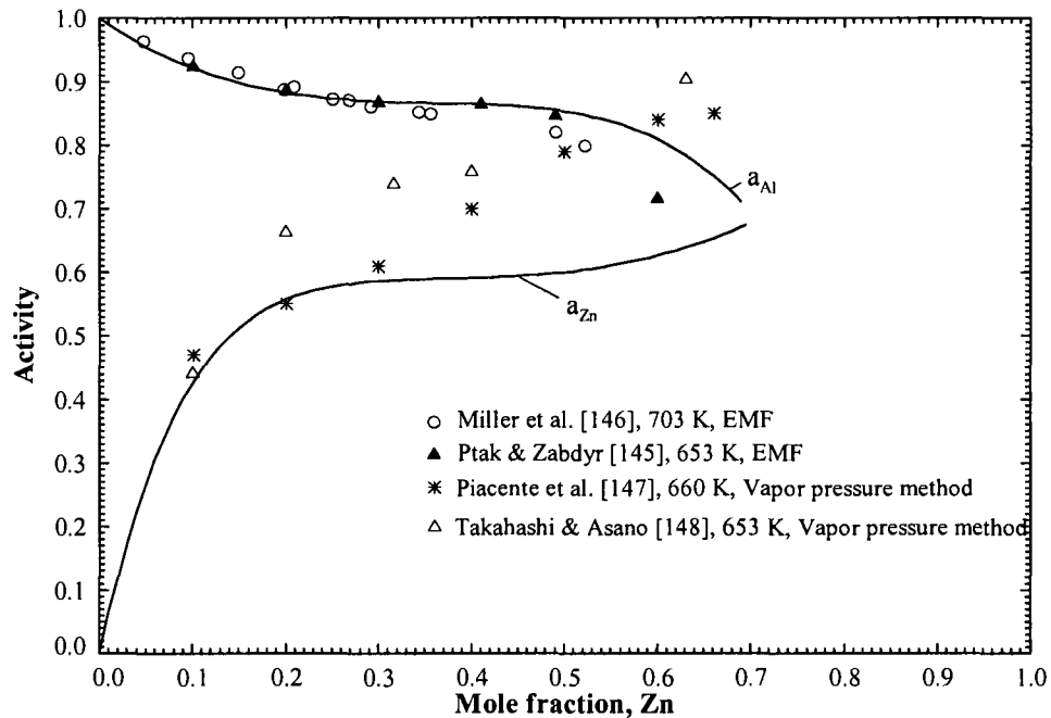
Figure 4.27: Calculated activity of Al and Zn in the fcc phase at 653 K
