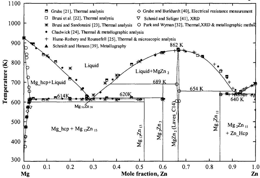
Figure 4.1: Calculated Mg-Zn phase diagram in comparison with the experimental results from the literature
