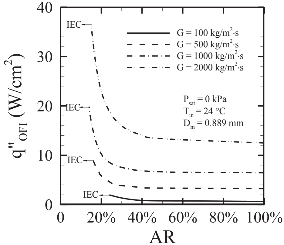
Figure 6.12: Effect of area ratio on the onset of flow instability.
