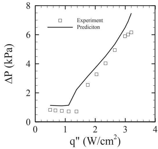
(a) G = 160 \text{ kg/m}^2\cdot\text{s}
