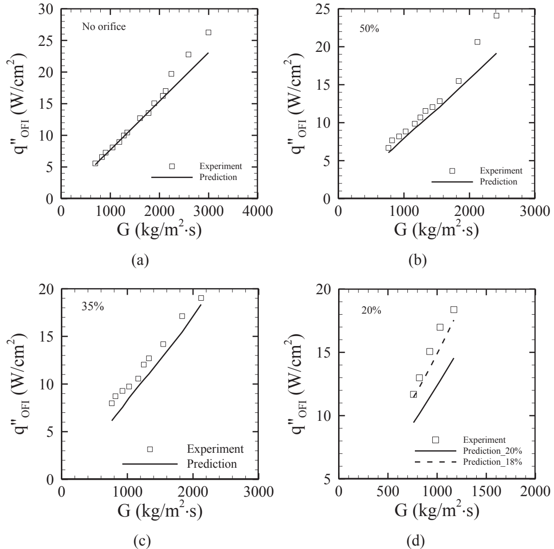
Figure 6.9: The predicted and measured onset of flow instability in the microtubes with and without orifices.
