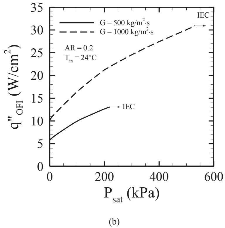
Figure 6.14: Effect of saturation pressure on the onset of flow instability.
