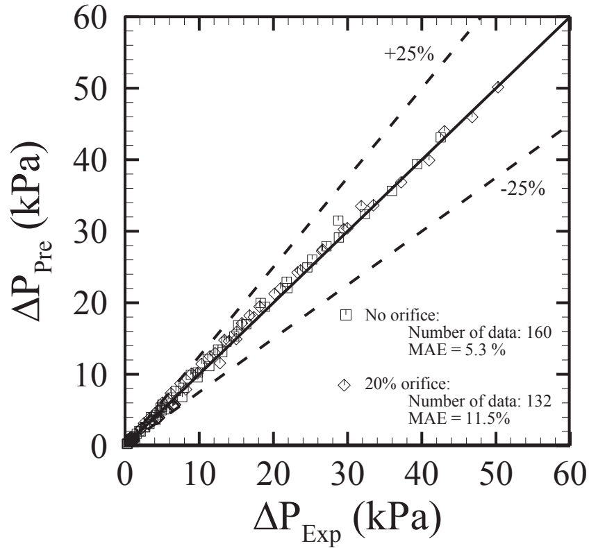
Figure 6.8: Comparisons of pressure drop between the prediction and experiment at four mass fluxes.
