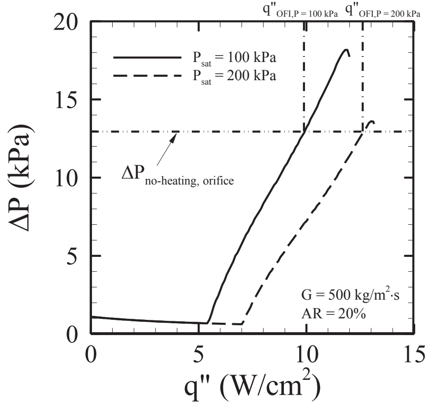
Figure 6.13: Pressure drop at G = 500 \text{ kg/m}^2\cdot\text{s} under two saturation pressures.
