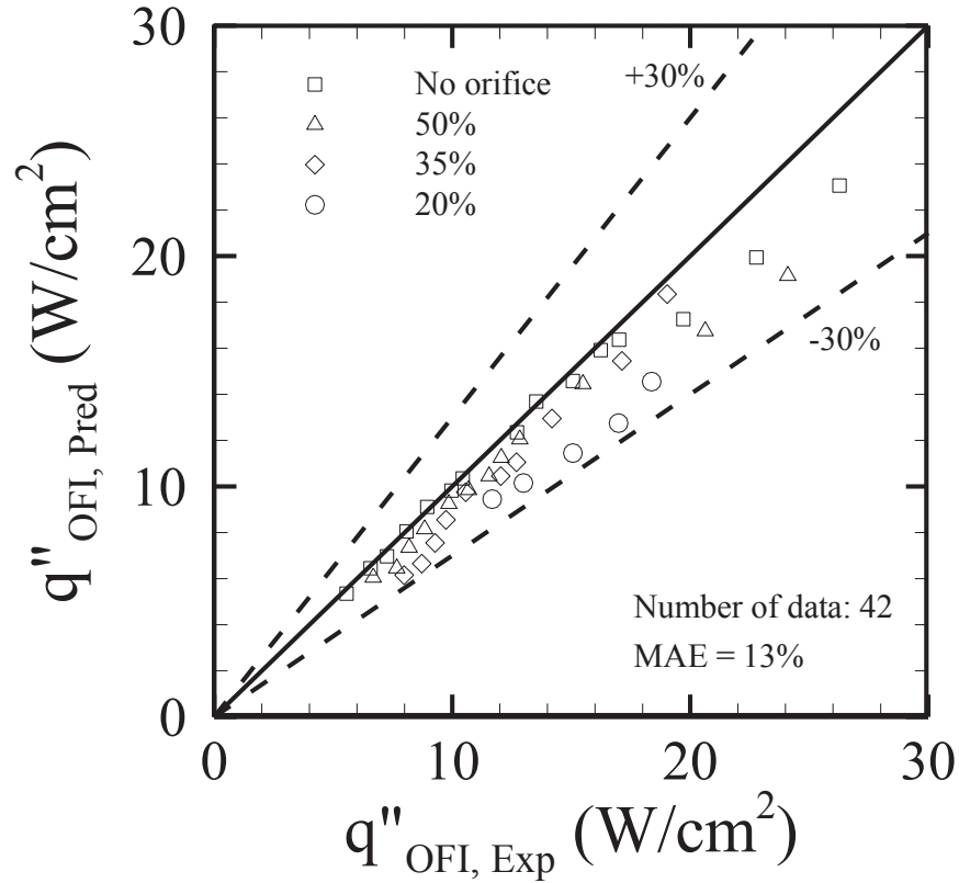
Figure 6.11: Comparison of the onset of flow instability between the experiment and prediction.
