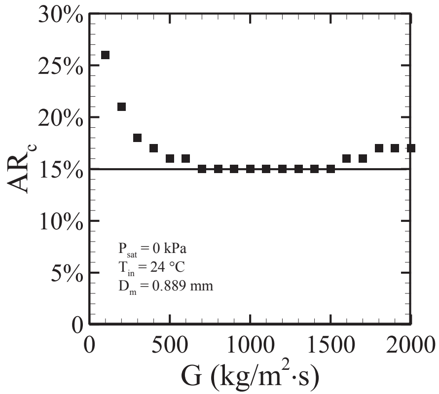
Figure 6.15: Critical area ratio at mass fluxes from 100 to 2000 kg/m 2 ·s.
