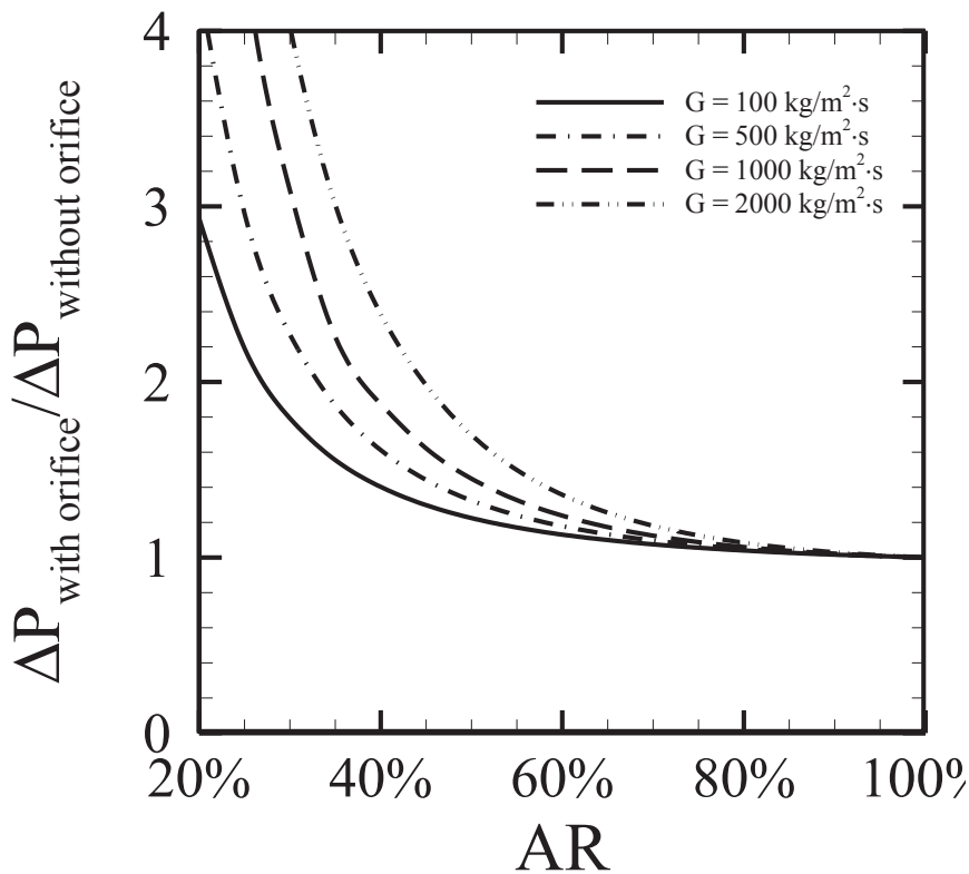
Figure 6.10: Pressure drop ratio in the microtube with and without an inlet orifice under no heating condition
