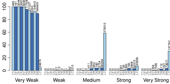
Fig. 5. FedEx checker password strength distribution
