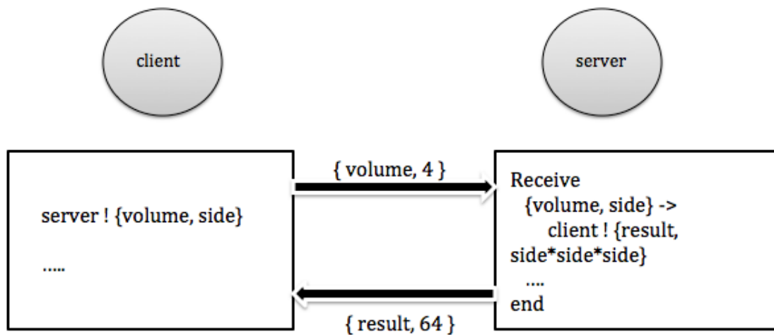
Figure 2.2: Erlang Communication between processes
