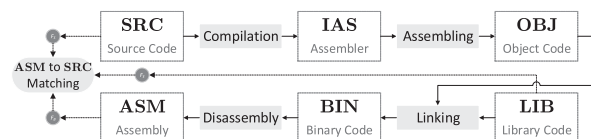
Fig. 3. Compilation steps.
