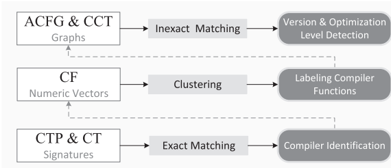
Fig. 1. BinComp architecture.
