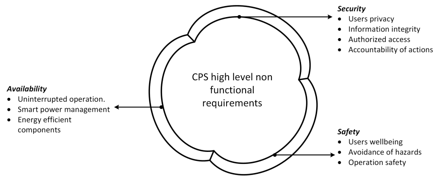
Fig. 3. High level properties of cyber physical systems
