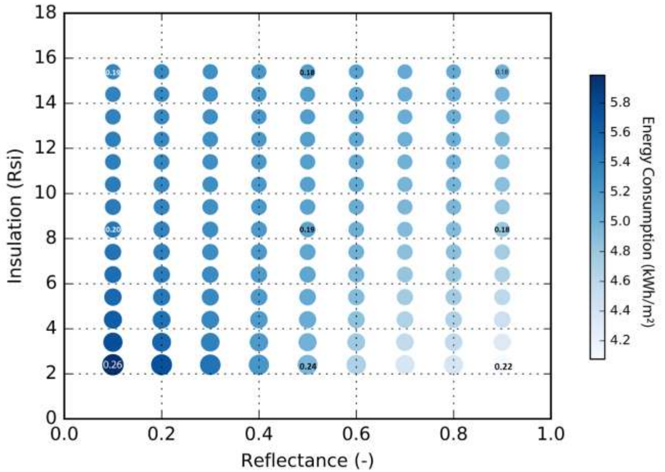
Figure 4 – Mean and variance of cooling energy use for all design combinations for 2018-2037
