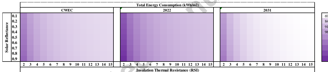
Figure 3 – Total energy consumption heat maps for CWEC and extreme future years 2022 and 2031.
