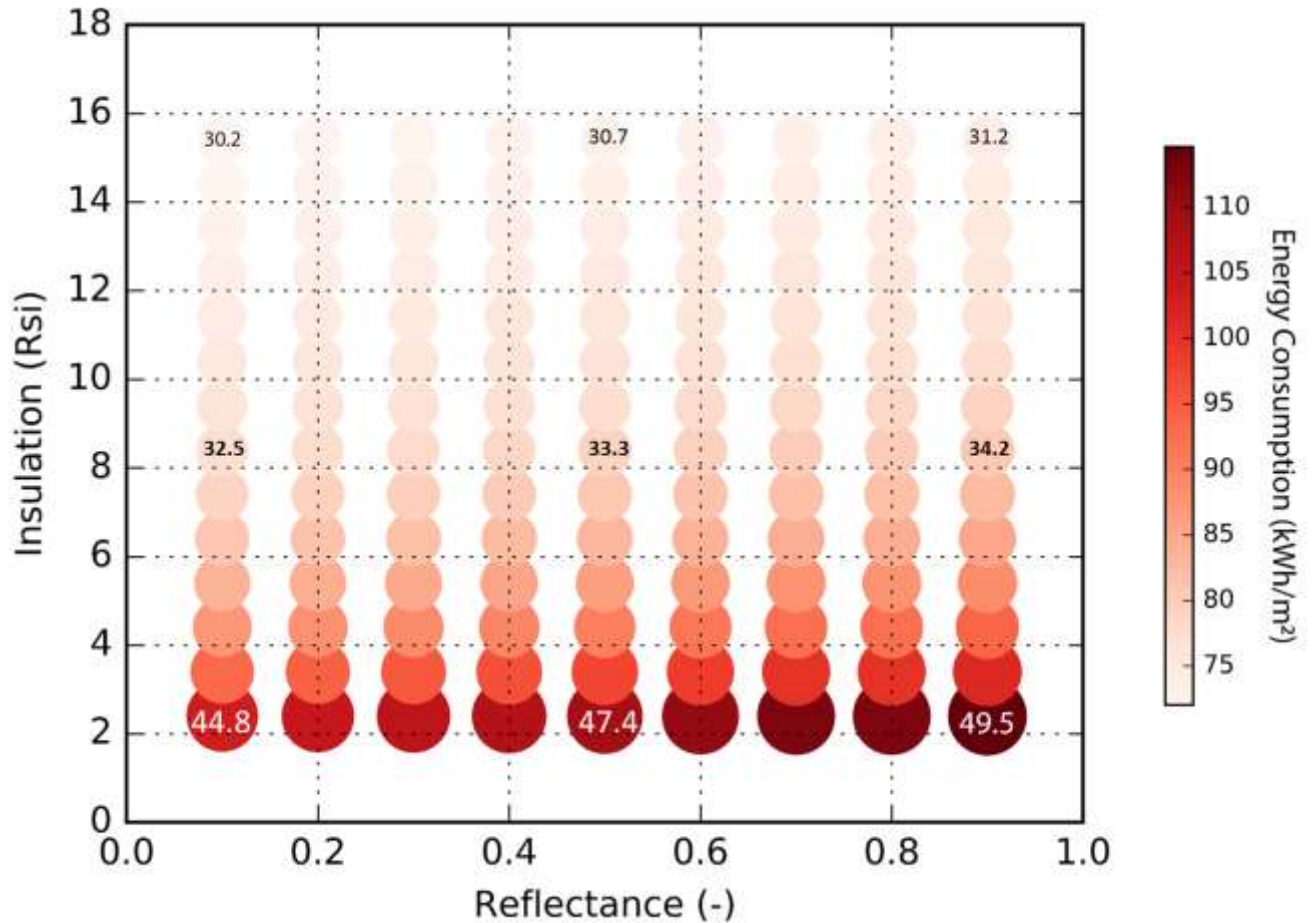
Figure 5 – Mean and variance of heating energy use for all design combinations for 2018-2037
