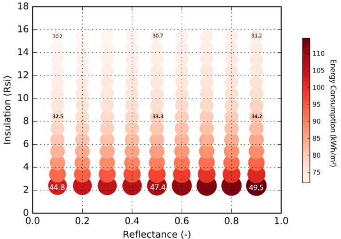
Figure 5 and 5 show average cooling and heating energy consumption of the building for the next 20 years. The bubble colours show the average intensity of future 20 years energy consumption. The variance of energy consumption for 9 designs are shown with the numbers inside the bubbles; and the bubble size indicate the relative scale in variance. The cooling plot indicates that regardless of the insulation value, a high solar reflectance value of 0.9 will lead to Pareto solutions (minimum mean and minimum variance) over all insulation values. High solar reflectance therefore minimizes the cooling energy consumption and its variance, which improves the robustness of the design. In this case, a flat roof is hit by solar rays and solar radiation becomes the most sensitive parameter. A high solar reflectance factor reduces the effects of solar radiation on energy consumption (as 90% of the solar radiation directed on the roof will be reflected towards the sky), so variations resulting from yearly variations are reduced.
