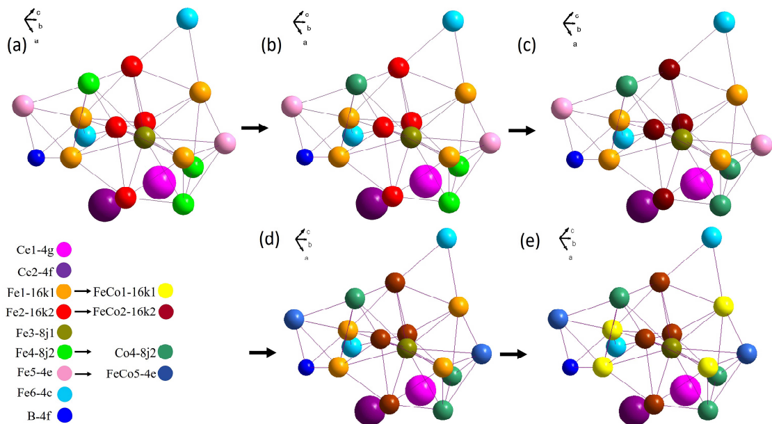
Figure 4. The coordination spheres of dynamic atomic substitution of Fe by Co with different atomic coordinates: (a) before Co substitution in \text{Ce}_2\text{Fe}_{14}\text{B} ; (b) to (c) substitution of Fe atoms by Co atoms on 8j2 site until they are completely occupied by Co and then started to occupy 16k2 site; (d) to (e) the substitution of Fe by Co atoms on 4e and 16k1 sites.
