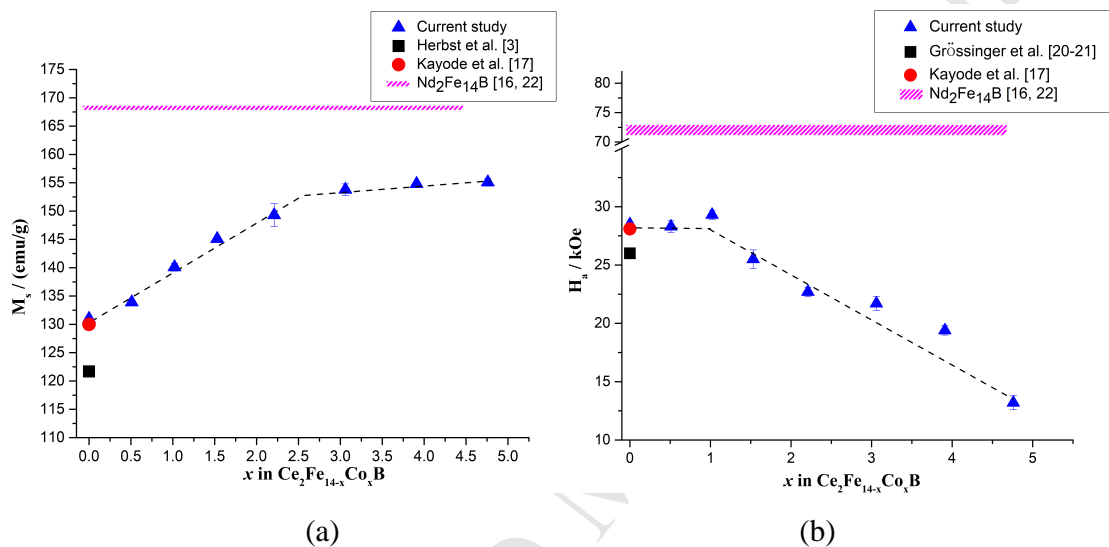
Figure 1. Compositional dependence of (a) saturation magnetization; (b) anisotropy field of \text{Ce}_2\text{Fe}_{14-x}\text{Co}_x\text{B} at 25°C. The thickness of \text{Nd}_2\text{Fe}_{14}\text{B} line represents the variation in the literature data.
