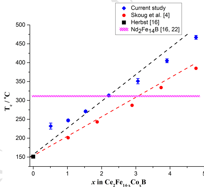
Figure 2. Current Curie temperature measurements in relation to Skoug et al. [4], Herbst [16] and Huang et al. [22].
