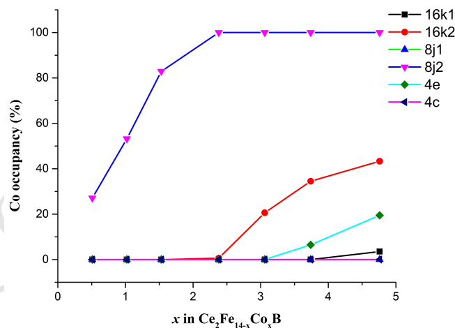
Figure 3. Co occupancy in \text{Ce}_2\text{Fe}_{14-x}\text{Co}_x\text{B} as a function of Co concentration.
