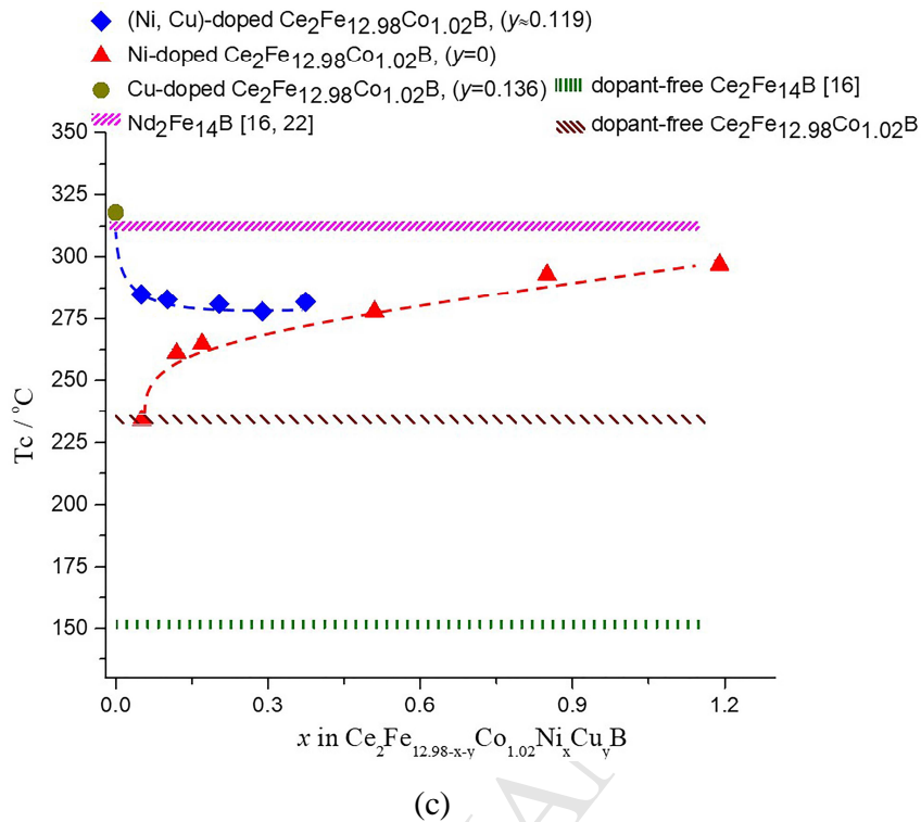
Figure 6. Compositional dependence of (a) saturation magnetization; (b) anisotropy field; (c) Curie temperature of \text{Ce}_2\text{Fe}_{12.98-x-y}\text{Co}_{1.02}\text{Ni}_x\text{Cu}_y\text{B} . The thickness of \text{Nd}_2\text{Fe}_{14}\text{B} line represents the variation in the literature data
