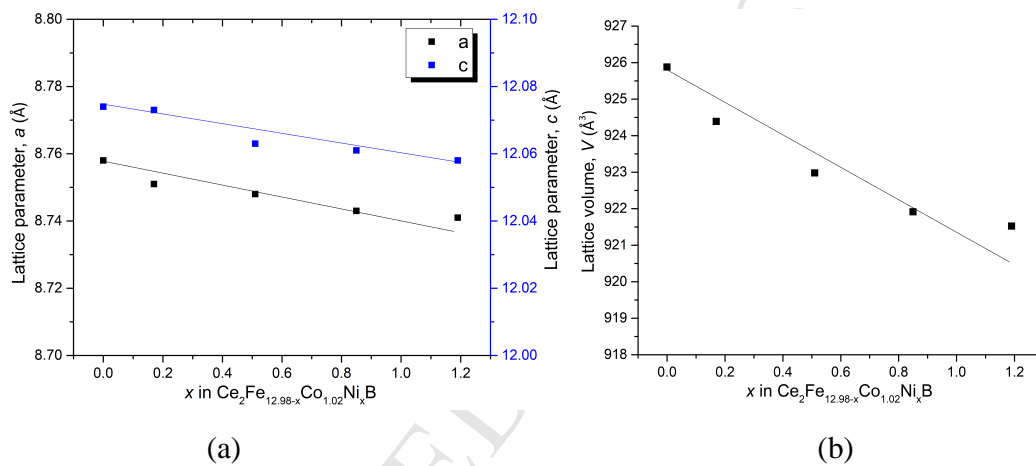
Figure 5. Cell parameters (a) a and c ; and (b) lattice volume V versus Ni concentration in \text{Ce}_2\text{Fe}_{12.98-x}\text{Co}_{1.02}\text{Ni}_x\text{B} .
