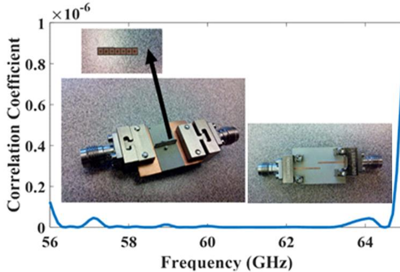
Figure 4-24: photograph of the proposed fabricated prototype, (M. Farahani et al. [51], @2017 IEEE).
