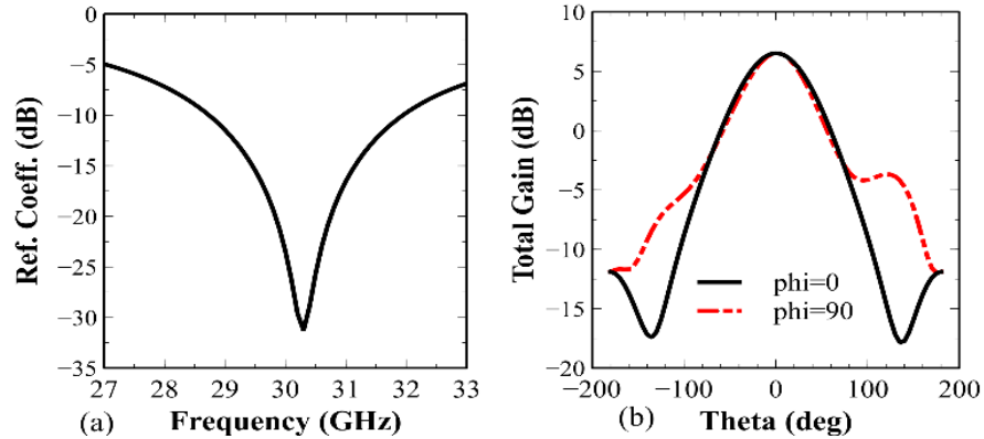
Figure 5-15: (a) The reflection coefficient and (b) radiation pattern of single ACMA at 30GHz, (M. Akbari et al. [93], @2017 IEEE).
