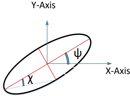
Figure 5-9: The polarization ellipse with two angles shown \psi and \chi as the geometrical parameters of the ellipse, (M. Akbari et al. [93], @2017 IEEE).
