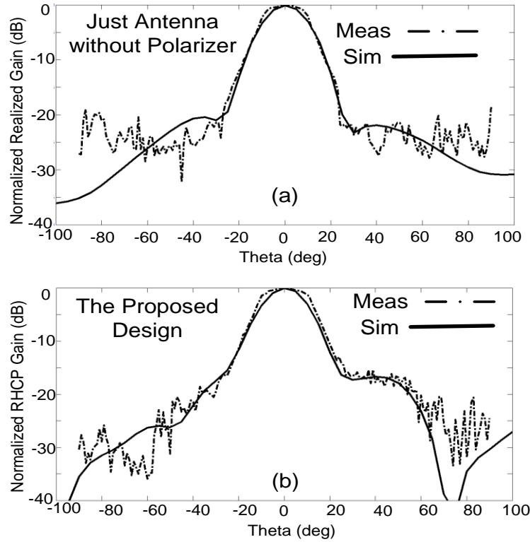
Figure 5-22: (a) The normalized total gain of the LP antenna array without the polarizer and (b) the normalized RHCP gain of the polarizer with the antenna array at 30GHz, (M. Akbari et al. [93], @2017 IEEE).
