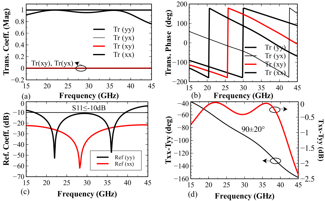
Figure 5-6: The simulated of transmission coefficients of dielectric slab with the conductor in unit cell model (a) magnitude of transmission coefficients, (b) phase of transmission coefficients, (c) reflection coefficient, and (d) difference of phase and magnitude between transmission coefficients, (M. Akbari et al. [93], @2017 IEEE).
