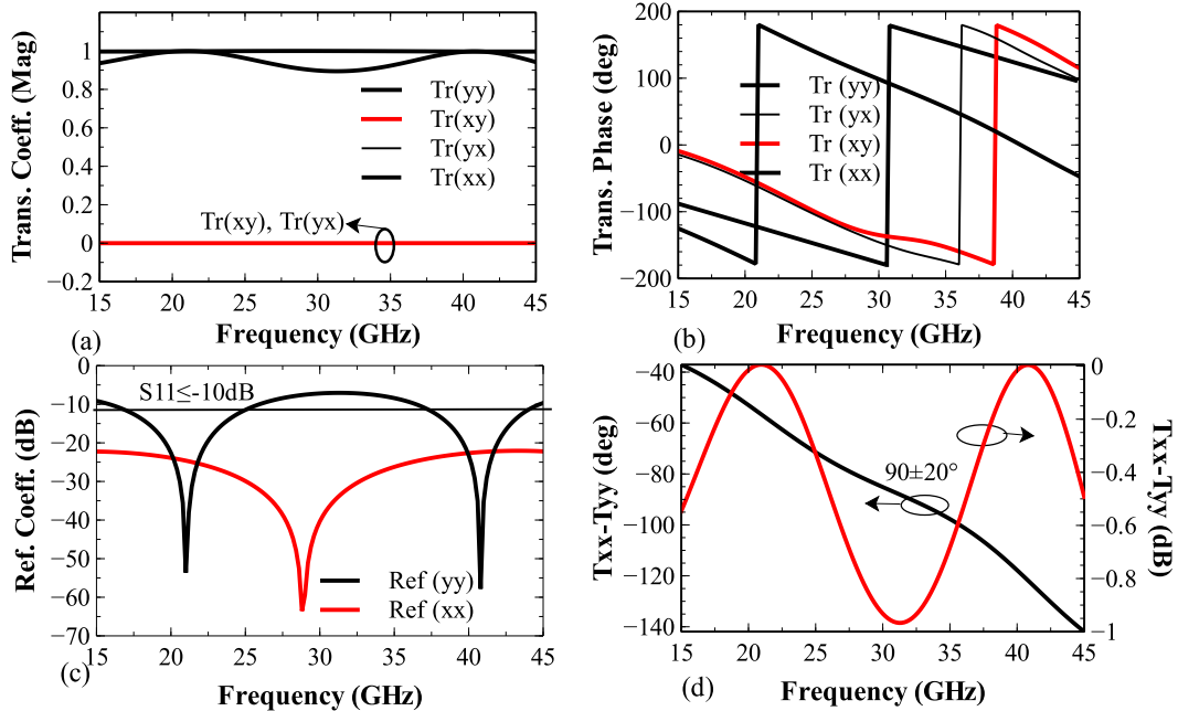
Figure 5-4: The simulated of transmission coefficients of dielectric slab without the conductor in unit cell model (a) magnitude of transmission coefficients, (b) phase of transmission coefficients, (c) reflection coefficient, and (d) difference of phase and magnitude between transmission coefficients, (M. Akbari et al. [93], @2017 IEEE).
