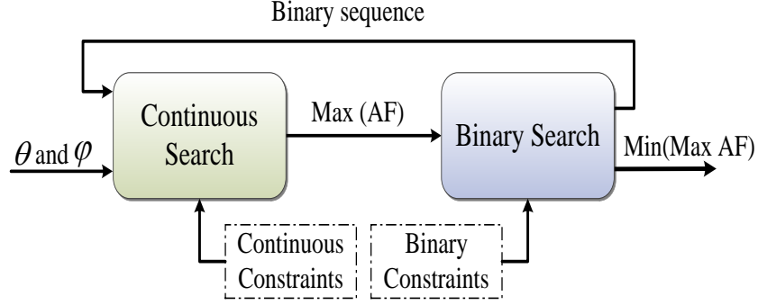
Figure A-3: Defined bi-level model of algorithm, (M. Akbari, F. Samadi et al. [136], @2019 IEEE) and (F. Samadi, M. Akbari et al. [18], @2019 IEEE).
