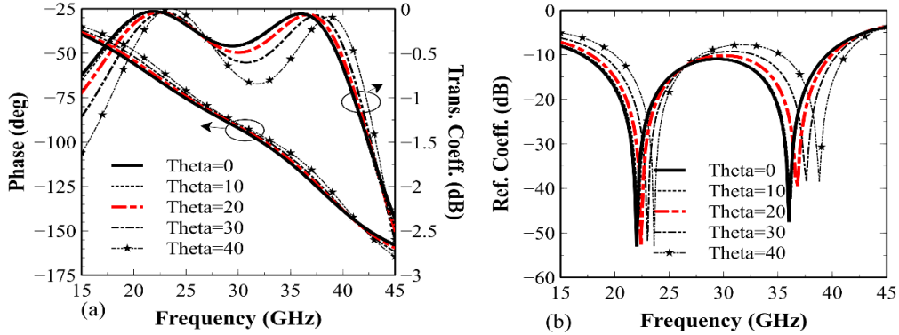
Figure 5-7: The results related to the dielectric slab with circle conductor in the unit cell model when is illuminated by an incident wave with different oblique angles (a) magnitude and phase of transmission coefficients, (b) reflection coefficients, (M. Akbari et al. [93], @2017 IEEE).
