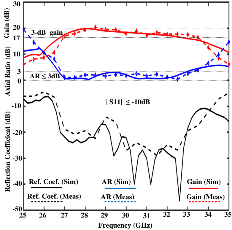
Figure 6-34: The simulated and measured reflection coefficient , AR, and gain for FPC antenna (with metasurface), (S. Zarbakhsh, M. Akbari et al. [32], @2019 IEEE).
