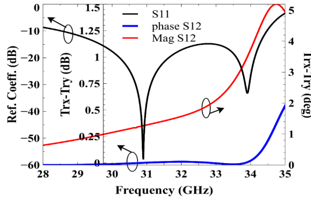
Figure 4-4: simulated results of S-parameter for the unit cell model of FSS, (M. Akbari et al. [49], @2017 IEEE).
