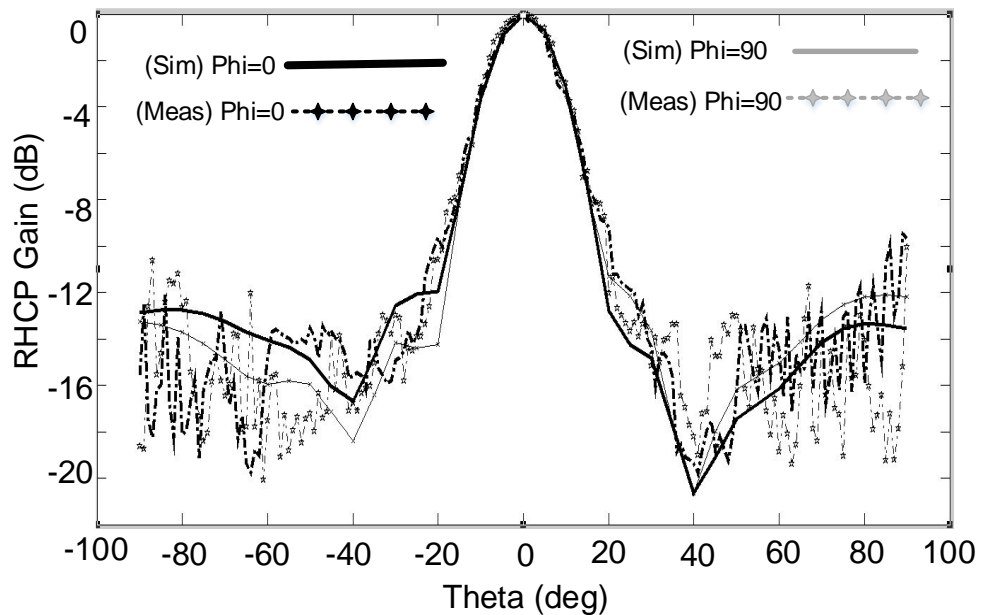
Figure 3-12: The normalized gain of the proposed antenna at 30GHz on both planes \phi=0 and \phi=90 , (M. Akbari et al. [31], @2016 IEEE).
