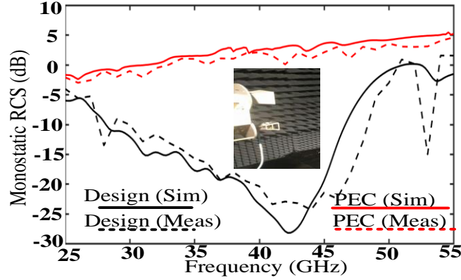
Figure 6-36: The simulated and measured monostatic RCS of the proposed FPC antenna and the PEC metasurface with the identical size under normal incidence, the photo of two types of horn antennas used for transmitting and receiving, (S. Zarbakhsh, M. Akbari et al. [32], @2019 IEEE).
