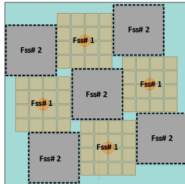
Figure 6-29: The FSS metasurface including structures of FSS#1 and FSS#2, (each FSS structure is formed by 4×4 FSS unit cells), (S. Zarbakhsh, M. Akbari et al. [32], @2019 IEEE).
