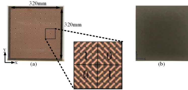
Figure 6-20: The photo of fabricated two-layer metasurface (a) bottom layer (reflective coding matrix metasurface) and (b) top layer (without any copper), (M. Akbari et al. [136], @2019 IEEE).
