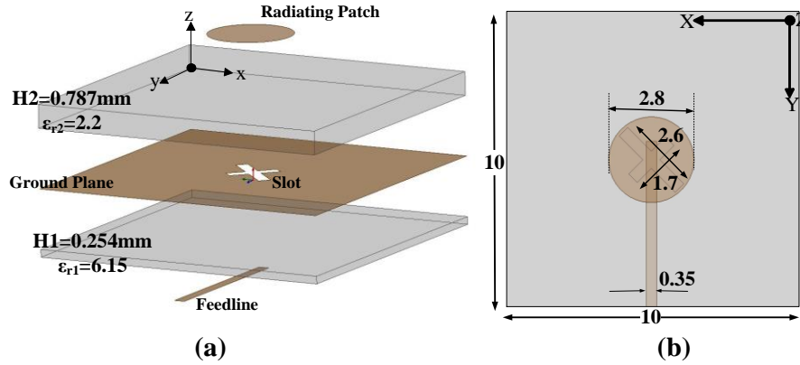
Figure 4-5: Geometry of single CP-ACMA (a) side view and (b) top view, (M. Akbari et al. [49], @2017 IEEE).
