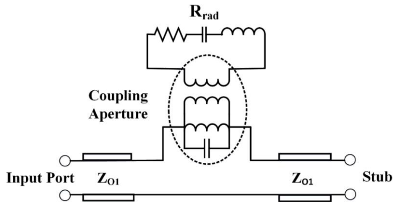
Figure 5-14: The equivalent circuit model of the ACMA [117], (M. Akbari et al. [93], @2017 IEEE).
