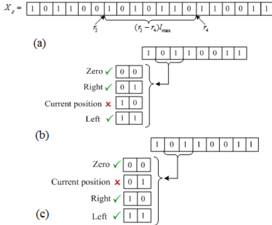
Figure A-1: (a) Random length selection for the producer member (b) Defining zero, right and left points, and (c) Producing procedure at the second step of head angle (F. Samadi, M. Akbari et al. [18], @2019 IEEE).
