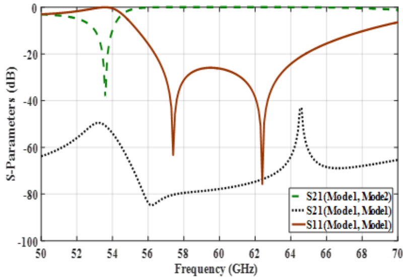
Figure 4-20: Transmission/reflection coefficients of the proposed MPR unit cell, (M. Farahani et al. [51], @2017 IEEE).
