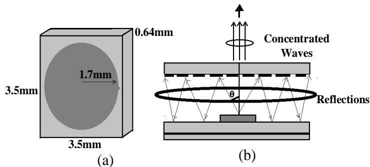
Figure 3-4: (a) The dimensions of the FSS unit cell and (b) illustration of multiple reflections and leaky waves, (M. Akbari et al. [31], @2016 IEEE).
