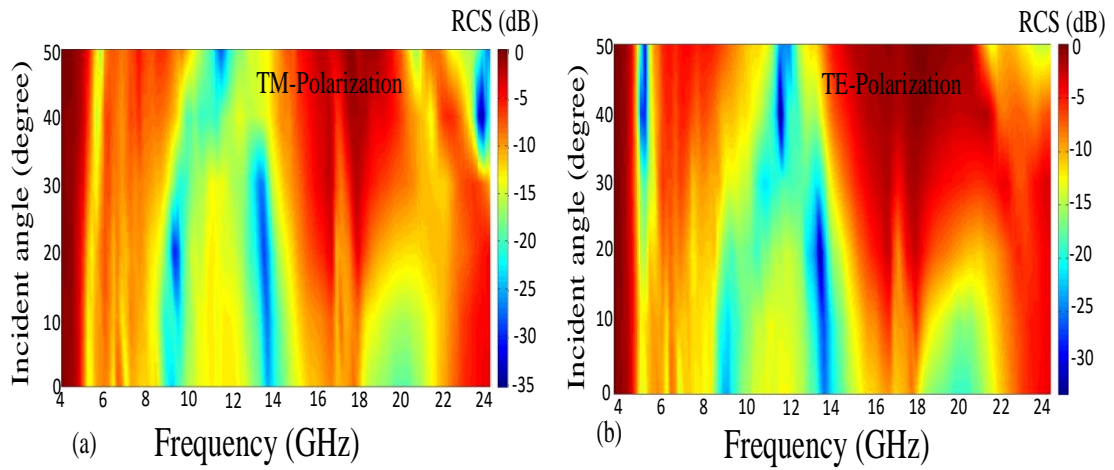
Figure 6-17: Maps of the simulated RCS reduction versus frequency range at different incidence angles for (a) TM and (b) TE polarizations, (M. Akbari et al. [136], @2019 IEEE).
