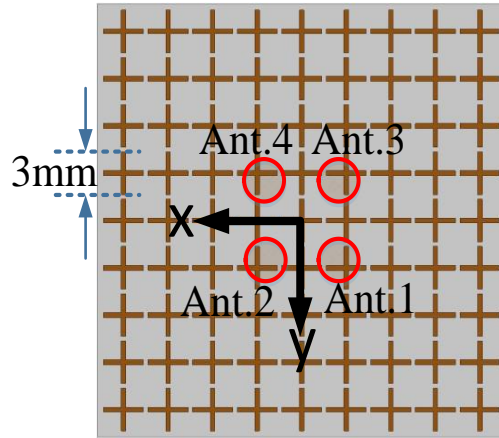
Figure 4-10: The formation schematic of FSS superstrate including 9 \times 9 FSS elements, and the precise position of a 2 \times 2 MIMO-ACMA below the superstrate in the x - y plane (the inter-element spacing d_i = \lambda/2 ), (M. Akbari et al. [49], @2017 IEEE).
