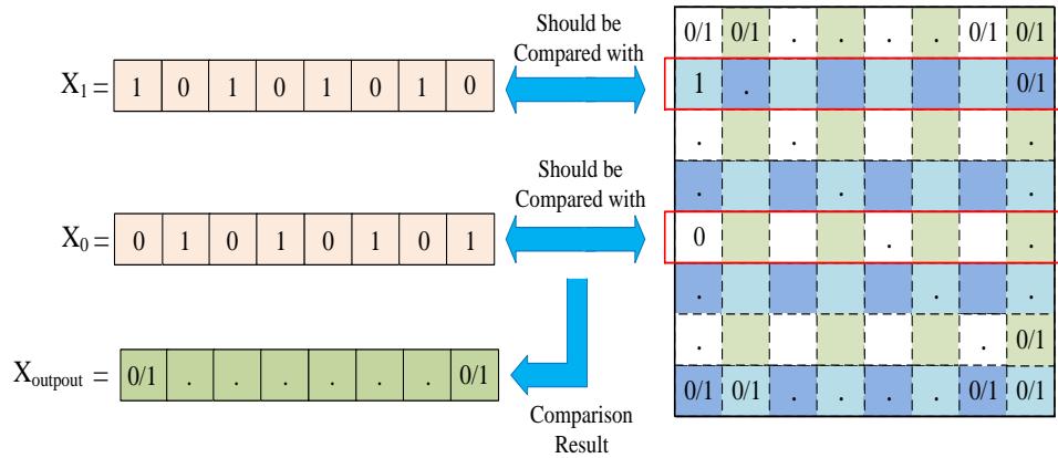
Figure A-4: (a) 1 \times 8 , x_0 and x_1 vectors, (b) 8 \times 8 , random matrix, and (c) 1 \times 8 , x output, (F. Samadi, M. Akbari et al. [18], @2019 IEEE).
