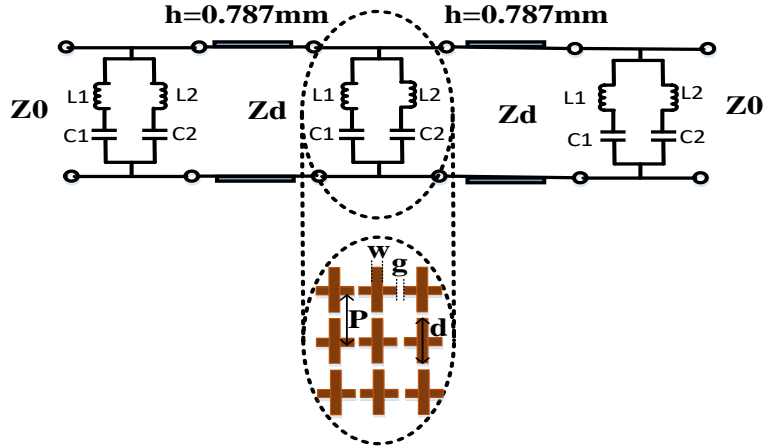
Figure 4-2: The equivalent circuit of FSS layers including inductive and capacitive elements [116], (M. Akbari et al. [49], @2017 IEEE).
