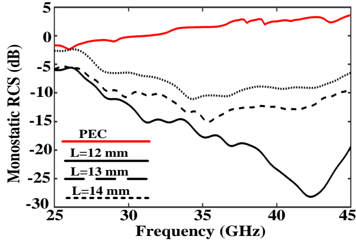
Figure 6-32: The monostatic RCS comparison of the FPC antenna with both the proposed and PEC metasurface with “L” parameter variations, (S. Zarbakhsh, M. Akbari et al. [32], @2019 IEEE).
