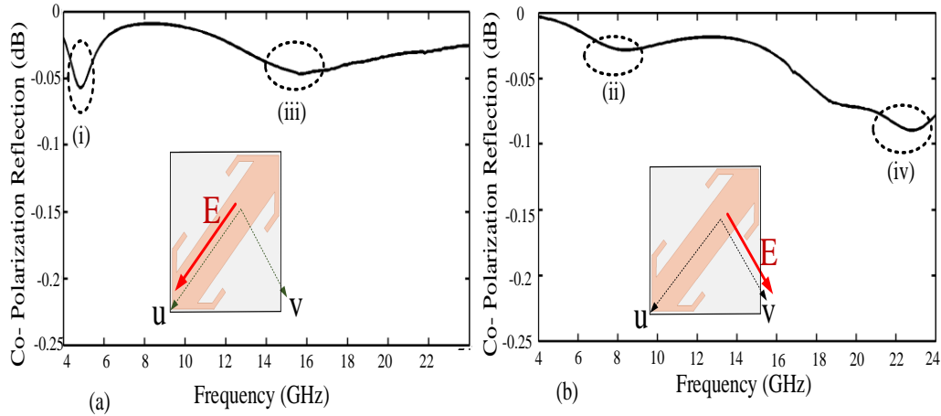
Figure 6-2: The four resonances of the proposed FSS under normal incidence: (a) u-polarized case and (b) v-polarized case, (M. Akbari et al. [136], @2019 IEEE).
