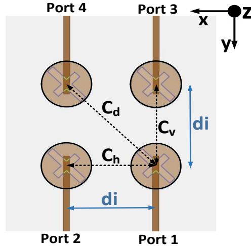
Figure 4-8: The schematic diagram of the MIMO-ACMAs with coupling coefficients ( C_d , C_h , and C_v ) and the inter-ACMA element spacing ( d_i ), (M. Akbari et al. [49], @2017 IEEE).
