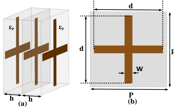
Figure 4-3: The unit cell model of crossed dipole FSS (a) side view and (b) top view ( d=2.7\text{mm} , P=3\text{mm} , W=0.3\text{mm} and \epsilon_r=2.2 , and h=0.787\text{mm} ), (M. Akbari et al. [49], @2017 IEEE).
