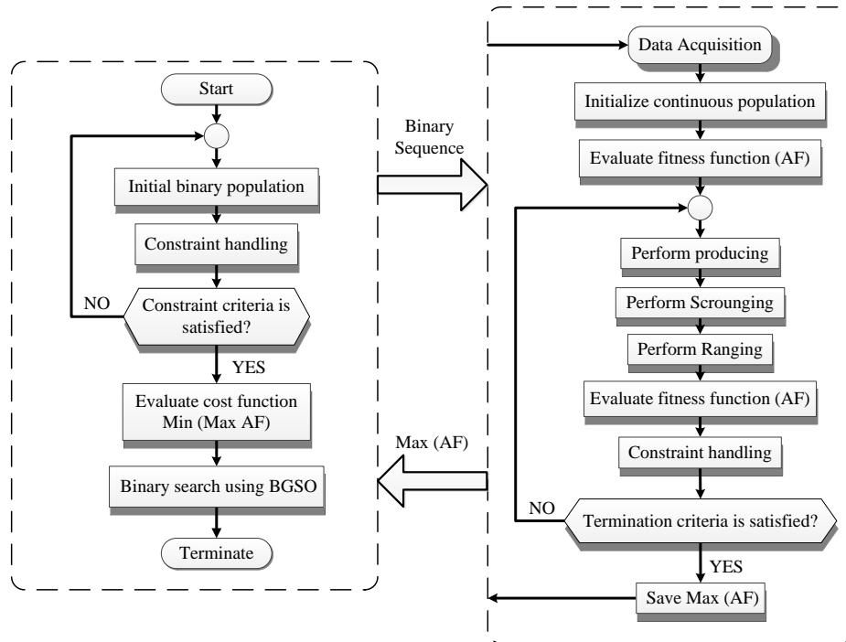
Figure A-6: Flowchart of bi-level GSO algorithm, (F. Samadi, M. Akbari et al. [18], ©2019 IEEE)
