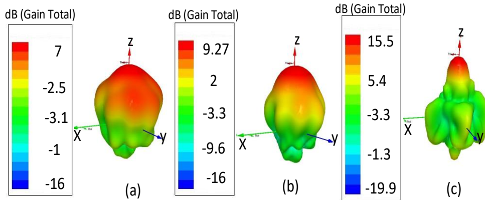
Figure 3-9: 3D radiation patterns of the aperture coupled DRA at 30 GHz for three cases: (a) the basic DRA, (b) the DRA with the only superstrate, and (c) DRA with the FSS superstrate, (M. Akbari et al. [31], ©2016 IEEE).
