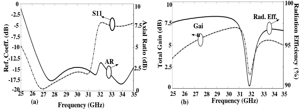
Figure 3-3: The simulated results of (a) reflection coefficient and axial ratio, and (b) total gain and radiation efficiency of the DRA without the FSS layer, (M. Akbari et al. [31], @2016 IEEE).
