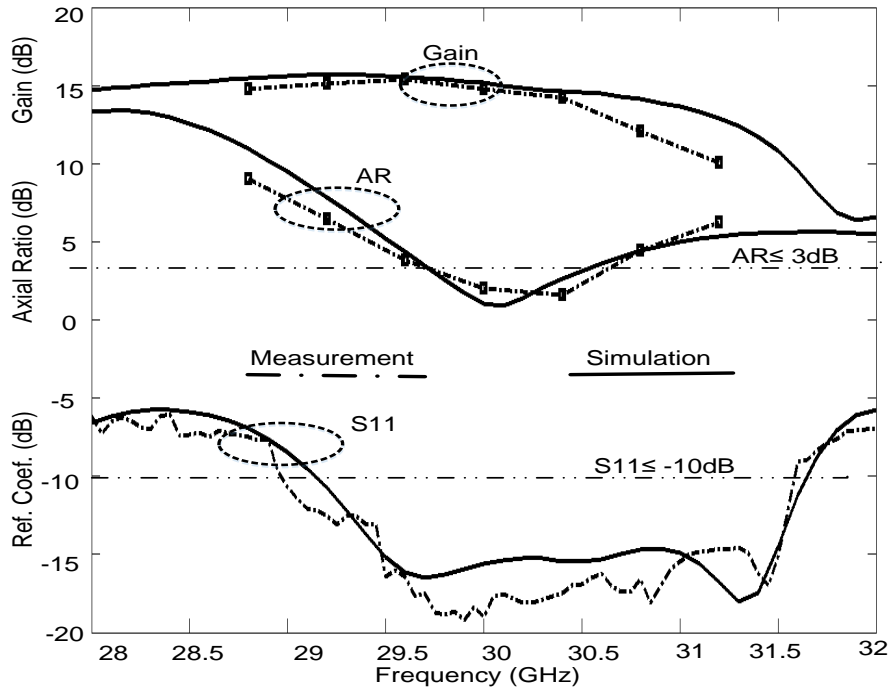
Figure 3-11: Measured and simulated curves of the total gain, axial ratio, and reflection coefficient of the proposed antenna, (M. Akbari et al. [31], @2016 IEEE).
