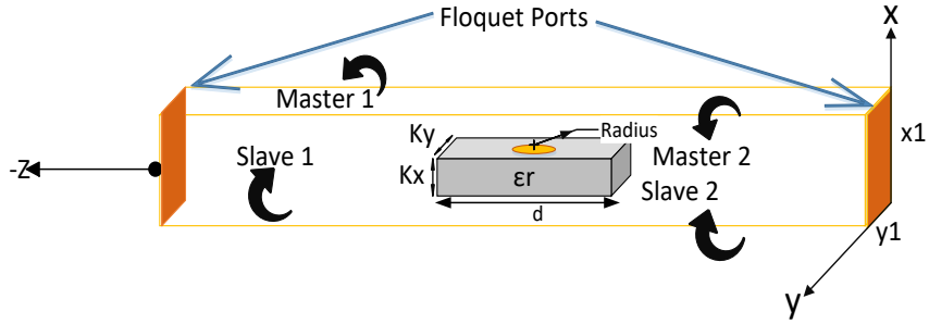
Figure 5-2: The unit cell model by HFSS software ( x_1=1.6\text{mm} , y_1=1\text{mm} , d=4.6\text{mm} , k_x=0.254\text{mm} , k_y=1\text{mm} , \epsilon_r=10.2 , \text{Radius}=0.3\text{mm} ), (M. Akbari et al. [93], @2017 IEEE).
