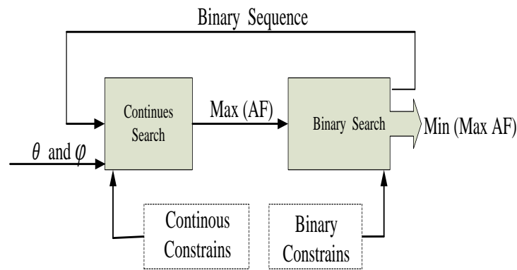
Figure 6-8: The Defined bi-level model of the algorithm, (M. Akbari et al. [136], @2019 IEEE).
