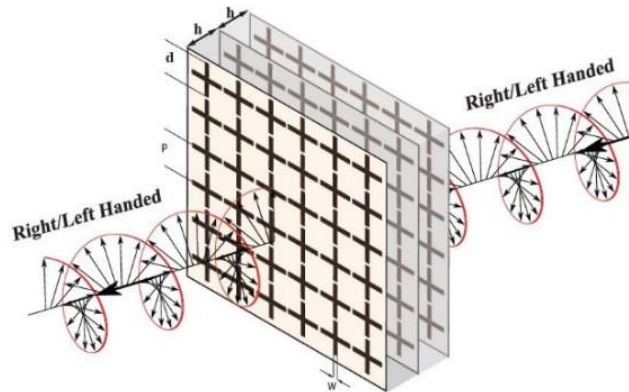
Figure 4-1: The schematic model of the transmission-type FSS superstrate illuminating by CP wave ( h=0.787\text{mm} , d=2.7\text{mm} , P=3\text{mm} , and W=0.3\text{mm} ), (M. Akbari et al. [49], @2017 IEEE).
