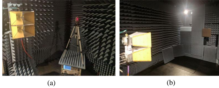
Figure 6-21: (a) the same antennas as transmitting and receiving along E8364B PNA and (b) the measurement set up and the proposed fabricated design inside the anechoic chamber, (M. Akbari et al. [136], @2019 IEEE).
