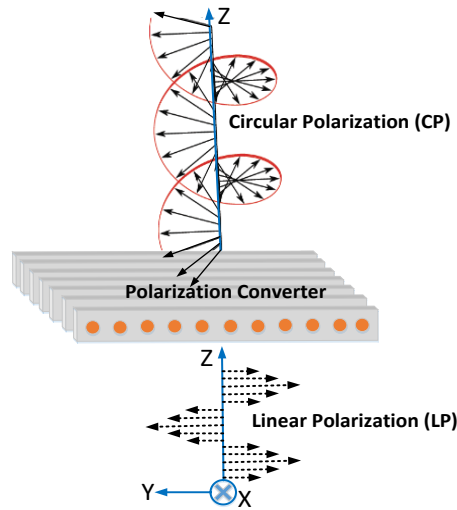
Figure 5-1: Schematic model of a linear-to-circular polarizer, (M. Akbari et al. [93], @2017 IEEE).
