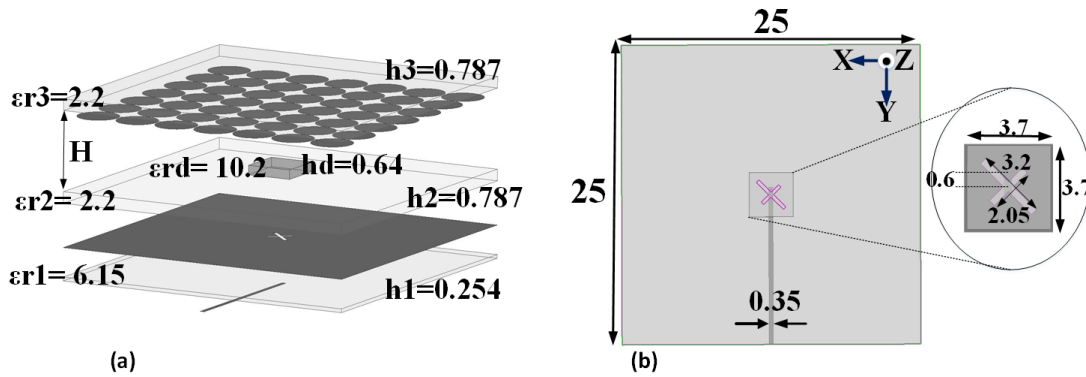
Figure 3-1: The geometry of the FPC antenna with radiating DR and an FSS superstrate layer (a) 3D view and (b) top view (measurements are in millimetre), (M. Akbari et al. [31], @2016 IEEE).
