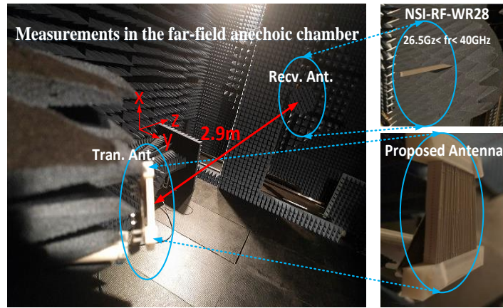
Figure 5-20: The photo of the antenna under test in the far-field anechoic chamber, (M. Akbari et al. [93], @2017 IEEE).
