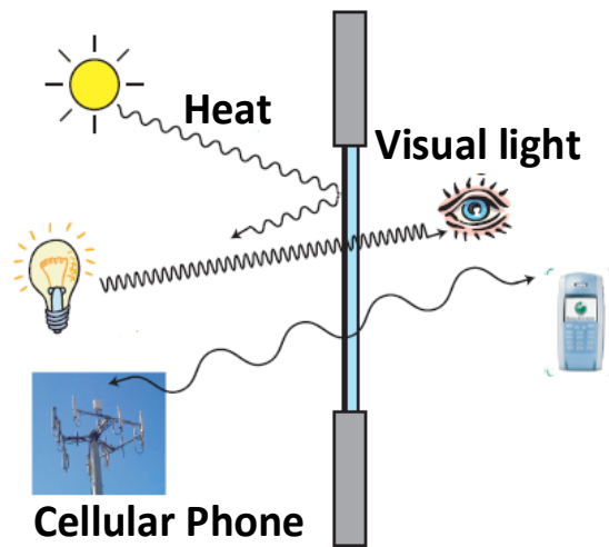
Figure 2-3: Illustration of a frequency selective window. The infrared radiation (heat) is blocked by the window, but the indoor outdoor communication is possible. The visible part of the spectrum remains unchanged (M. Gustafsson, et al. [24], @ Lund University, 2005).
