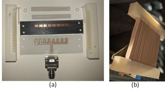
Figure 5-19: The photo of (a) the assembled design and (b) the proposed structure, (M. Akbari et al. [93], @2017 IEEE).
