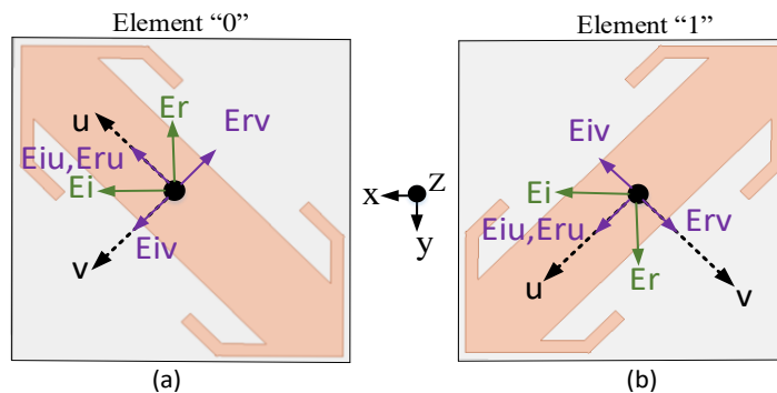
Figure 6-4: Intuitive image of the x -polarized wave ( E incident field along the x -axis) normally illuminating the FSS cell of (a) the elements “0” and (b) “1”, (M. Akbari et al. [136], ©2019 IEEE).
