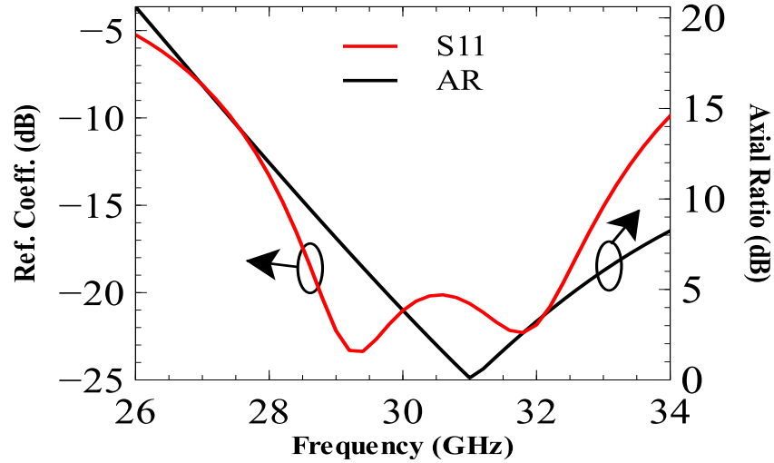
Figure 4-7: Reflection coefficient and axial ratio of a single element CP patch, (M. Akbari et al. [49], @2017 IEEE).
