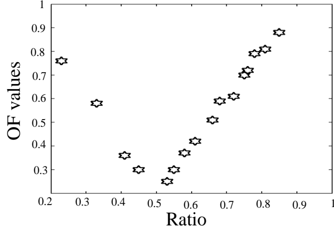
Figure 6-9: Optimized OF values versus ratio of “1” and “0” elements, (M. Akbari et al. [136], @2019 IEEE).
