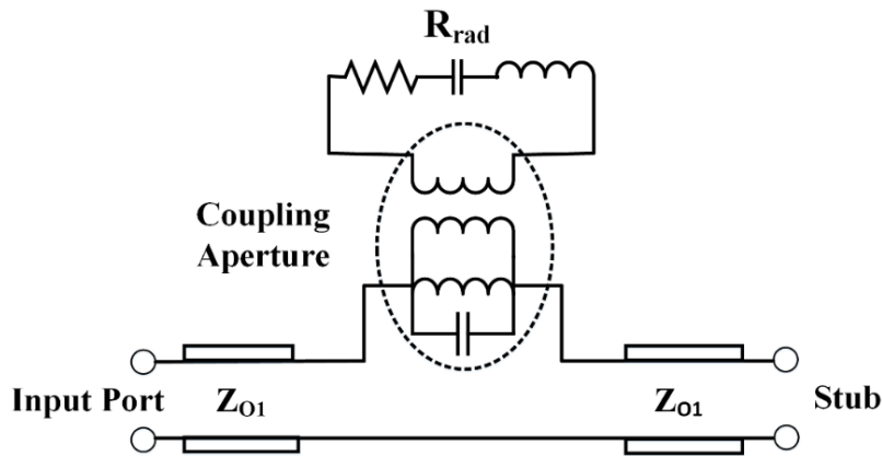
Figure 4-6: The equivalent circuit model of the ACMA [117], (M. Akbari et al. [49], @2017 IEEE).
