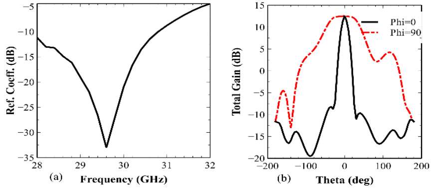
Figure 5-17: (a) The reflection coefficient and (b) radiation pattern of 8-element linear array antennas at 30GHz, (M. Akbari et al. [93], @2017 IEEE).
