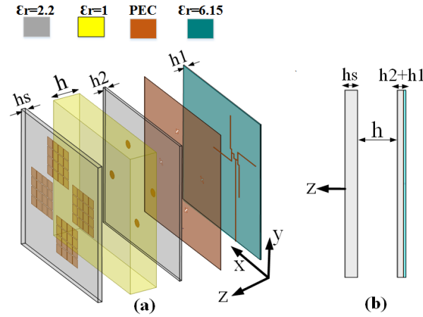
Figure 6-28: (a) The 3-D configuration and (b) side view of the FPC antenna ( h_1=0.25\text{mm} , h_2=0.787\text{mm} , h=4.8\text{mm} , h_s=1.52\text{mm} ), (S. Zarbakhsh, M. Akbari et al. [32], @2019 IEEE).
