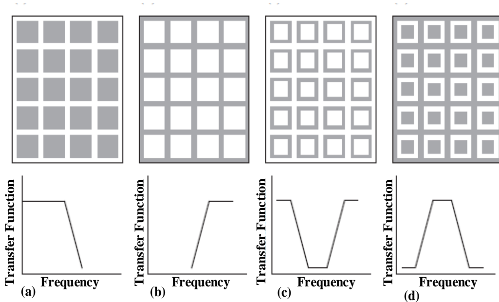
Figure 2-4: Typical FSS types and their responses. The gray surface represents a metallic surface. (a) array of metallic patches and respective low pass behavior, (b) apertures on the conductive medium and ideally high pass transfer function. Figures (c) and (d) show the loop elements that have resonant characteristics (c) metallic loop and (d) aperture loop (M. Gustafsson, et al. [24], @ Lund University, 2005).
