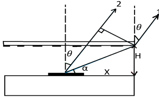
Figure 3-7: Model of the diffraction and transmission rays, (M. Akbari et al. [31], @2016 IEEE).
