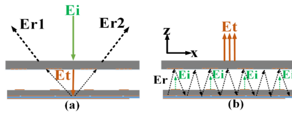
Figure 6-23: The schematic view of the proposed structure including the antenna with the FSS metasurface for two cases of (a) RCS reduction and (b) gain enhancement, ], (S. Zarbakhsh, M. Akbari et al. [32], @2019 IEEE).
