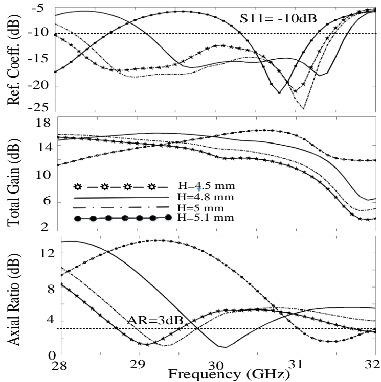
Figure 3-8: The simulated results of the reflection coefficient, total gain, and axial ratio for different values of the airgap height H, (M. Akbari et al. [31], @2016 IEEE).
