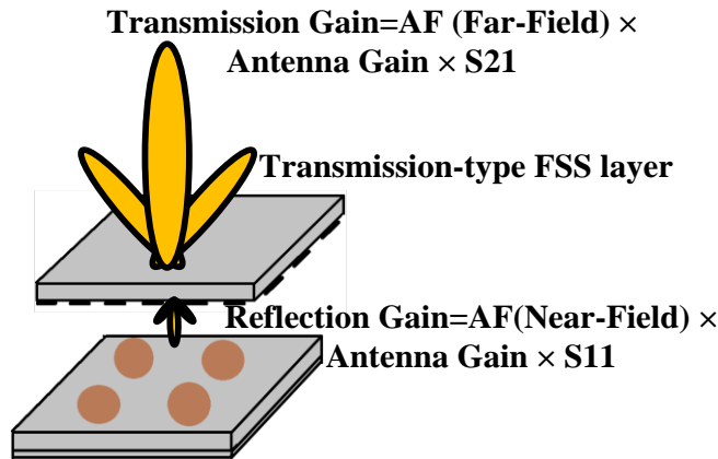
Figure 4-9: The schematic of the transmission-type FSS layer with transmission and reflection gains in two directions with respect to AF and S-parameters, (M. Akbari et al. [49], @2017 IEEE).
