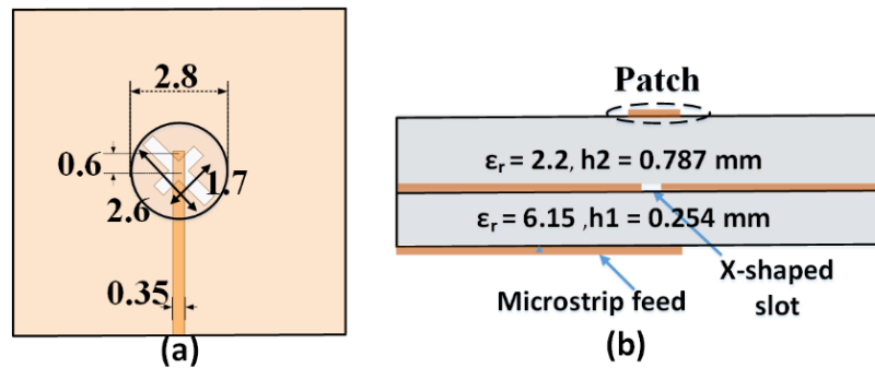
Figure 6-24: The geometry of patch antenna (a) top view and (b) side view [4], (S. Zarbakhsh, M. Akbari et al. [32], @2019 IEEE).
