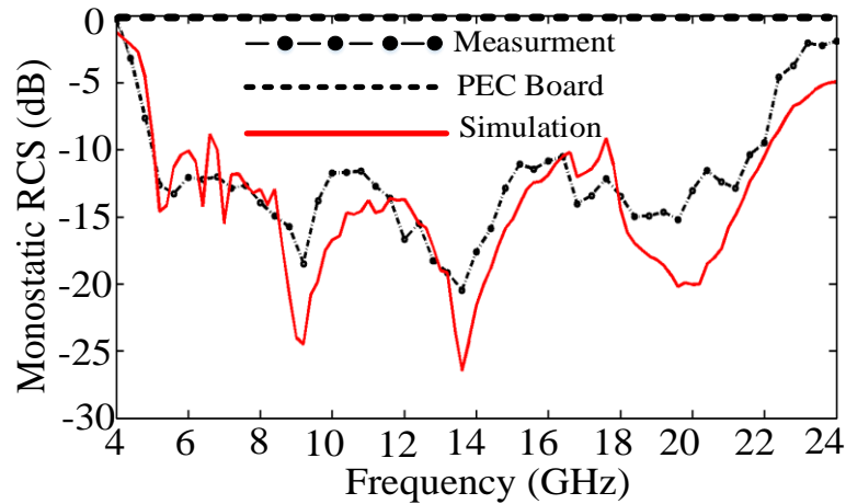
Figure 6-22: Normalized RCS reduction of the proposed reflective metasurface at normal incidence with respect to an equal size metallic plate. Solid and dashed lines represent: the simulated and measured diagrams, respectively, (M. Akbari et al. [136], @2019 IEEE).
