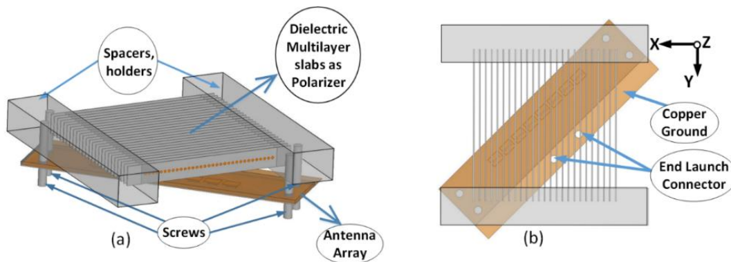
Figure 5-18: The final proposed design, including the multilayer slab polarizer, the antenna array, spacer, screws; (a) isometry view and (b) top view, (M. Akbari et al. [93], @2017 IEEE).
