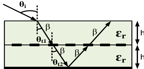
Figure 6-18: Diagrammatic sketch of EM wave propagation in a two-layer dielectric substrate at oblique incidence ( \theta_{t1} \simeq \theta_{t2} \simeq \theta_i ), (M. Akbari et al. [136], @2019 IEEE).
