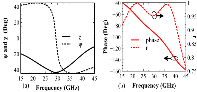
Figure 5-10: (a) The simulated angles of polarization azimuth ( \psi ) and ellipticity ( \chi ) and (b) the phase difference ( \Delta\phi ) and amplitude ratio ( r ) versus frequency, (M. Akbari et al. [93], @2017 IEEE).
