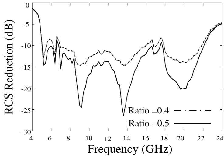
Figure 6-13: Normal incidence RCS reduction for different ratios versus frequency, (M. Akbari et al. [136], ©2019 IEEE).
