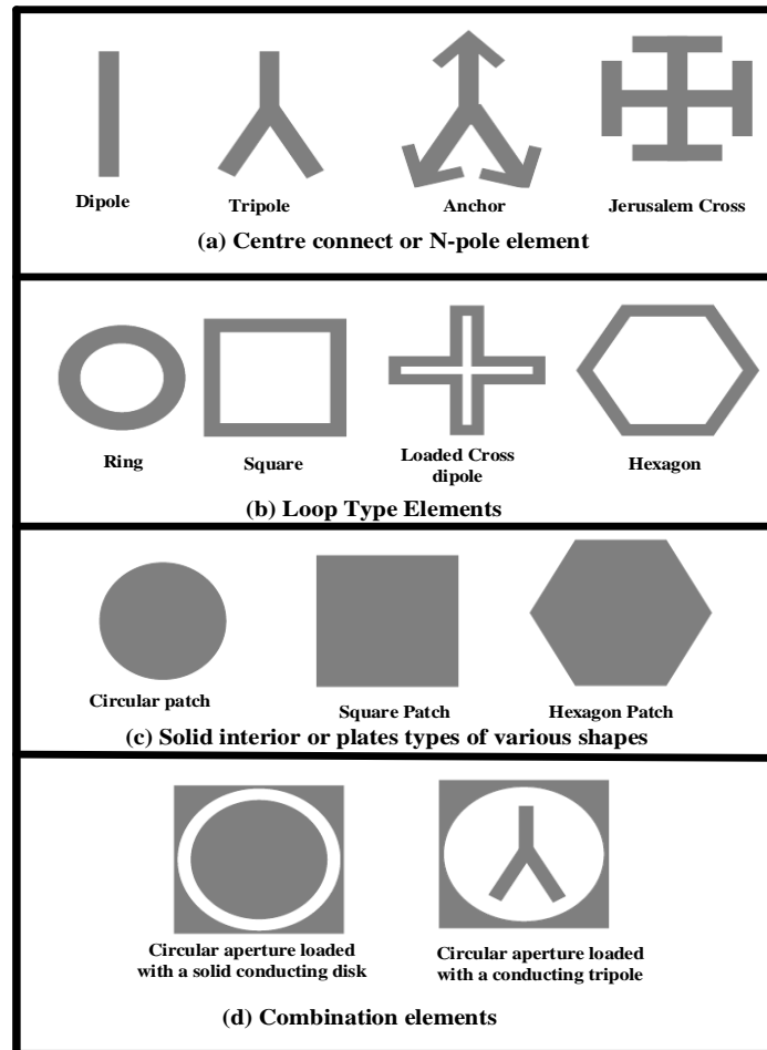
Figure 2-5: Common FSS element types (B. Turki, et al. [25], @ University of Kent, 2015).
