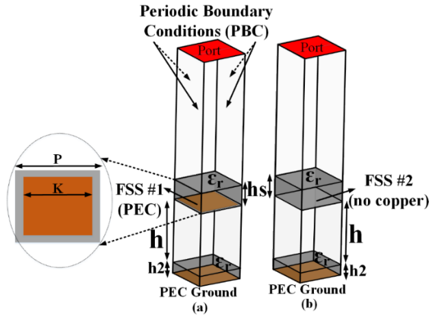
Figure 6-26: The simulated models of the FSS unit cells (a) FSS#1 and (b) FSS#2 ( P=3.5\text{mm} , K=3.2\text{mm} , h=4.8\text{mm} , h_2=0.787\text{mm} , h_s=1.52\text{mm} , \epsilon_r=2.2 ), (S. Zarbakhsh, M. Akbari et al. [32], ©2019 IEEE).
