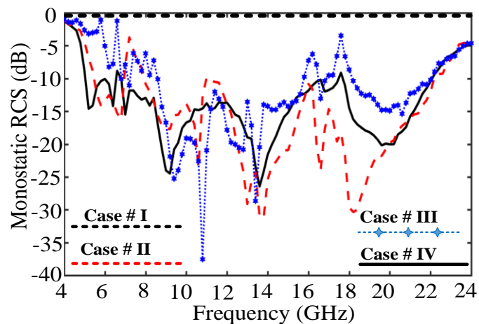
Figure 6-16: Normalized RCS reduction of the designs for the different cases (shown in Figure 6-15) at normal incidence with respect to an equal size metallic plate, (M. Akbari et al. [136], @2019 IEEE).
