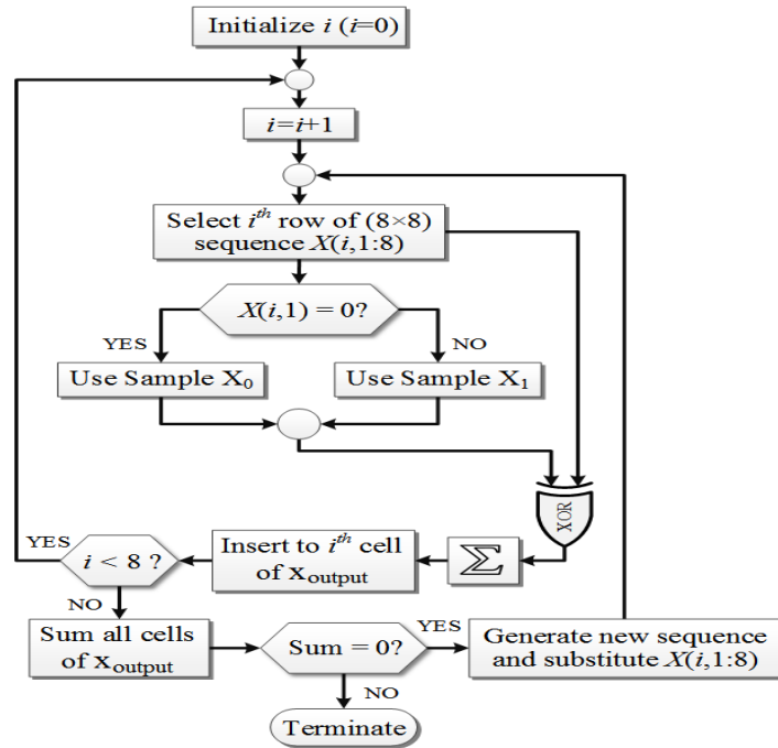
Fig. A-5: Constraint handling process in binary space, (F. Samadi, M. Akbari et al. [18], ©2019 IEEE)
