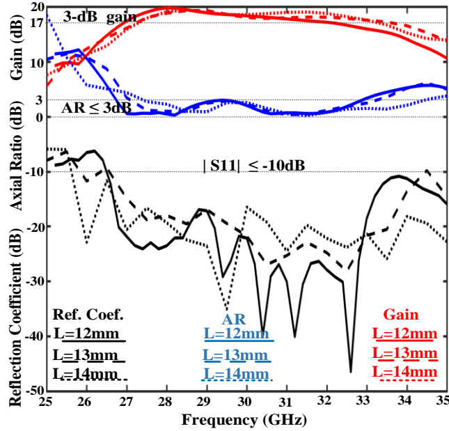
Figure 6-31: The simulated reflection coefficient , AR, and gain for FPC antenna (with metasurface) for “L” parameter variations, (S. Zarbakhsh, M. Akbari et al. [32], @2019 IEEE).
