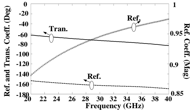
Figure 3-6: The phase and magnitude of reflection and transmission coefficients of the FSS unit cell, (M. Akbari et al. [31], @2016 IEEE).
