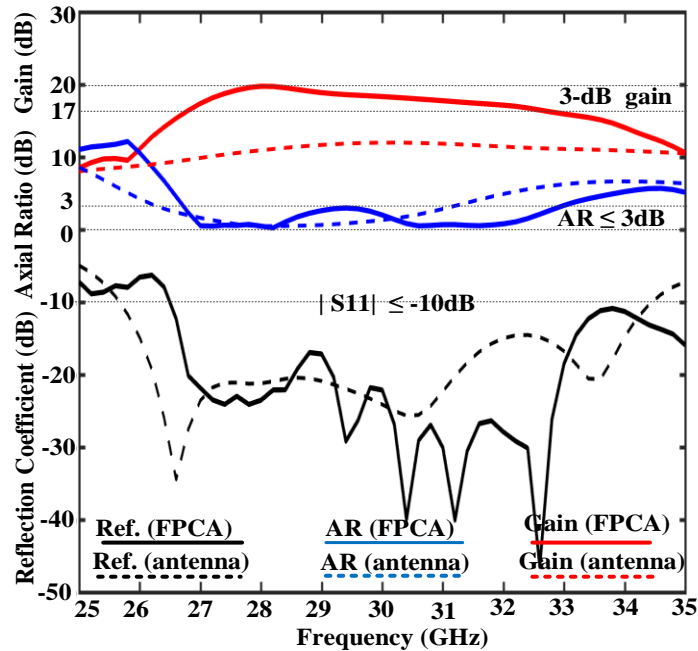
Figure 6-30: The simulated gain, AR, and reflection coefficient, for both the source antenna (without metasurface) and the FPC antenna (with metasurface), (S. Zarbakhsh, M. Akbari et al. [32], @2019 IEEE).
