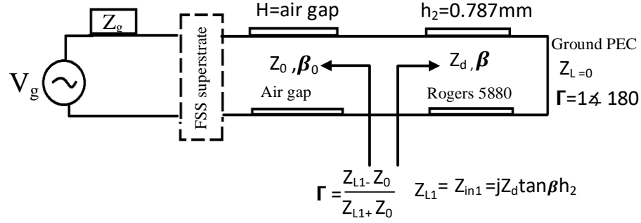
Figure 3-5: Transmission line circuit model for mismatched load and generator, (M. Akbari et al. [31], @2016 IEEE).
