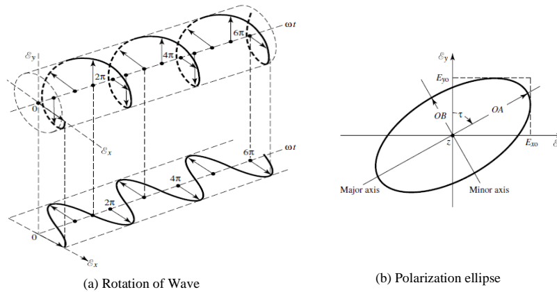
Figure 1-1: Rotation of a plane electromagnetic (EM) wave and its polarization ellipse at z = 0 as a function of time, (C. A. Balanis et al. [8], @ 2005 Wiley & Sons).
