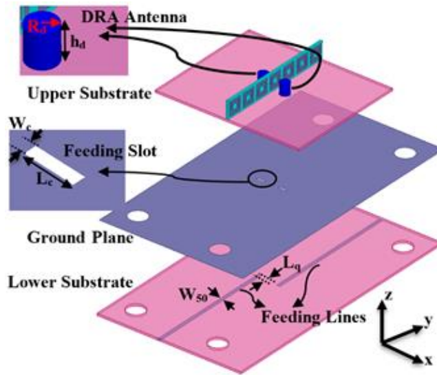
Figure 4-21: The layout of the 1 \times 2 DR MIMO antenna with the FSS wall. The dimensions are R_d=0.53 , h_d=1.27 , W_c=0.18 , L_c=0.87 , W_{50}=0.41 , L_q=0.3 , and all in millimetre, (M. Farahani et al. [51], @2017 IEEE).
