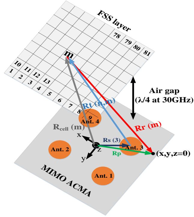
Figure 4-11: The sketch of a uniform rectangular array of 81 FSS elements with spacing 3mm along the x and y-axis above 2x2 MIMO-ACMA with an air gap 2.5mm along z-axis, (M. Akbari et al. [49], @2017 IEEE).
