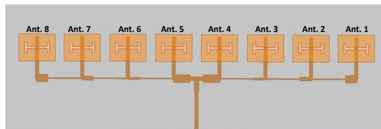
Figure 5-16: The 8-element linearly polarized array ACMA with Chebyshev tapered distribution, (M. Akbari et al. [93], @2017 IEEE).
