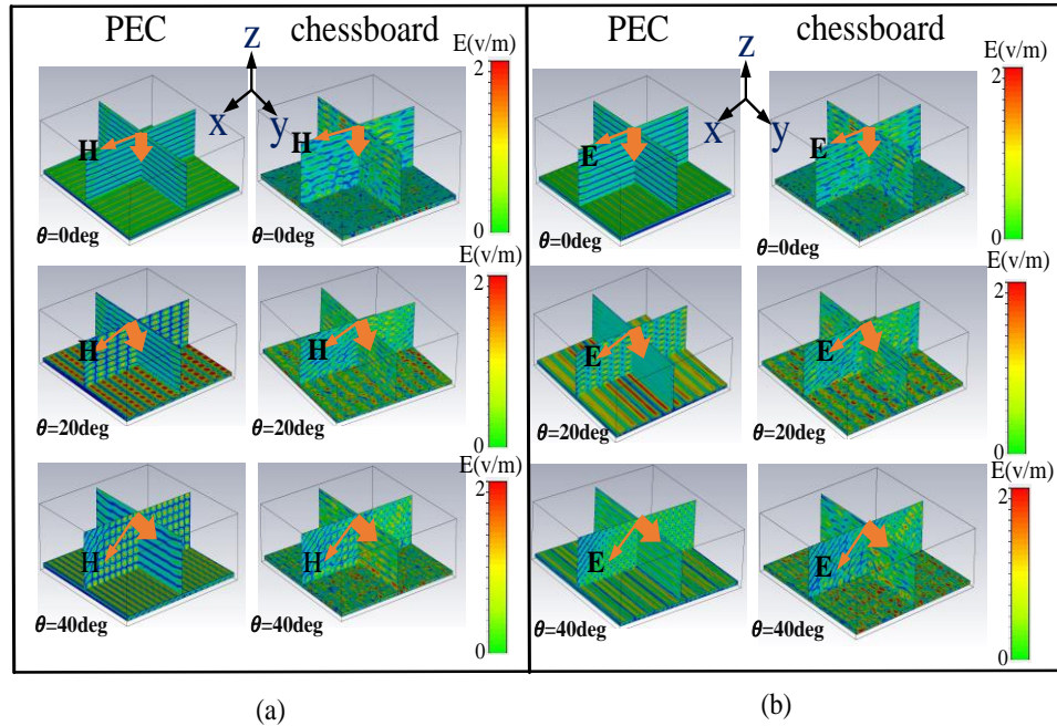
Figure 6-19: Near-fields of reflective metasurface with optimized coding matrix and PEC at 14 GHz for an incident angle of 0 deg, 20 deg, and 40 deg (a) TE polarization and (b) TM polarization, (M. Akbari et al. [136], @2019 IEEE).
