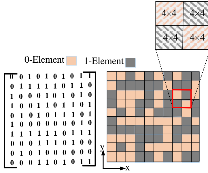
Figure 6-12: Proposed coding matrix and associated metasurface, (M. Akbari et al. [136], ©2019 IEEE).
