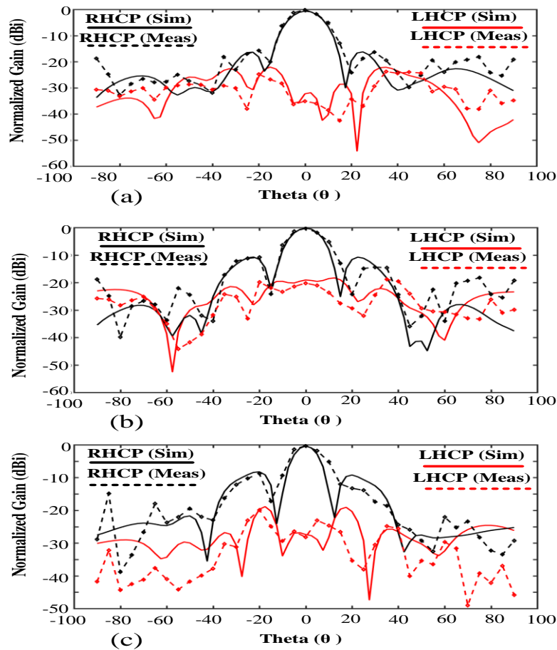
Figure 6-35: The normalized simulations and measurements of RHCP and LHCP gain at \varphi=45^\circ for the FPC antenna at three frequencies of (a) 27.5 GHz, (b) 30 GHz, and (c) 33 GHz, (S. Zarbakhsh, M. Akbari et al. [32], ©2019 IEEE).
