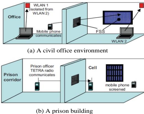
Figure 2-1: Example of finite FSS panel usage in different scenarios. In both cases it is assumed that the surrounding walls, floors, and ceilings are screened with thermally insulating metal sheeting (Q. Nidal, et al. [22], @ Loughborough University, 2012) and (J. Batchelor, et al. [23], @ Loughborough University, 2009).
