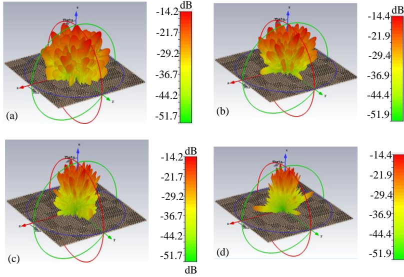
Figure 6-14: 3-D RCS pattern of the proposed metasurface under normal incidence at (a) 7 GHz, (b) 9.2 GHz, (c) 14 GHz, and (d) 19.6 GHz, (M. Akbari et al. [136], @2019 IEEE).
