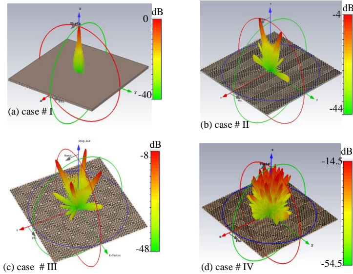
Figure 6-15: 3-D simulation patterns of periodic coding metasurfaces to indicate their ability to control scattering patterns using various coding sequences under the normal incidence of EM waves at the centre frequency 14 GHz. (a) case #I (000000.../000000...), (b) case #II (010101.../010101...), (c) case #III (010101.../101010...), and (d) case #IV (the proposed metasurface) , (M. Akbari et al. [136], @2019 IEEE).
