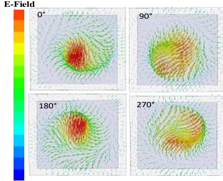
Figure 3-10: RHCP E-field variations at different phases (a) 0°, (b) 90°, (c) 180°, and (d) 270 °at the centre frequency 30 GHz, (M. Akbari et al. [31], @2016 IEEE).
