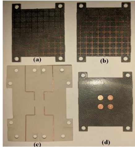
Figure 4-15: Photos of the fabricated 2×2 MIMO-ACMA: (a) and (b) FSS layers, (c) feedlines, and (d) patches, (M. Akbari et al. [49], @2017 IEEE).
