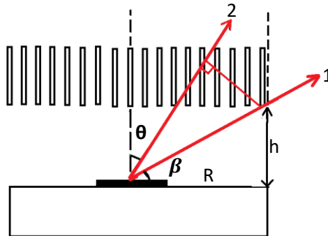
Figure 5-8: Model of the diffraction and transmission rays [31]., (M. Akbari et al. [93], @2017 IEEE).
