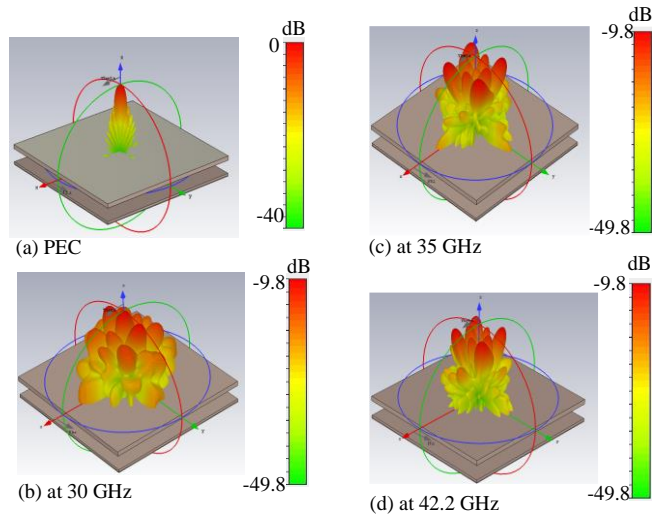
Figure 6-37: The 3-D RCS pattern of the FPC antenna terminated with the matching load under normal incidence for (a) particular case of the mettalic plate, the proposed metasurface at (b) 30 GHz, (c) 35 GHz, and (d) 42.2 GHz. (the plots are normalized with a metallic plate), (S. Zarbakhsh, M. Akbari et al. [32], @2019 IEEE).
