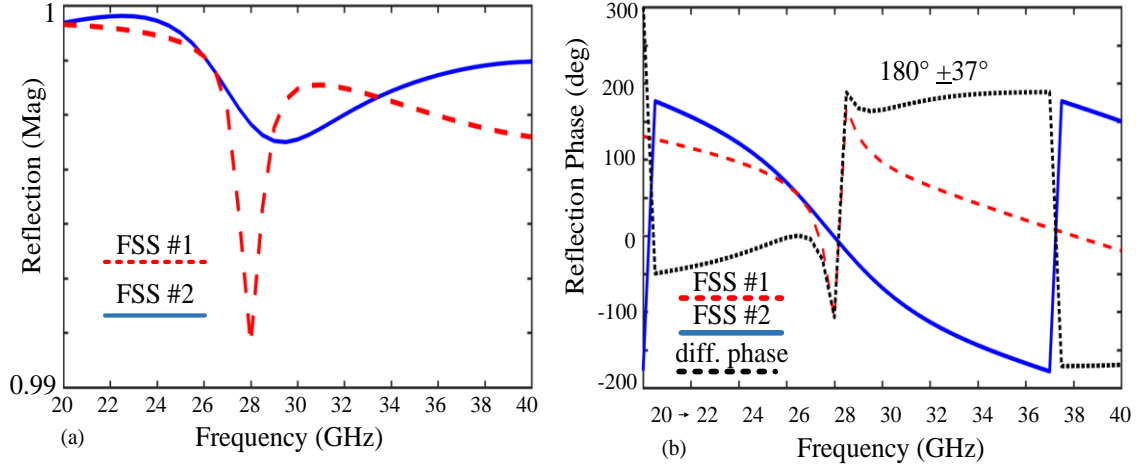
Figure 6-27: The reflection coefficients of FSS units (a) magnitude and (b) phase, (S. Zarbakhsh, M. Akbari et al. [32], @2019 IEEE).
