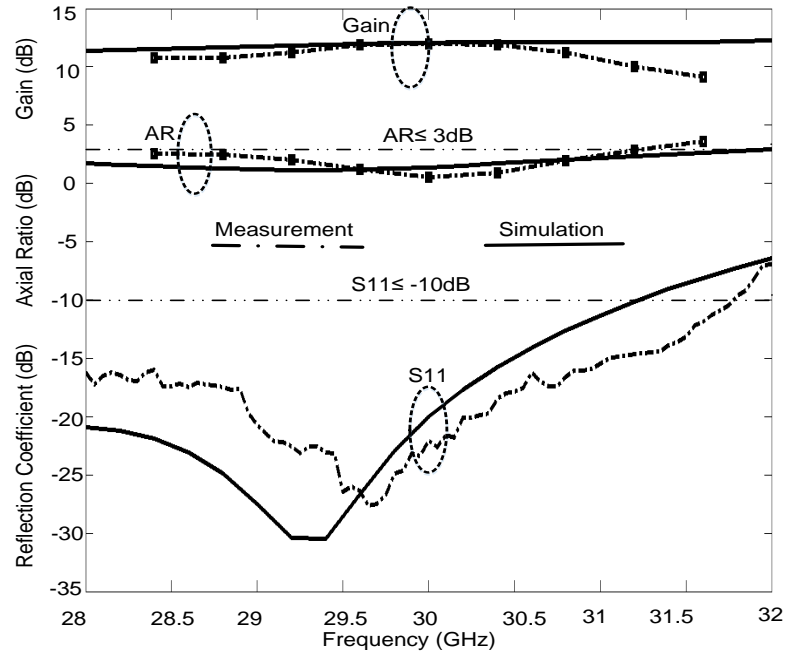
Figure 5-21: The measured and simulated curves of total gain, axial ratio, and reflection coefficient of the proposed design; including the LP antenna array with the polarizer, (M. Akbari et al. [93], @2017 IEEE).
