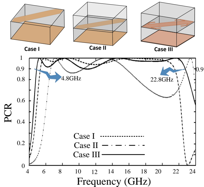
Figure 6-7: The PCR results for the different FSS cells with respect to the design procedure, (M. Akbari et al. [136], @2019 IEEE).
