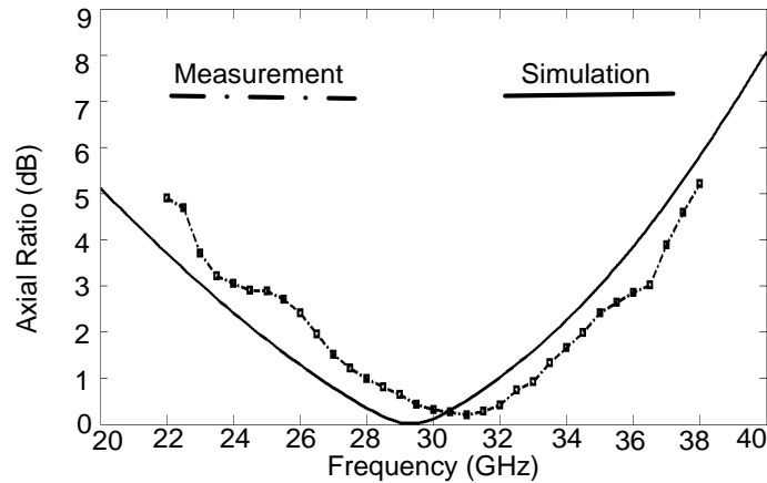
Figure 5-12: The measured and simulated axial ratio of the polarizer with the wideband horn antenna, (M. Akbari et al. [93], @2017 IEEE).
