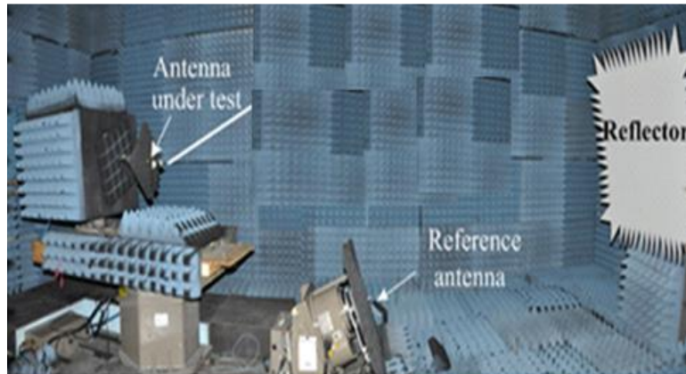
Figure 4-25: Radiation pattern measurement setup with receiving mode of the antenna under test, (M. Farahani et al. [51], @2017 IEEE).
