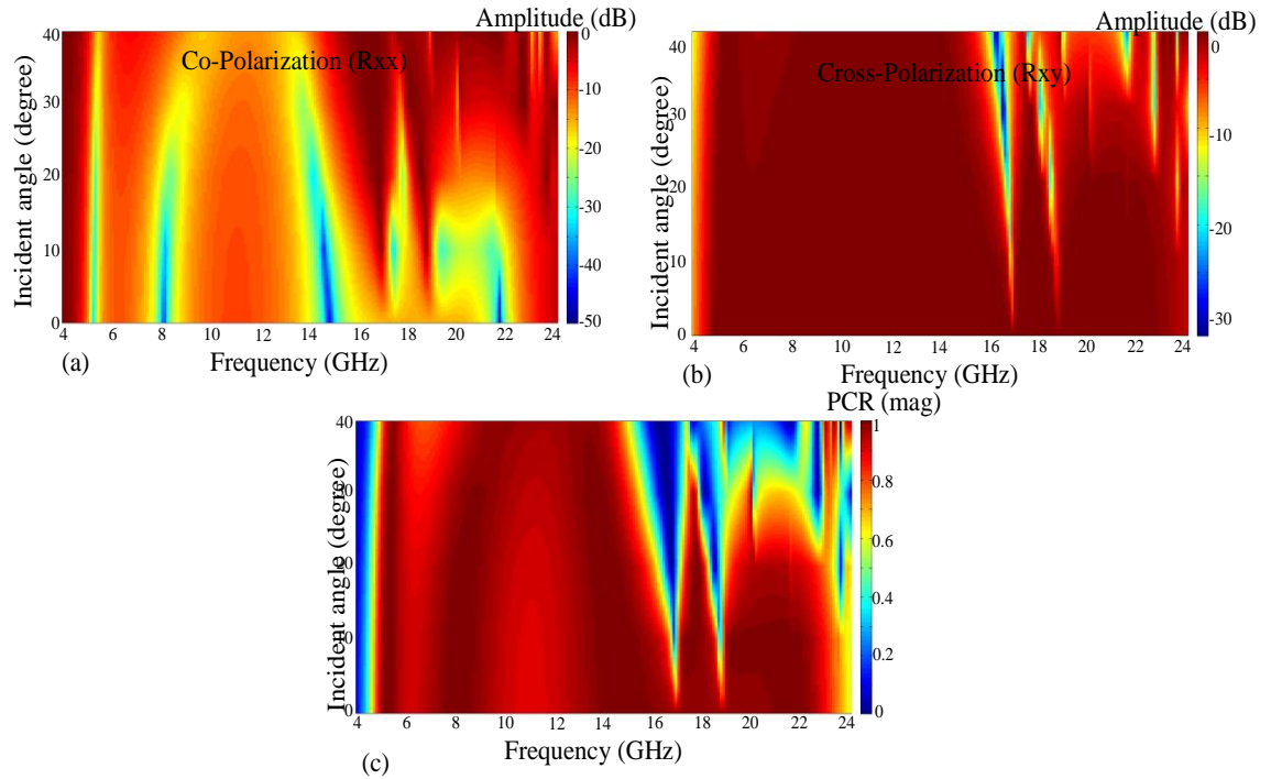
Figure 6-6: Simulated results of reflective parameters of FSS with different incident angles versus frequency band. (a) The amplitude of reflective coefficients with co-polarization, (b) amplitude of reflective coefficients with cross-polarization, (c) PCR of reflective coefficients, (M. Akbari et al. [136], @2019 IEEE).
