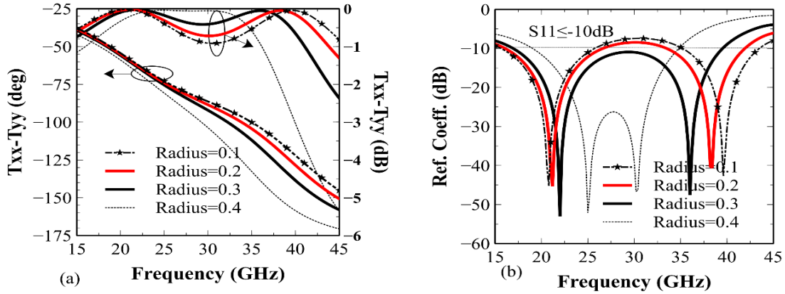
Figure 5-5: (a) variations of transmission coefficients and (b) reflection coefficients in the unit cell model when the radius of the circle conductor changes, (M. Akbari et al. [93], @2017 IEEE).
