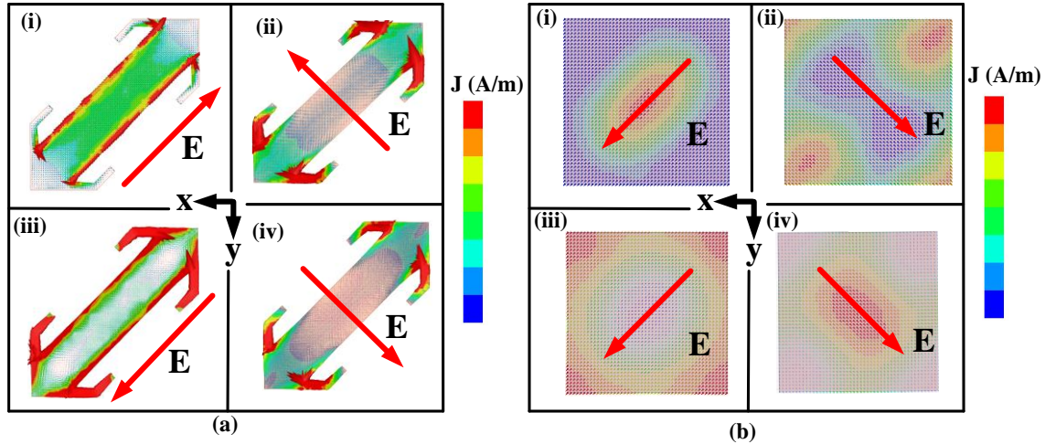
Figure 6-3: The surface current distributions induced on (a) FSS and (b) ground plate for resonance (i) to resonance (iv), (M. Akbari et al. [136], ©2019 IEEE).
