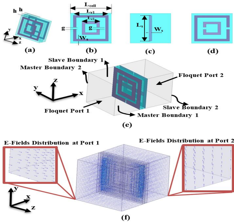
Figure 4-19: (a) Perspective view of the unit cell. (b) Metallic SRR-like on the top surface. (c) Metallic strip on the middle surface. (d) Metallic SRR-like on the bottom surface. (e) Specific boundary conditions defined Floquet port excitation to extract scattering parameters. (f) E-fields distribution at 60 GHz. The dimensions are L_{cell} = 2 , L_{r1} = 1.6 , L_{r2} = 1 , g = 0.05 , W_s = 0.2 , h = 0.127 , and all in millimetre, (M. Farahani et al. [51], ©2017 IEEE).
