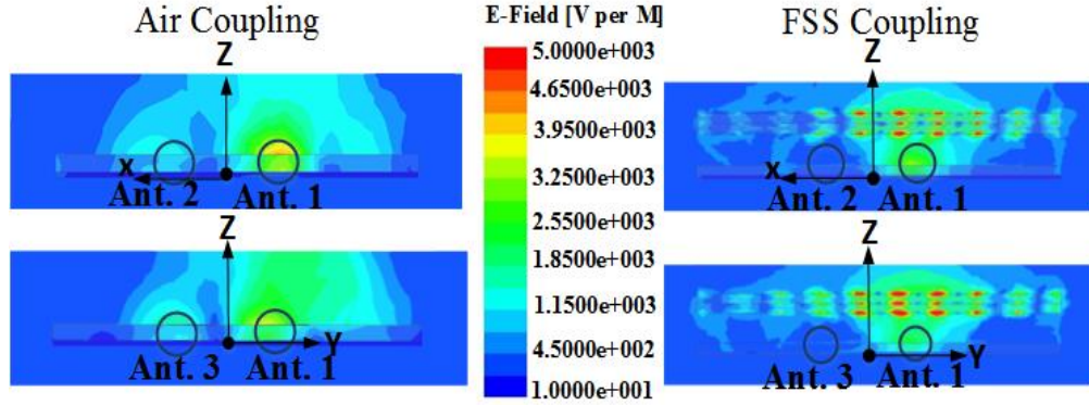
Figure 4-14: Simulated E-Field distribution on the 2×2 MIMO-ACMA for both cases air and FSS couplings in the xz- and yz- planes at frequency 31.2GHz, (M. Akbari et al. [49], @2017 IEEE).
