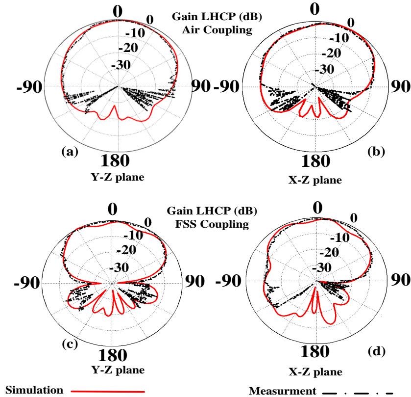
Figure 4-18: Measured and simulated LHCP gain for both cases of (a), (b) air coupling and (c), (d) FSS coupling in the yz- and xz- planes at frequency 31GHz, (M. Akbari et al. [49], @2017 IEEE).
