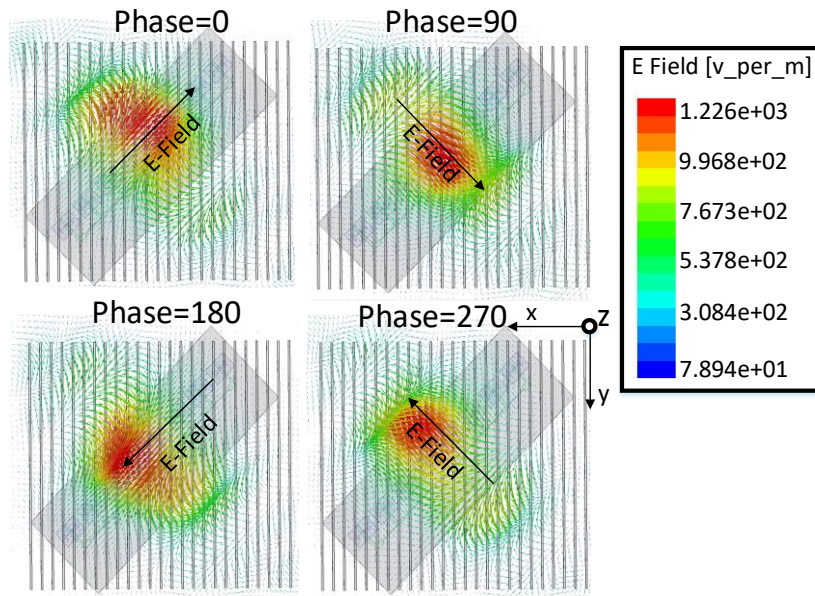
Figure 5-23: (a) RHCP for E-field variations at different phases (a)0°, (b)90°, (c)180°, and (d)270 ° at the centre frequency 30 GHz, (M. Akbari et al. [93], @2017 IEEE).
