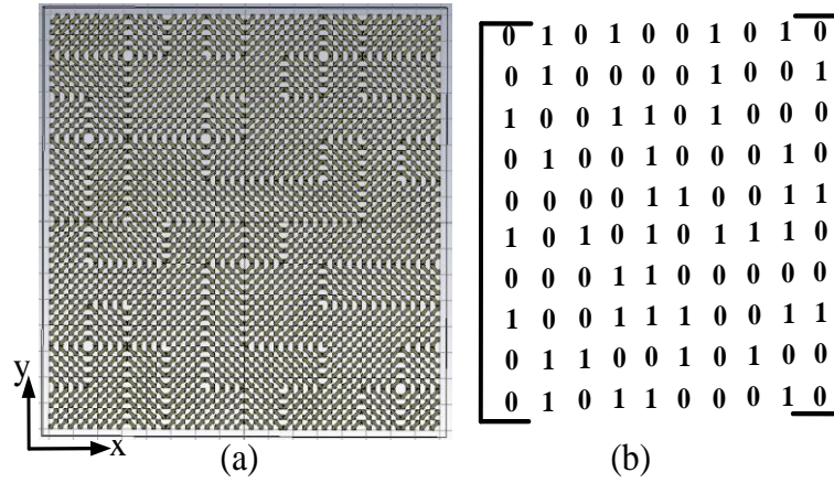
Figure 6-10: Proposed metasurface and associated coding matrix with ratio 0.4, (M. Akbari et al. [136], @2019 IEEE).
