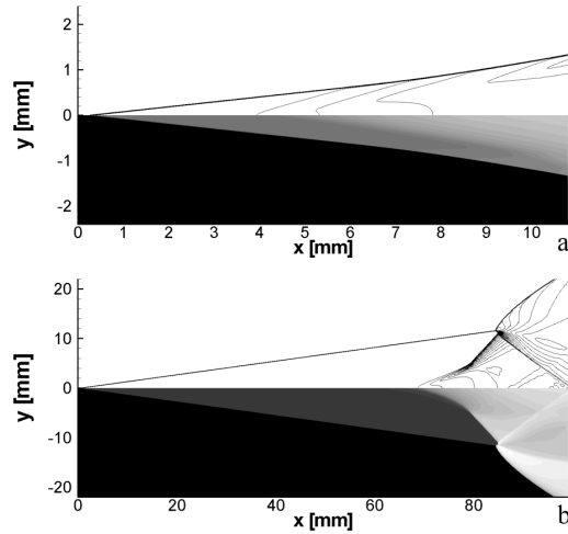
Fig. 6. Pressure (upper) and temperature (lower) fields with P_0 = 0.2 atm and M_0 = a) 10.0 and b) 7.0.
