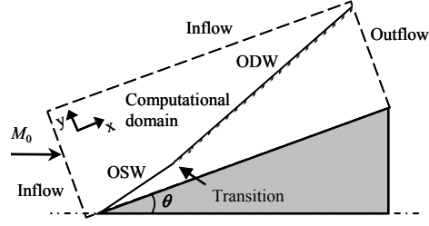
Fig. 1. Schematic of a typical ODW.
