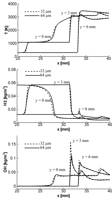
Fig. 3. Temperature and species profiles along different y -line locations from the resolution study for P_0 = 0.5 atm and M_0 = 7.0 .
