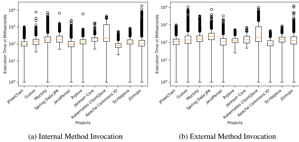
Figure 6.3: Execution Time for Internal and External Method Invocation
