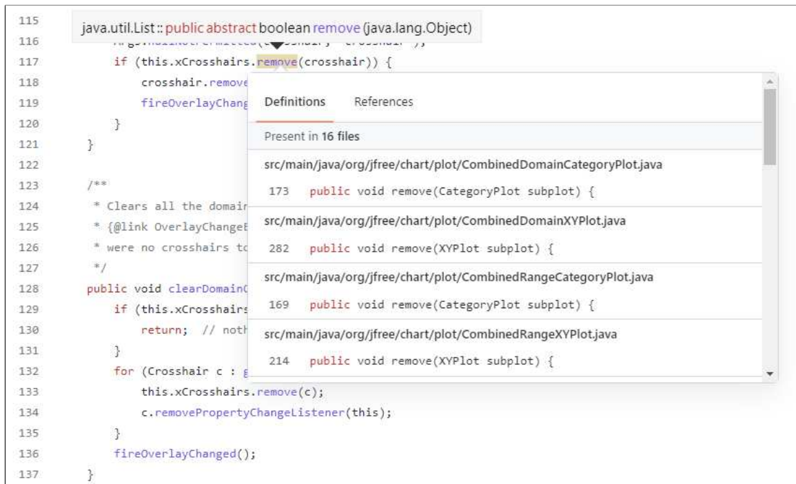
Figure 5.3: No Consideration of Invocation Context (Collected from JFreeChart 3 )
