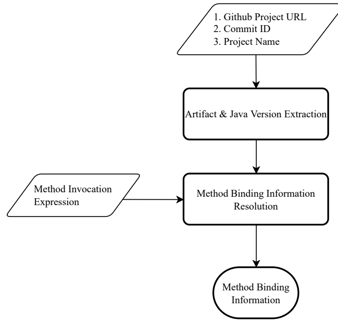
Figure 4.1: Overview of our approach
