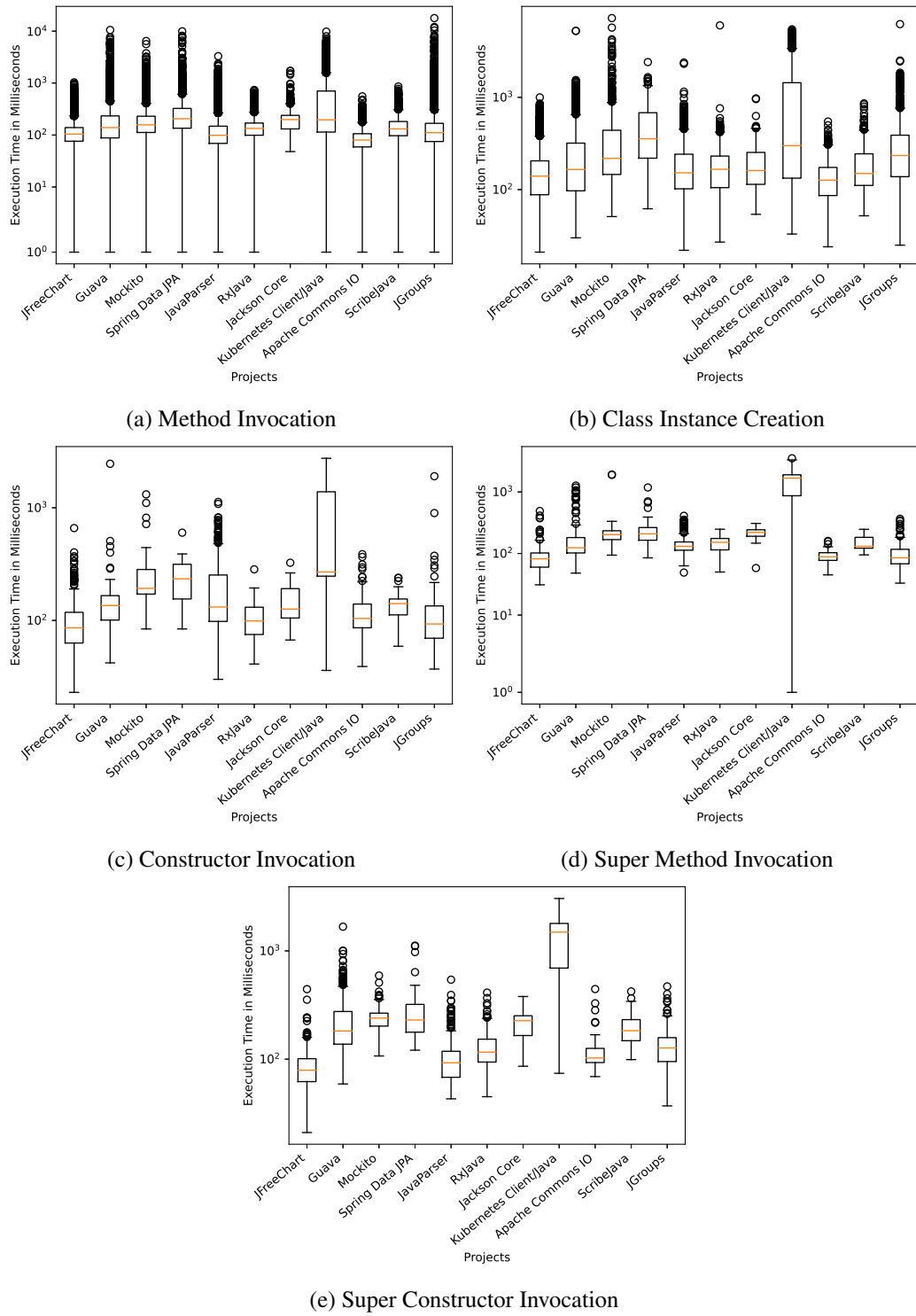
Figure 6.4: Execution Time for Method Invocation Expressions
