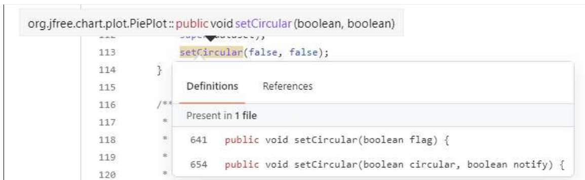
Figure 5.4: No Consideration of Number of Method Arguments (Collected from JFreeChart 4 )
